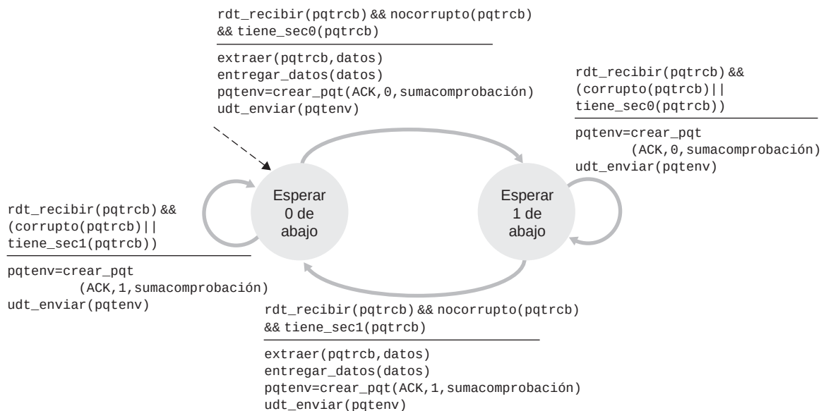
Figura 3.14 ♦ Lado receptor de rdt2.2
