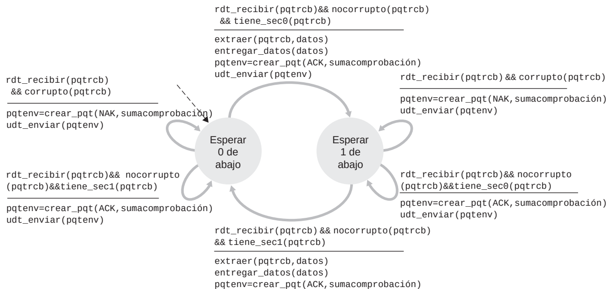
Figura 3.12 ♦ Lado receptor de rdt2.1
