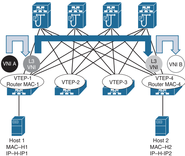
Figure 13-8 Symmetric IRB Flow
