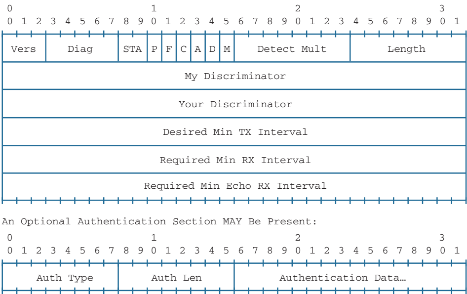
Figure 14-5 BFD Control Plane Format
