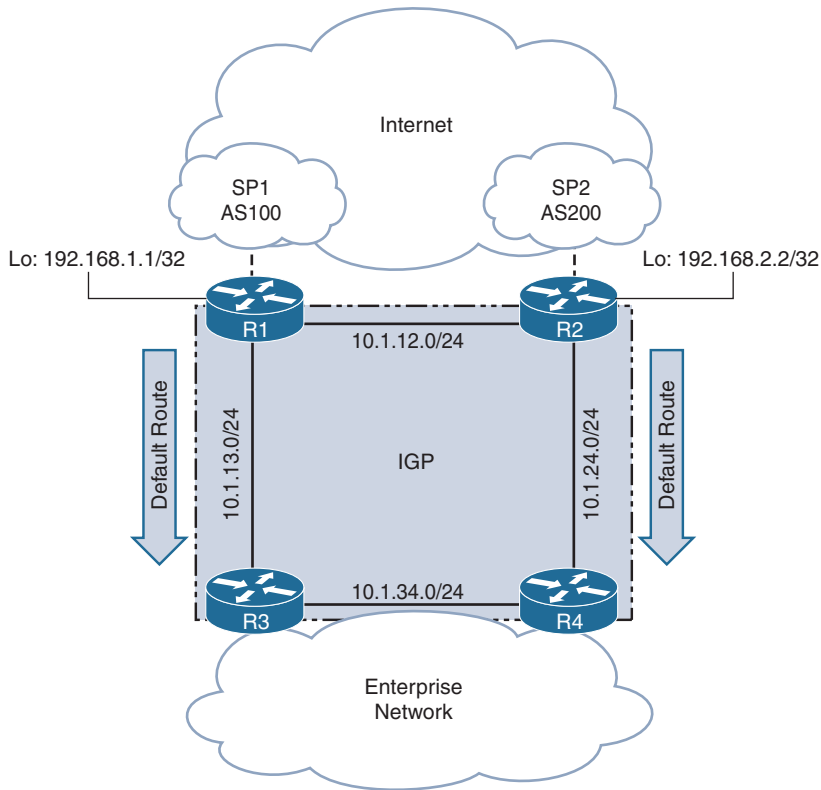
Figure 8-13 Common BGP Multihomed Topology
