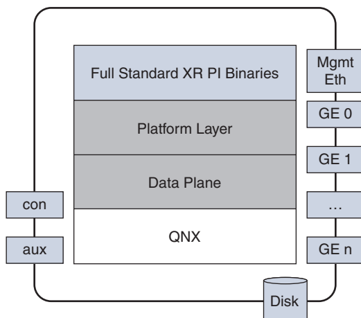
Figure 7-22 IOS XRv Architecture
