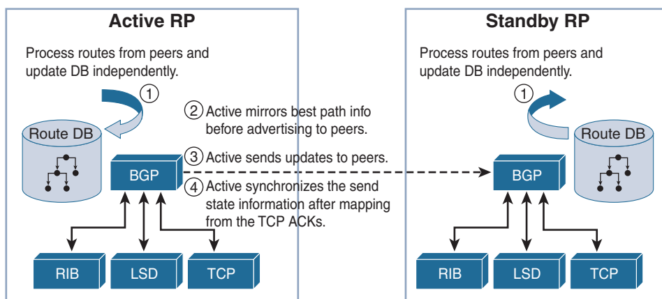
Figure 14-2 BGP NSR Architecture on Cisco IOS
