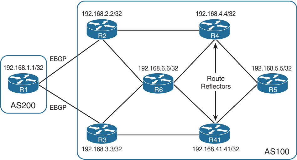
Figure 7-25 RR Topology with Multiple IGP Paths of Different Metric
