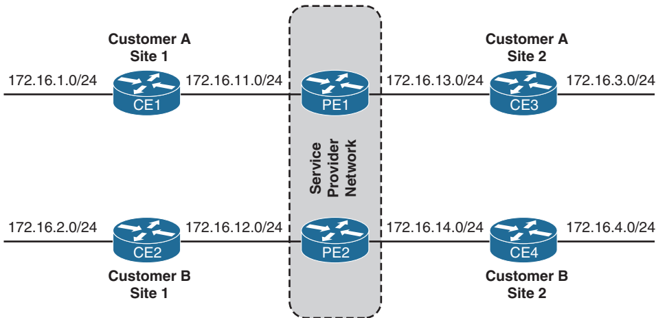
Figure 10-2 Separate Routing Domains
