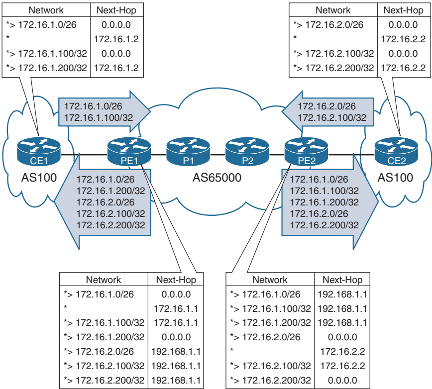
Figure 10-7 Problems with CE Route Tables if CEs Use the Same ASN
