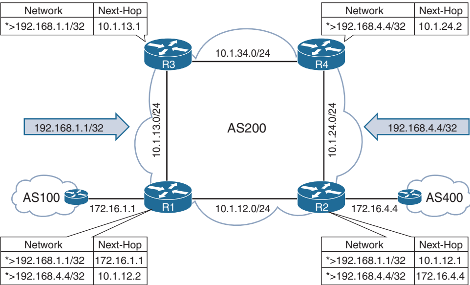
Figure 8-14 Common BGP Multihomed Topology
