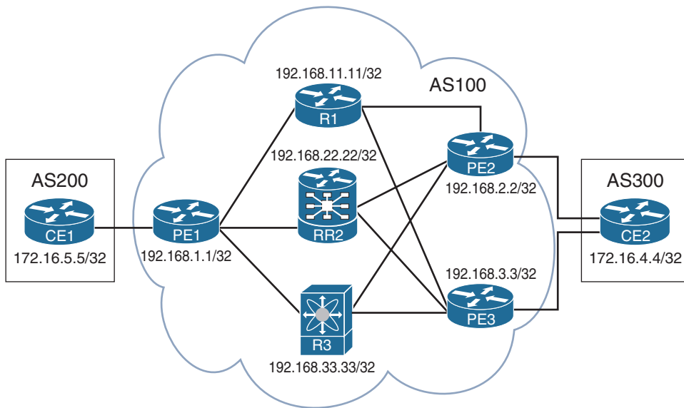
Figure 14-8 Topology with Route Reflector
