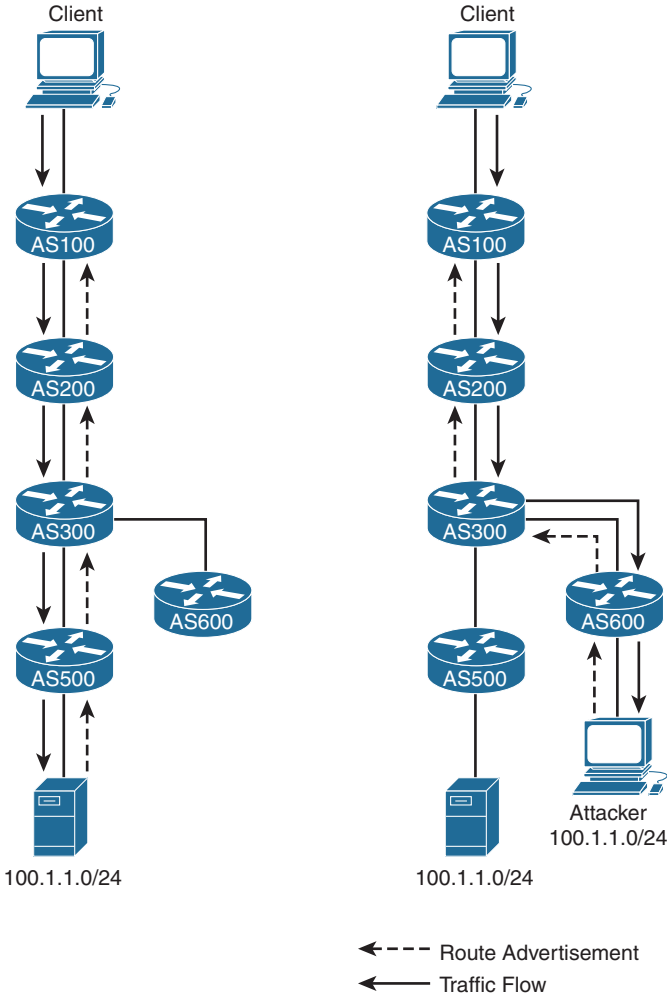
Figure 9-4 Prefix Hijacking—More Specific Prefix
