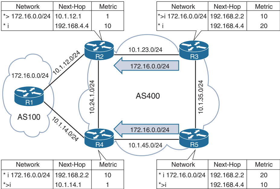
Figure 8-7 Lowest IGP Metric Topology
