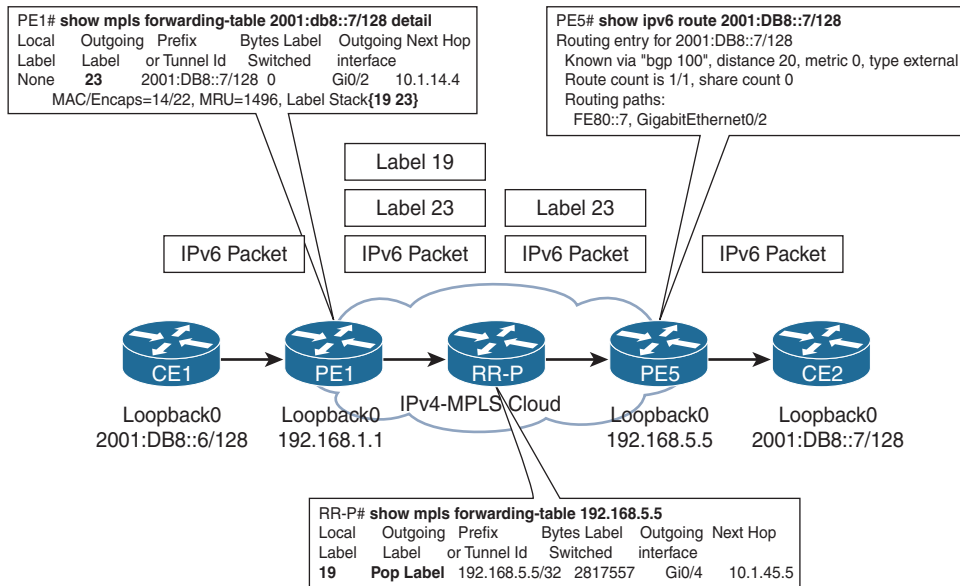
Figure 12-6 6PE Data Plane Flow
