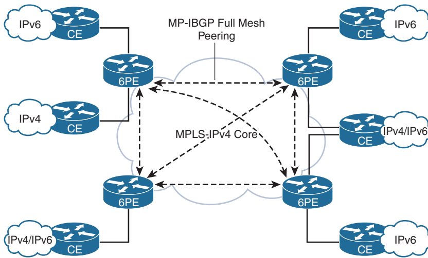
Figure 12-4 6PE Architecture
