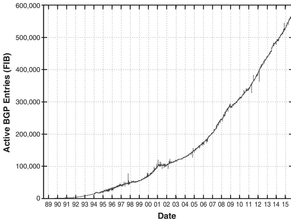
Figure 7-1 IPv4 Internet Routing Table Growth from 1989–2015
