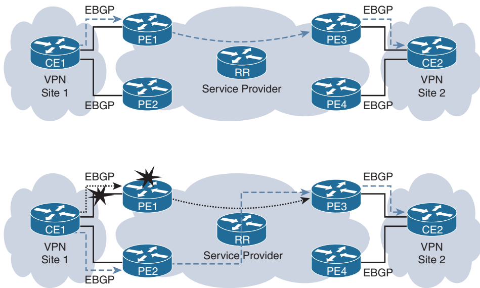
Figure 14-15 BGP PIC for PE-CE Link/Node Protection on CE Side
