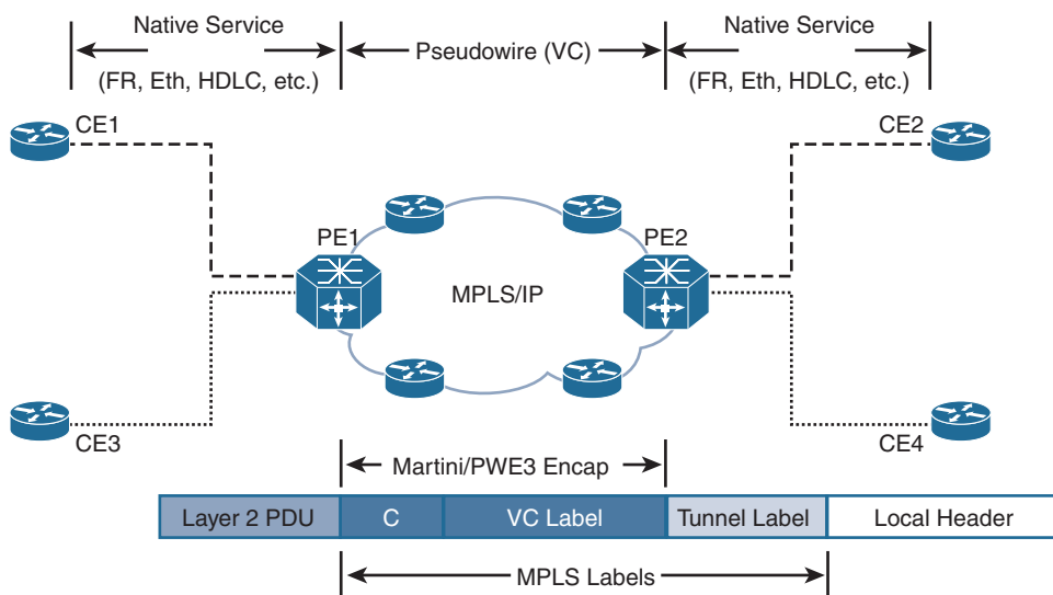
Figure 11-4 VPWS Data Plane
