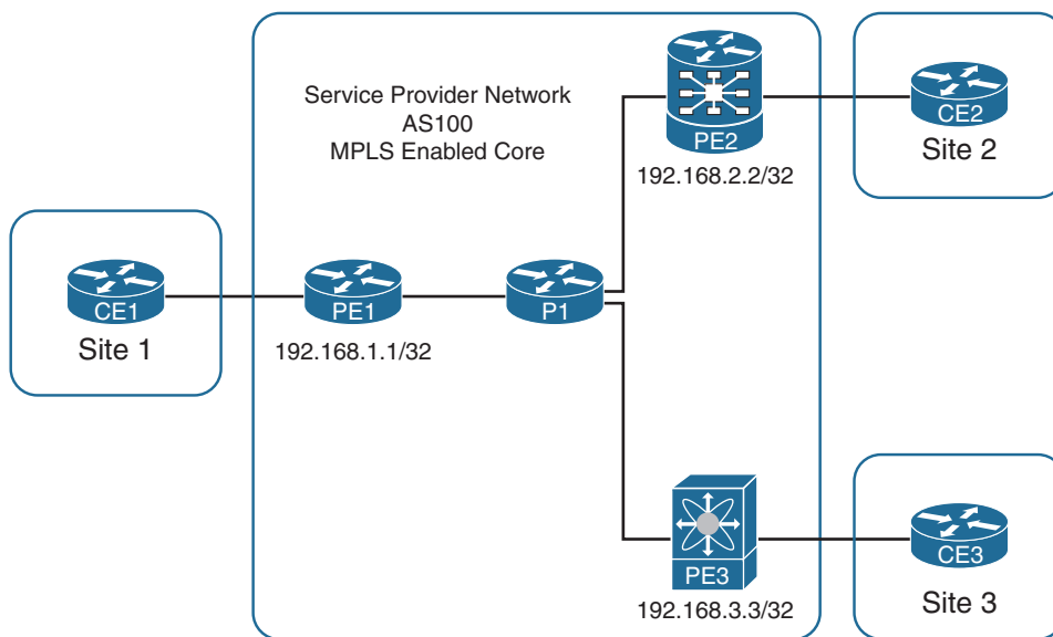
Figure 11-5 Topology
