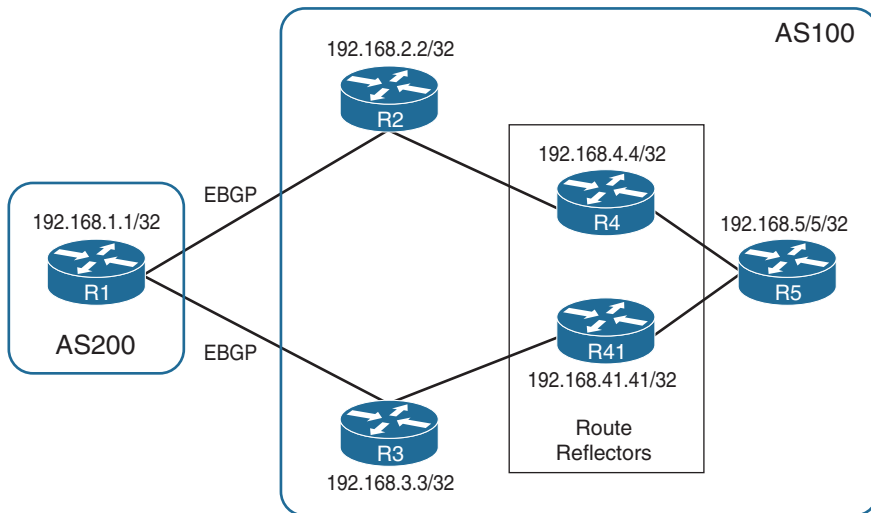
Figure 7-23 RR Topology with Multiple IGP Paths
