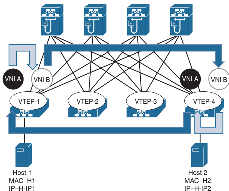
Figure 13-7 Asymmetric IRB Flow
