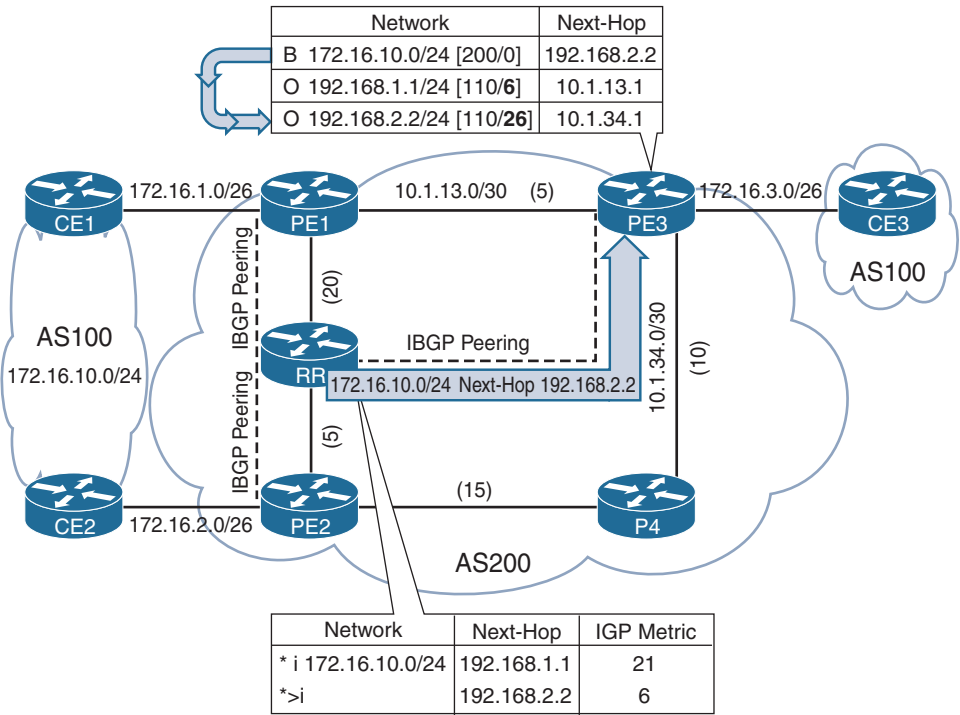
Figure 10-8 VPNv4 Suboptimal Routing with Route Reflectors
