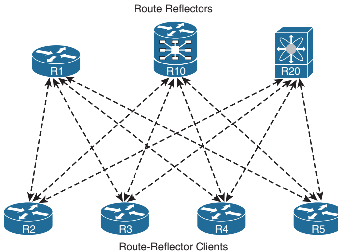
Figure 5-3 Topology with Route Reflectors
