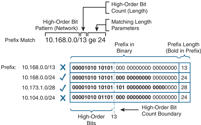
Figure 4-10 Prefix Match Pattern with Matching Length Parameters
