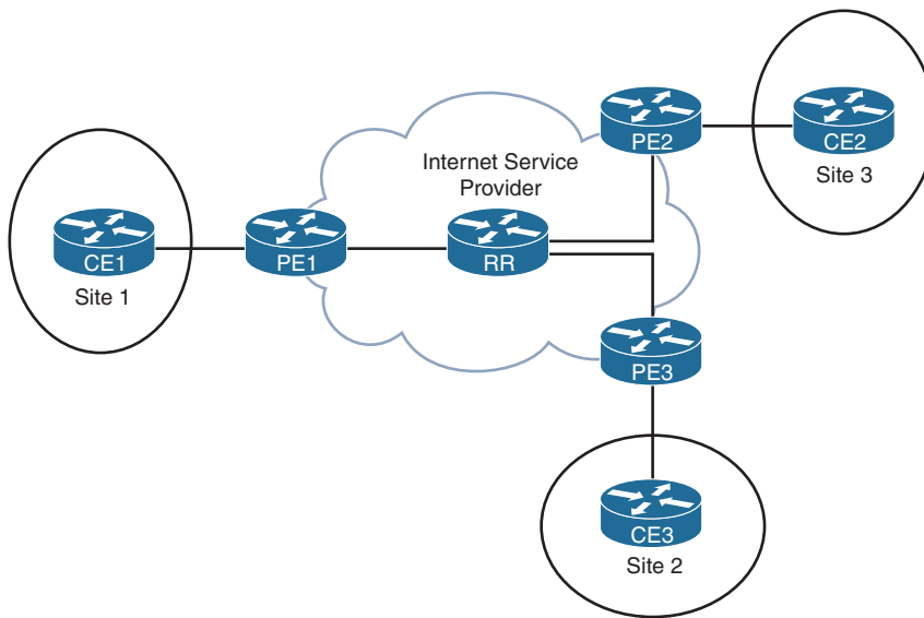
Figure 9-2 Typical Internet Deployment Topology
