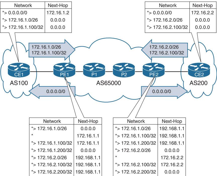
Figure 10-6 CE Routers Receiving Only a Default Route
