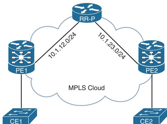
Figure 15-10 PBB-EVPN Topology
