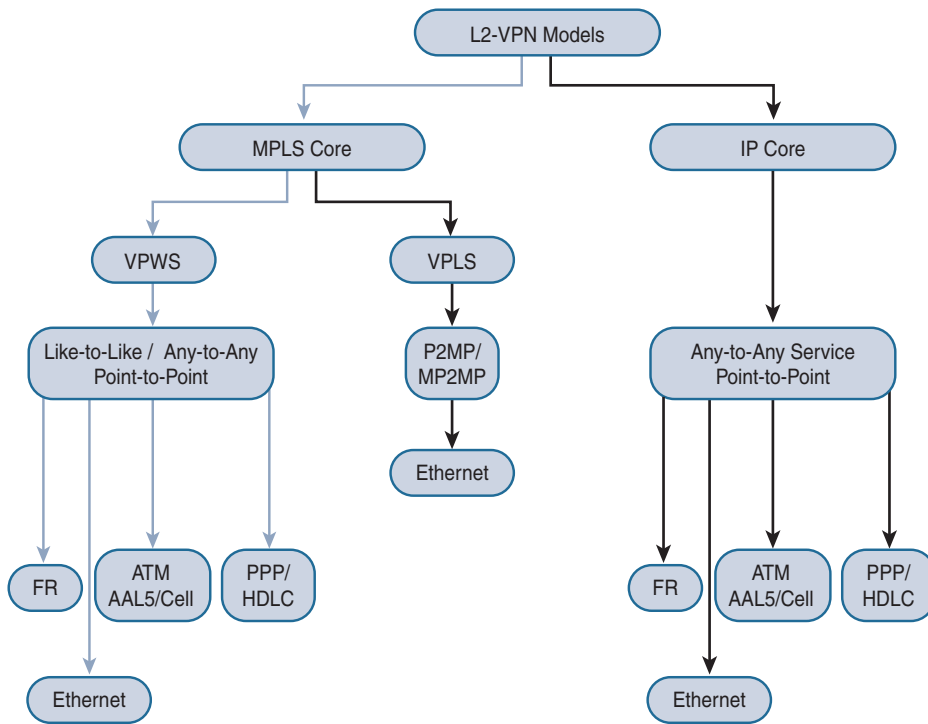
Figure 11-1 L2VPN Models
