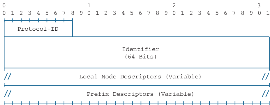
Figure 15-5 Type 3 and Type 4—Prefix NLRI
