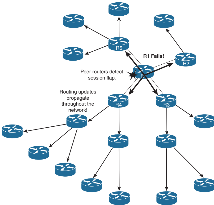
Figure 14-1 Impact of Node Failure in a Network with BGP Route Reflectors
