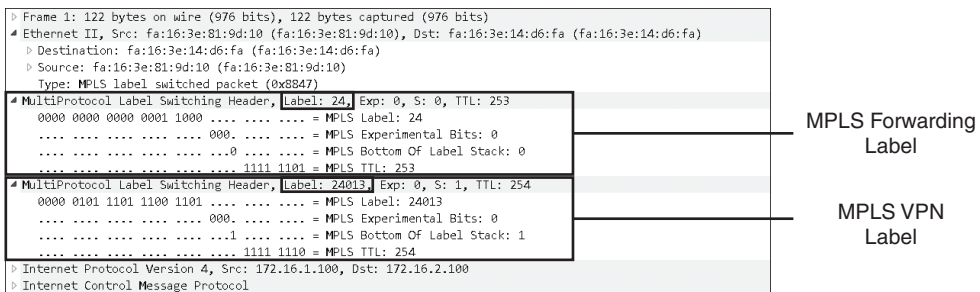
Figure 10-13 Packet Capture of MPLS L3VPN Packet
