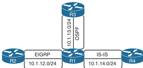
Figure 4-1 Route Redistribution Topology
