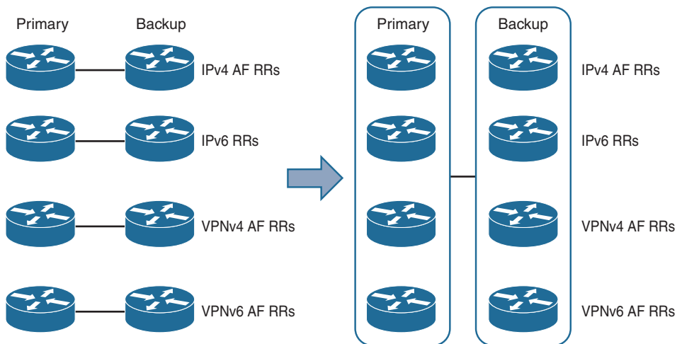
Figure 7-20 vRR Routing Design
