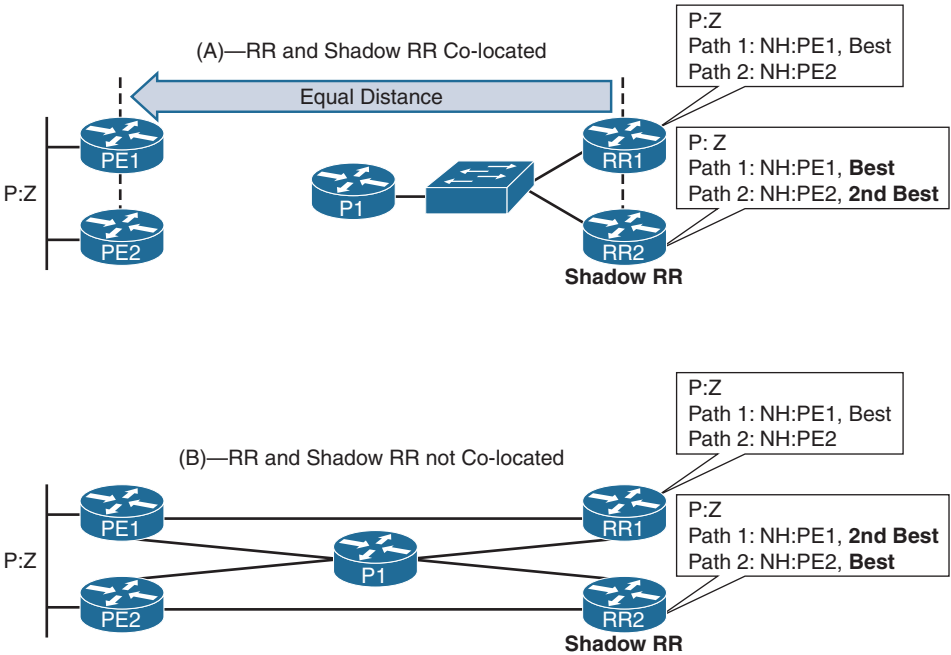
Figure 7-24 Shadow Routers Design Scenarios
