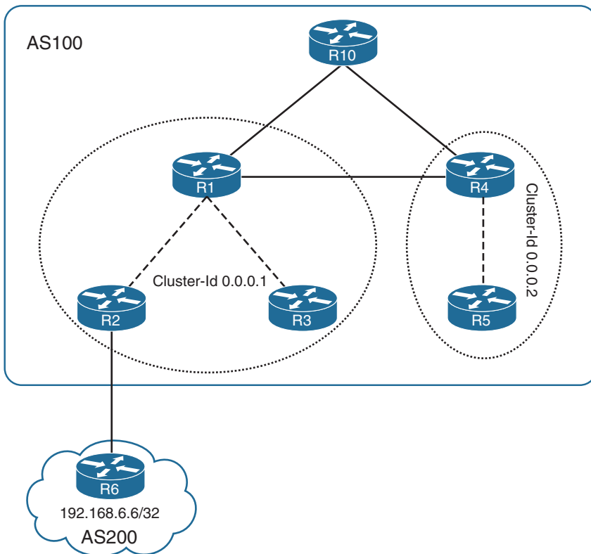
Figure 7-16 BGP Cluster Topology
