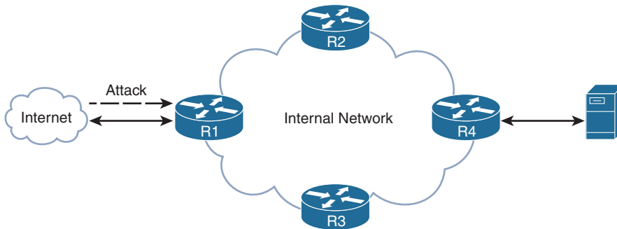
Figure 9-15 DDOS Attack Mitigation with RTBH
