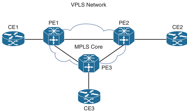
Figure 11-9 Virtual Private LAN Services
