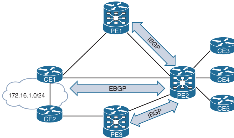
Figure 8-3 EIBGP Multipath with MPLS L3VPN Topology
