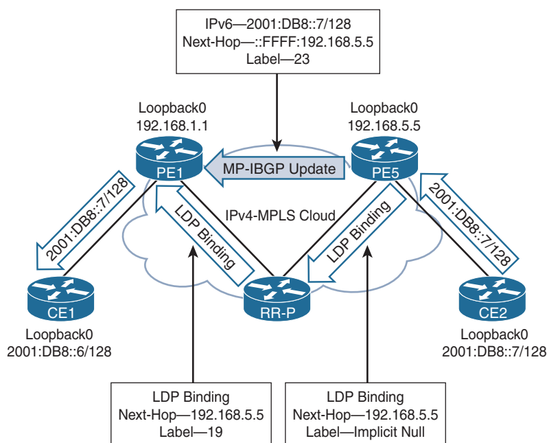
Figure 12-5 6PE Control-Plane Flow
