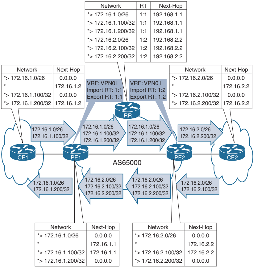
Figure 10-9 Different Import and Export Route Targets
