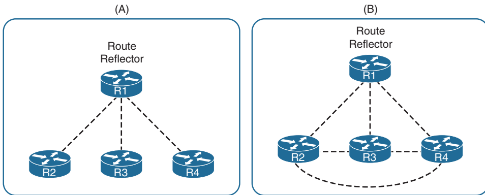
Figure 7-15 Topology with RR and RR Clients and Topology with RR with Full-Mesh RR Clients
