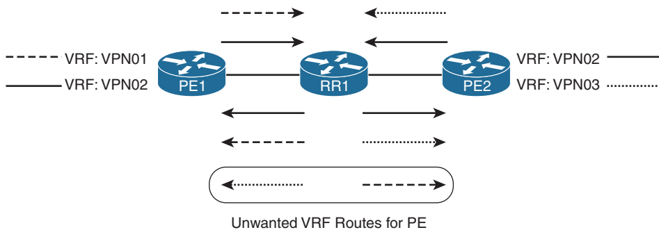
Figure 10-11 Unnecessary VPN Prefixes Advertised to PE Routers
