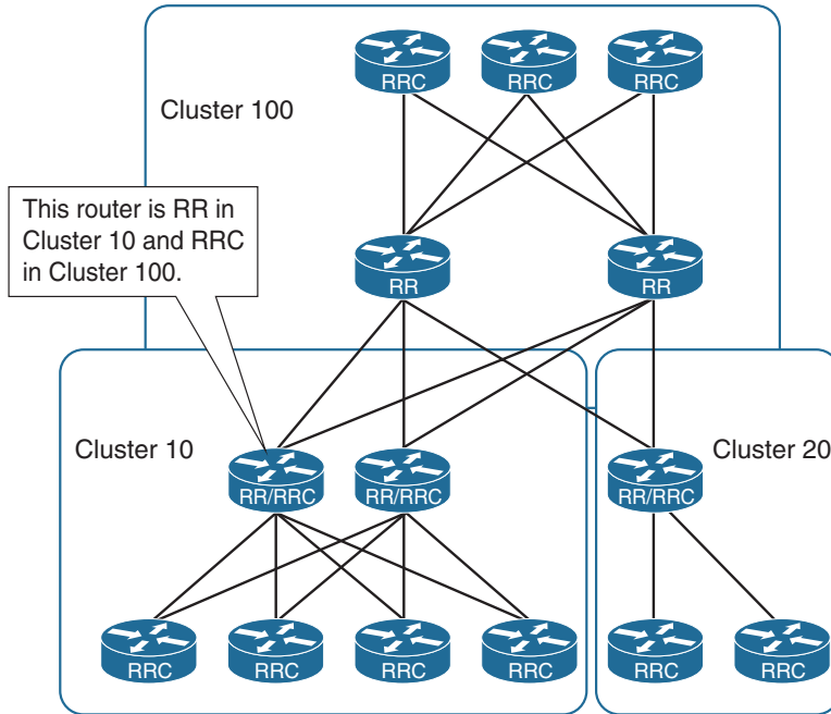
Figure 7-17 Hierarchical Route Reflector
