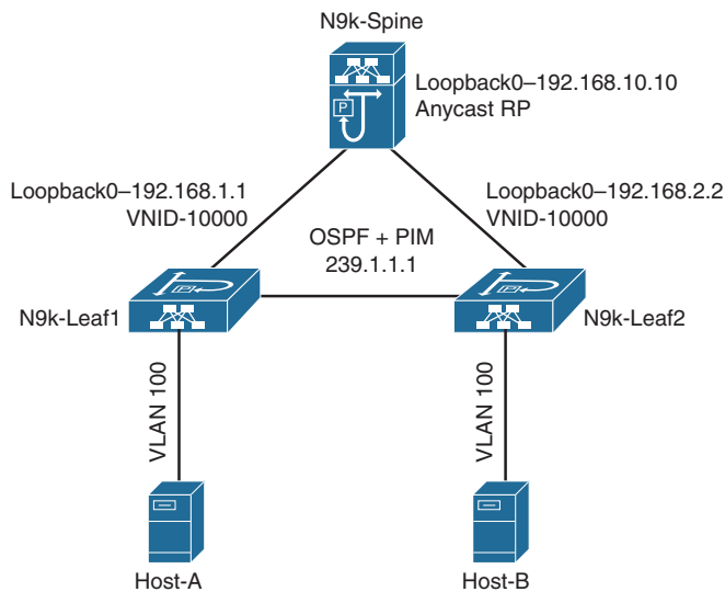
Figure 13-5 VxLAN Flood-and-Learn Topology
