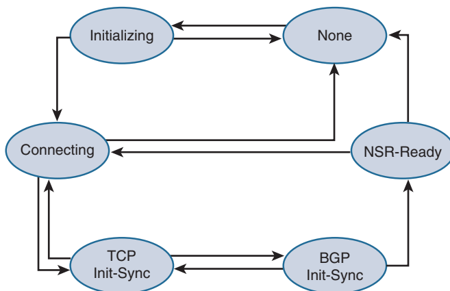
Figure 14-3 BGP NSR Finite State Machine
