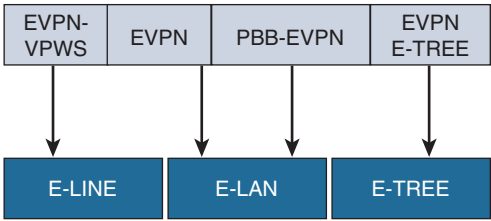
Figure 15-9 EVPN Solution Architecture
