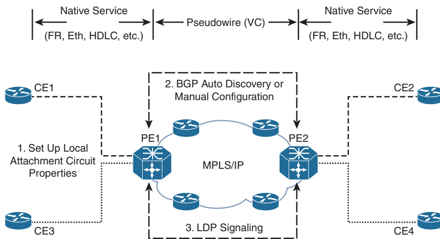
Figure 11-3 VPWS Control Plane
