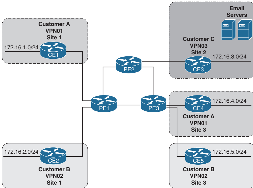
Figure 10-10 VRF Services Topology
