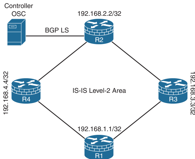
Figure 15-6 Topology
