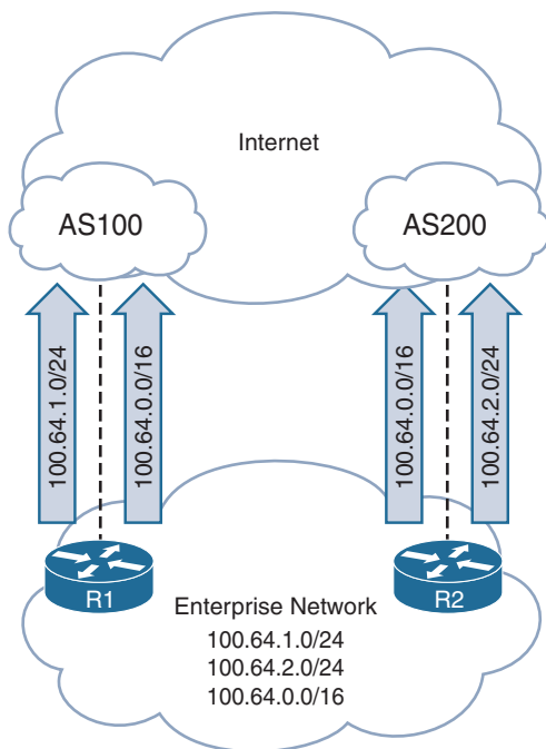
Figure 8-4 BGP Path Selection Using Longest Match
