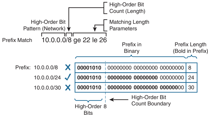
Figure 4-11 Prefix Match with Ineligible Matched Prefixes
