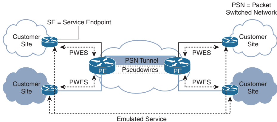
Figure 11-2 Pseudowires over Packet Switched Network
