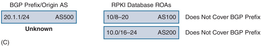
Figure 9-13 Unknown Prefix Based on ROA Entries
