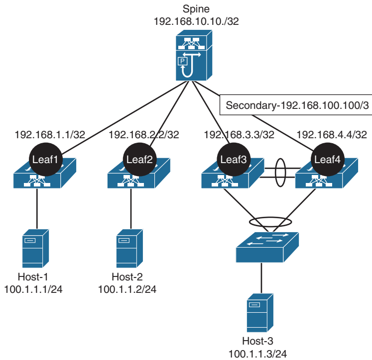
Figure 13-12 VxLAN BGP EVPN Topology
