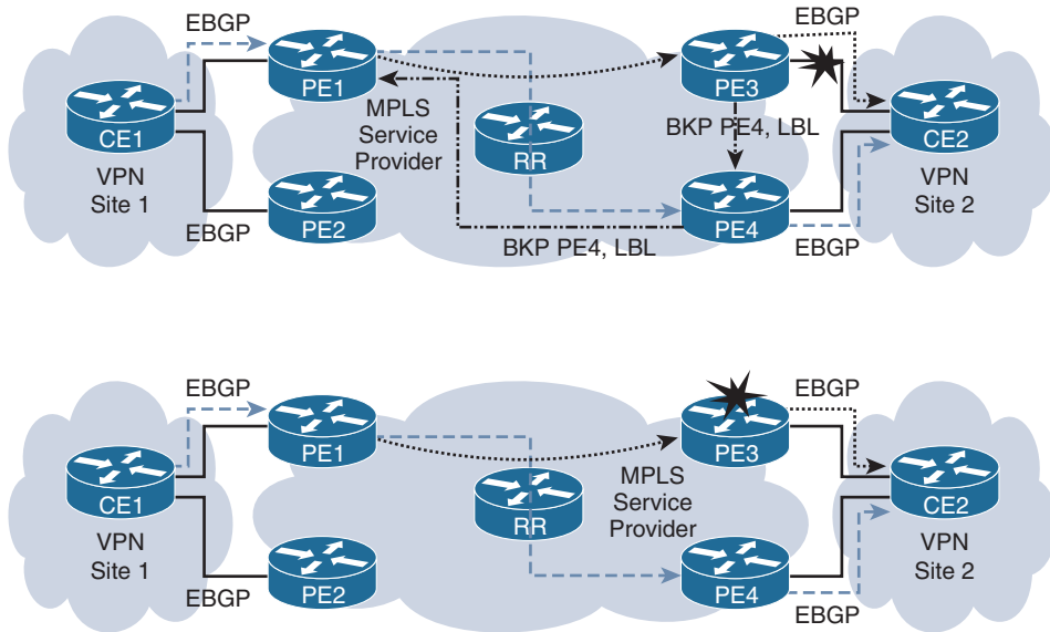
Figure 14-16 BGP PIC with PE-CE Link Protection in MPLS VPN Network
