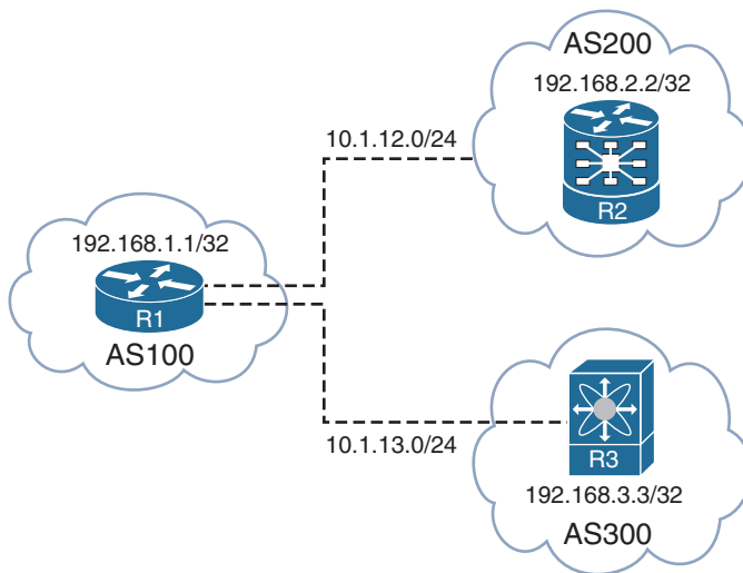
Figure 14-7 EBGP Peering with BFD
