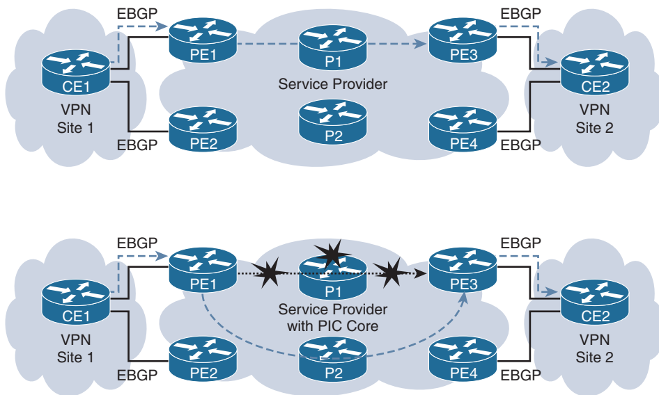
Figure 14-11 BGP PIC Core
