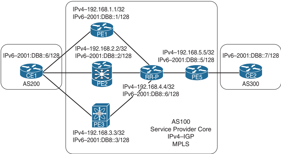
Figure 12-1 IPv6 Topology
