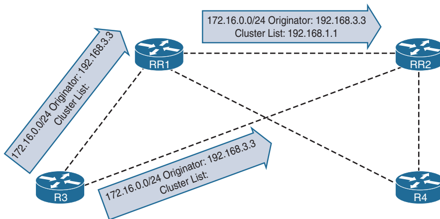
Figure 8-8 Minimum Cluster List Length
