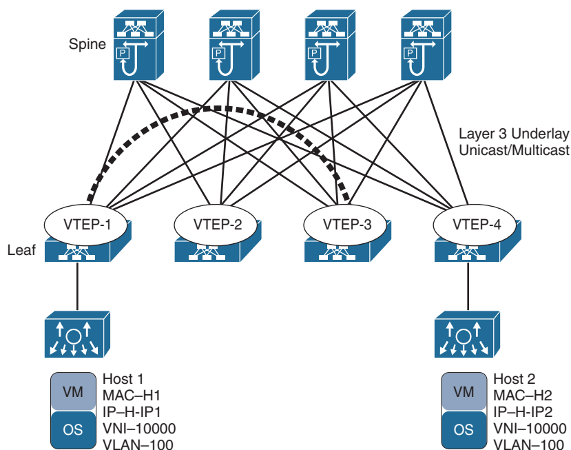
Figure 13-3 Data Center with VxLAN Overlay
