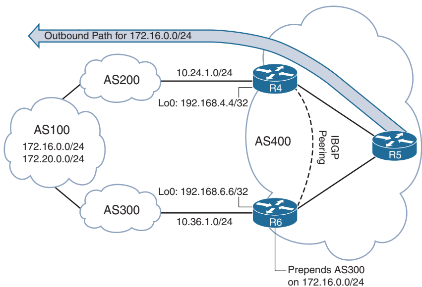
Figure 8-10 Modifying BGP AS-Path
