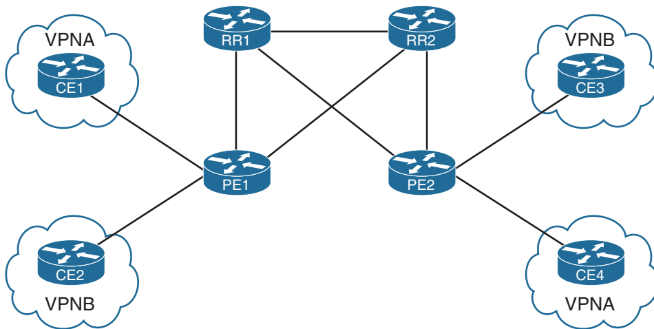
Figure 7-18 Partitioned RR Topology
