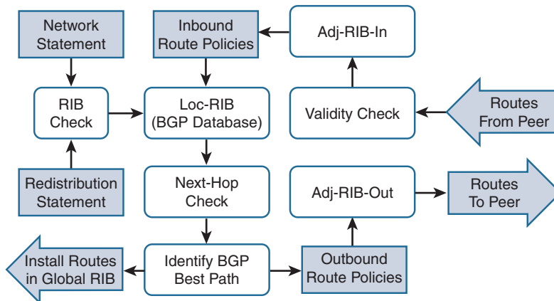
Figure 4-3 Complete BGP Network Advertisement
