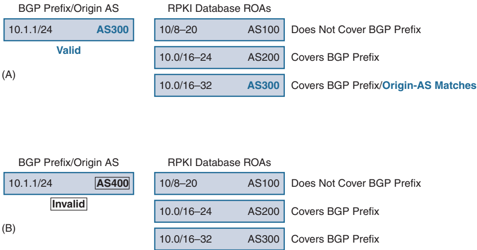
Figure 9-12 Valid Prefix Based on ROA Entries
