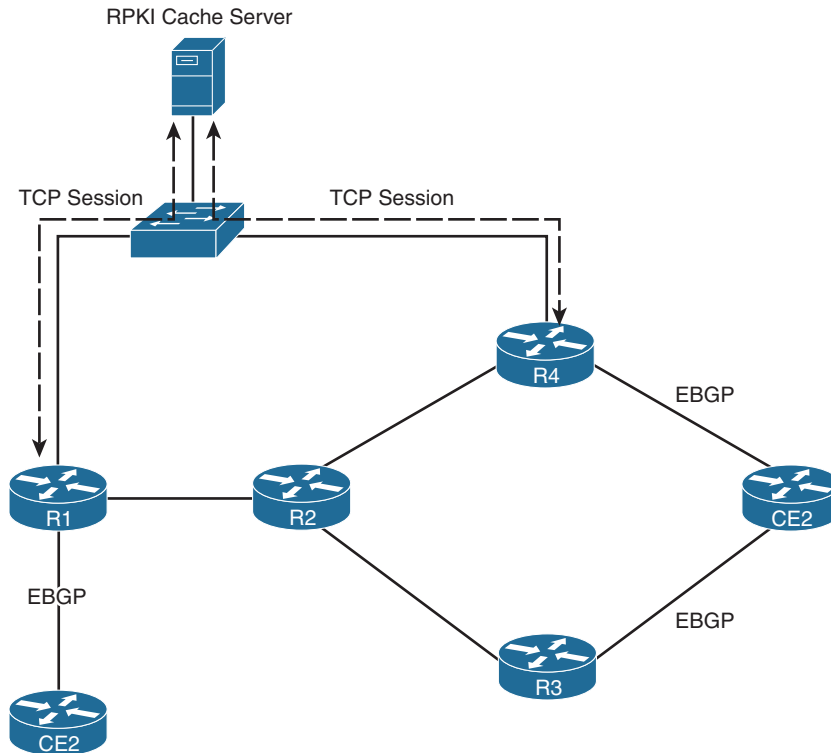
Figure 9-14 Topology with RPKI Cache Server
