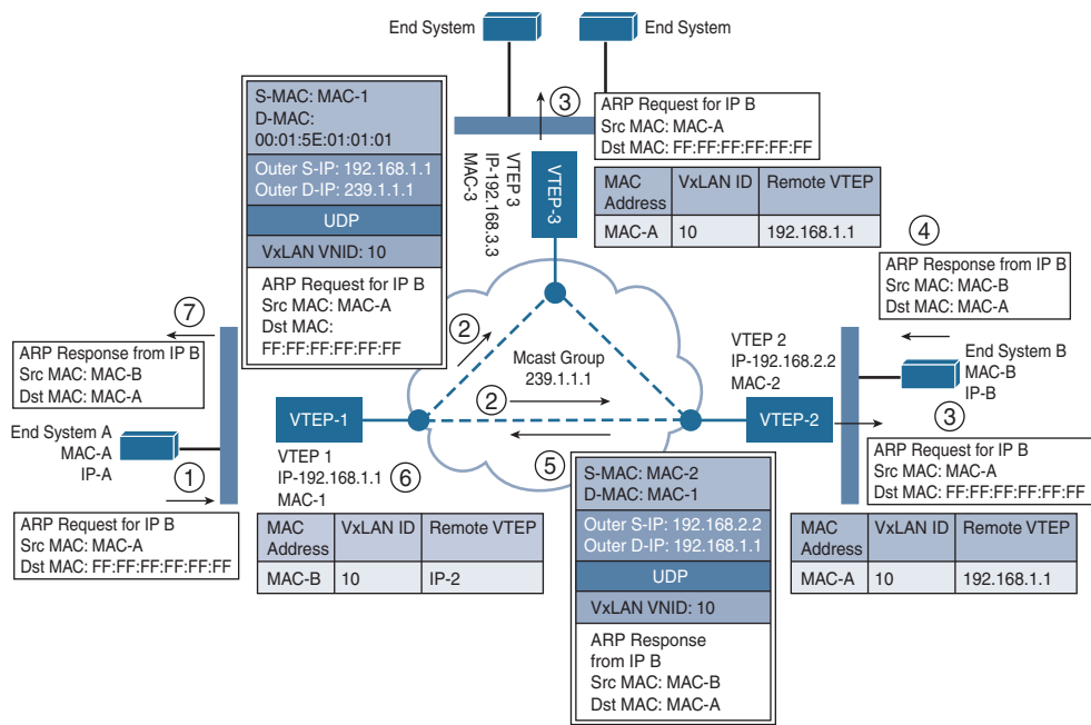
Figure 13-4 VxLAN Flood-and-Learn Packet Flow
