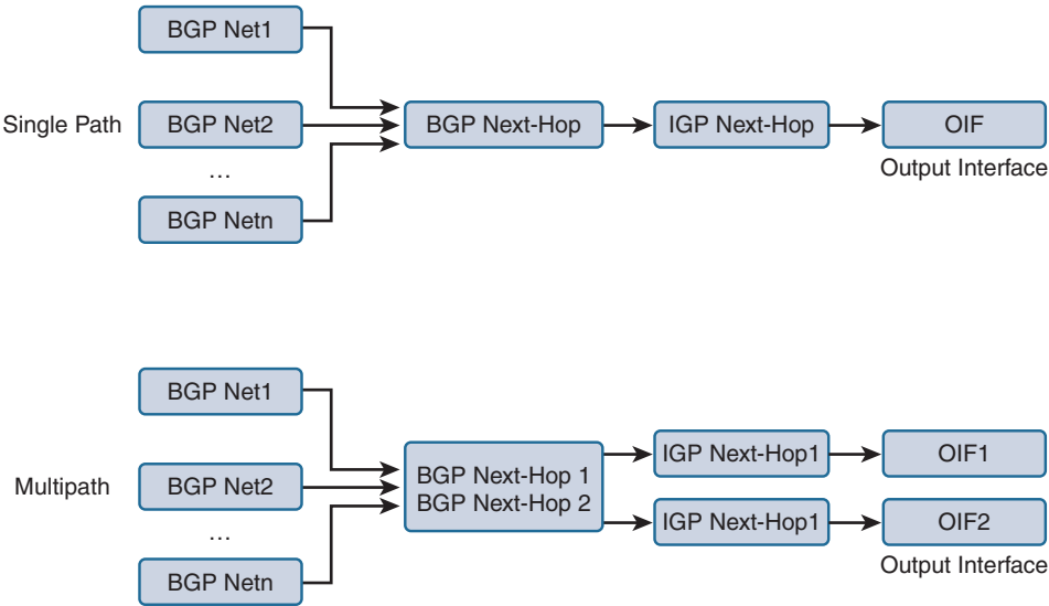
Figure 14-14 Hierarchical FIB Architecture
