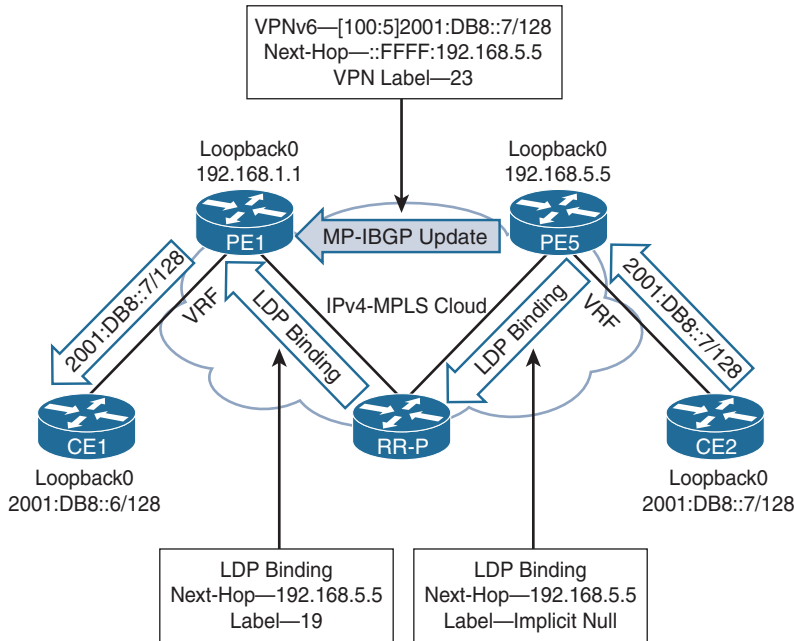
Figure 12-8 6VPE Control Plane
