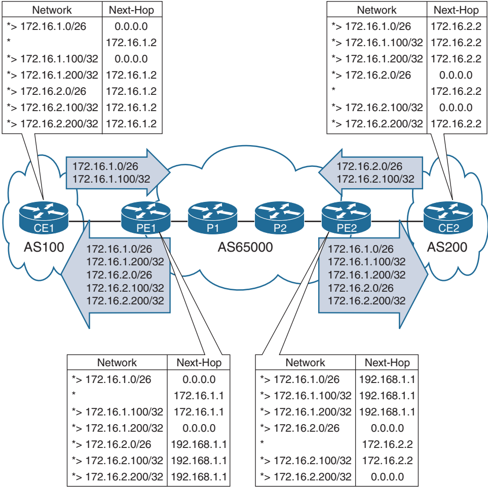
Figure 10-5 MPLS L3VPN Routing Tables Working Properly
