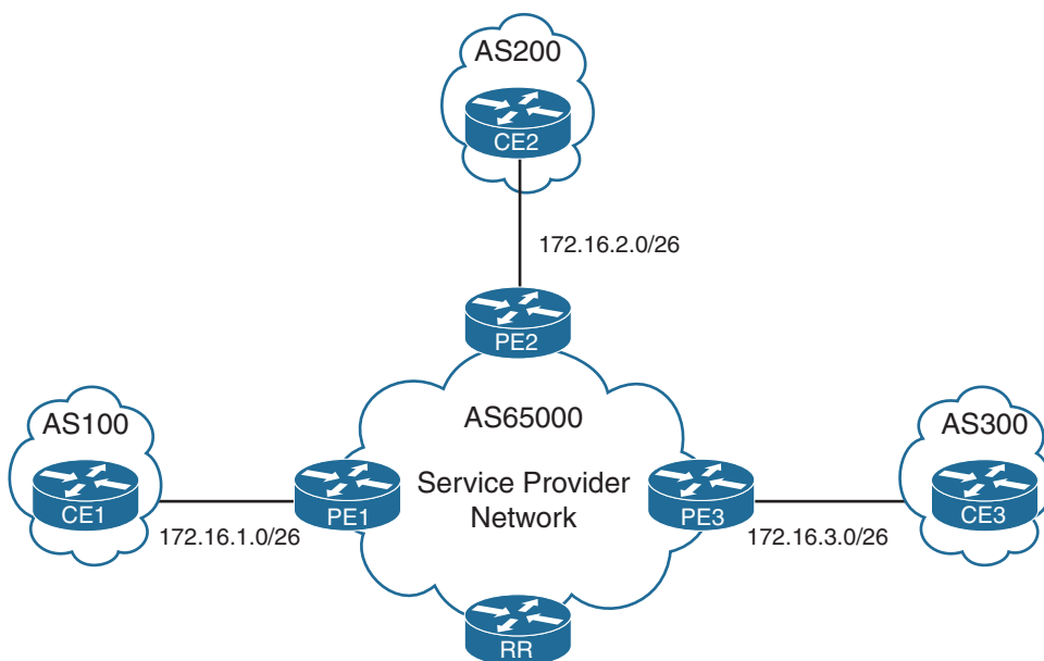
Figure 10-4 MPLS L3VPN Sample Topology
