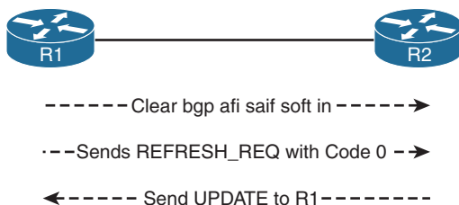
Figure 7-7 BGP Route Refresh
