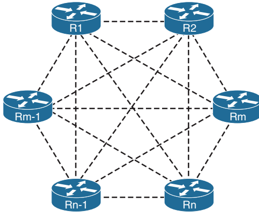
Figure 7-5 IBGP Full Mesh
