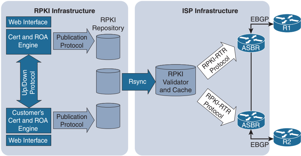
Figure 9-9 BGP Origin AS Validation System
