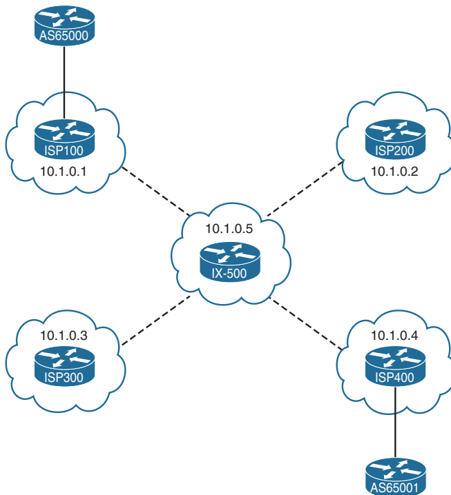
Figure 7-27 Topology with EBGp Peers and Route Server
