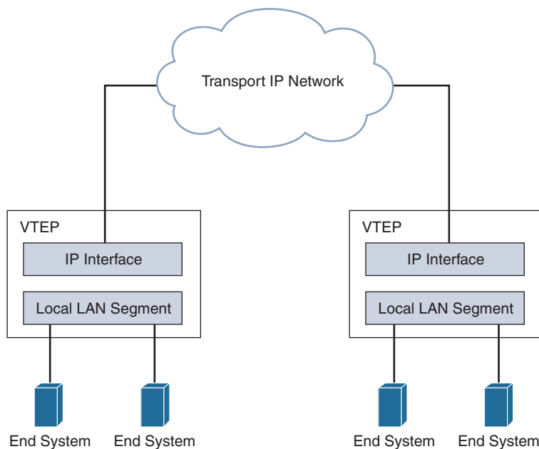
Figure 13-1 VTEP and End Systems
