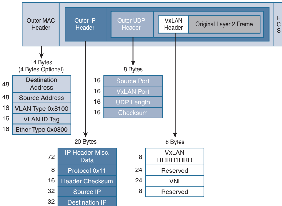
Figure 13-2 VxLAN Packet Format
