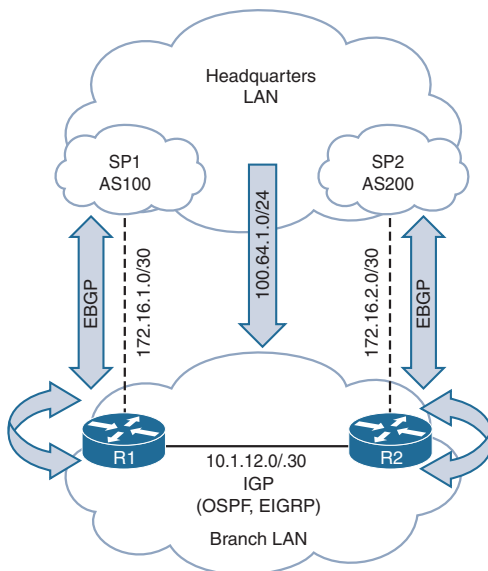
Figure 8-12 Topology for BGP Race Condition
