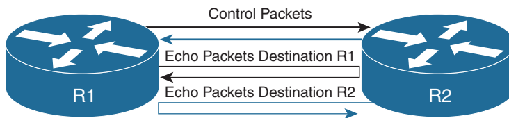
Figure 14-6 BFD Asynchronous Mode with Echo Function
