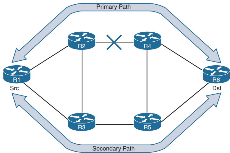
Figure 5-1 Topology with Primary and Secondary Path
