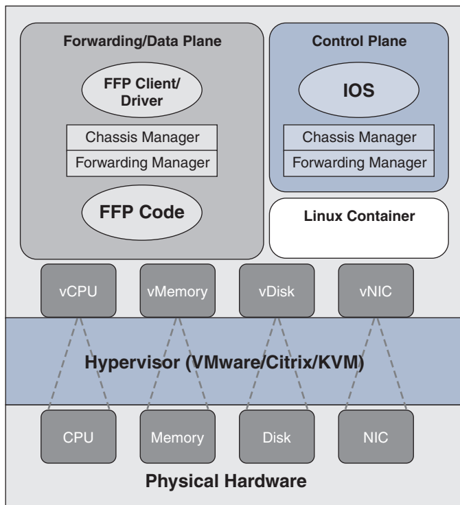
Figure 7-21 CSR1000v Architecture
