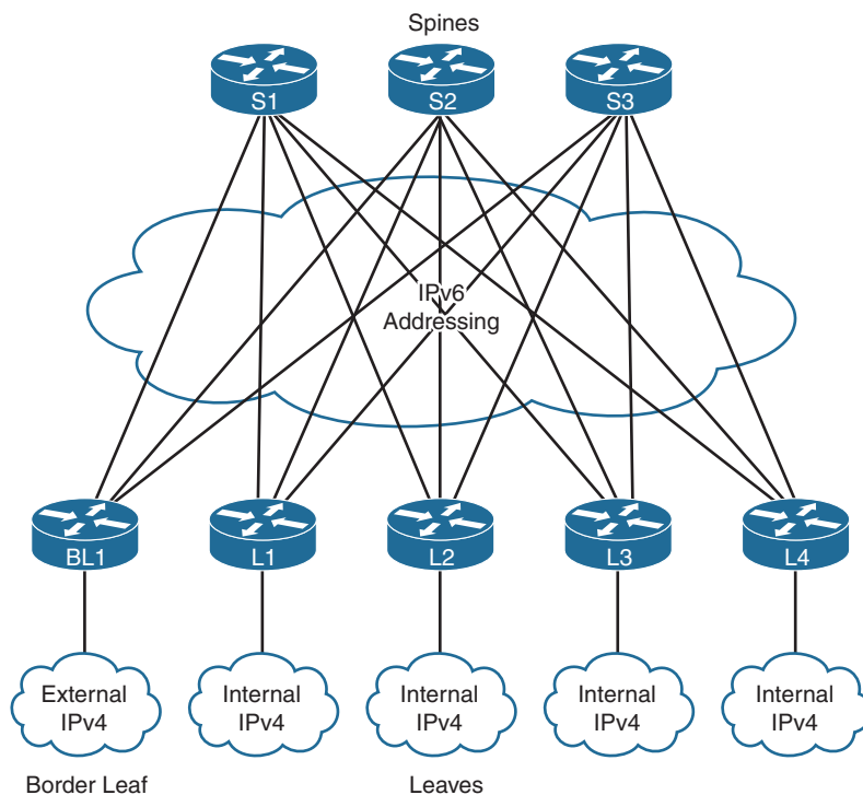
Figure 12-3 Spine-Leaf Topology
