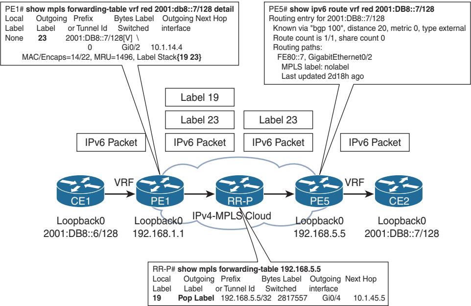
Figure 12-9 6VPE Data Plane
