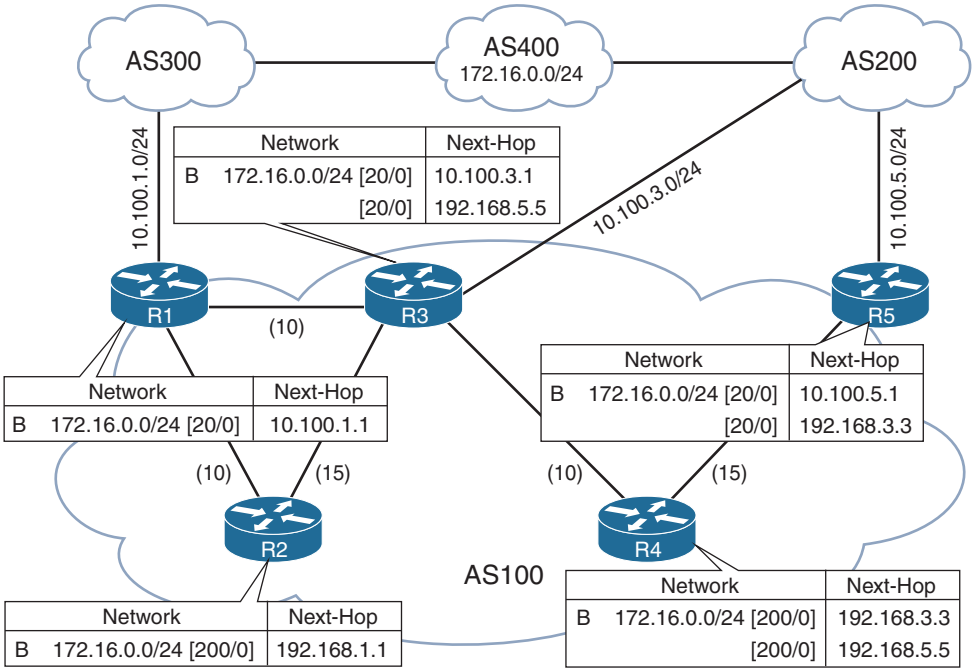
Figure 8-2 EIBGP Multipath Topology
