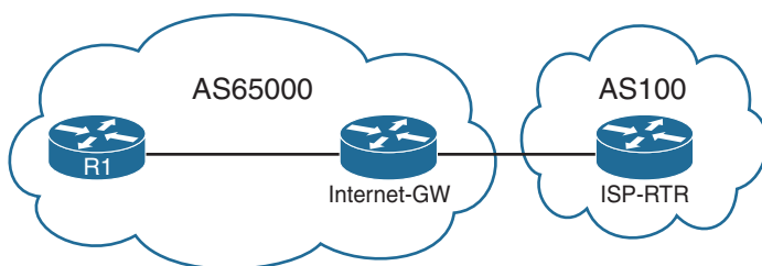
Figure 7-4 Enterprise-ISP BGP Peering
