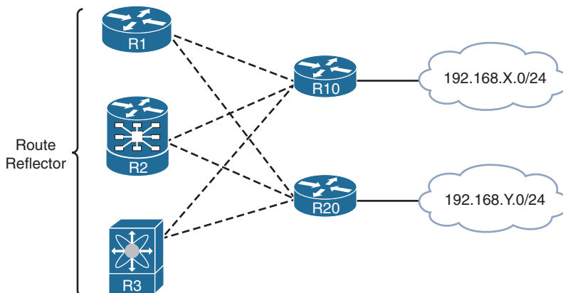
Figure 7-19 Selective Route Download Topology
