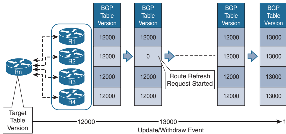
Figure 7-9 Updates When Route Refresh Is Received
