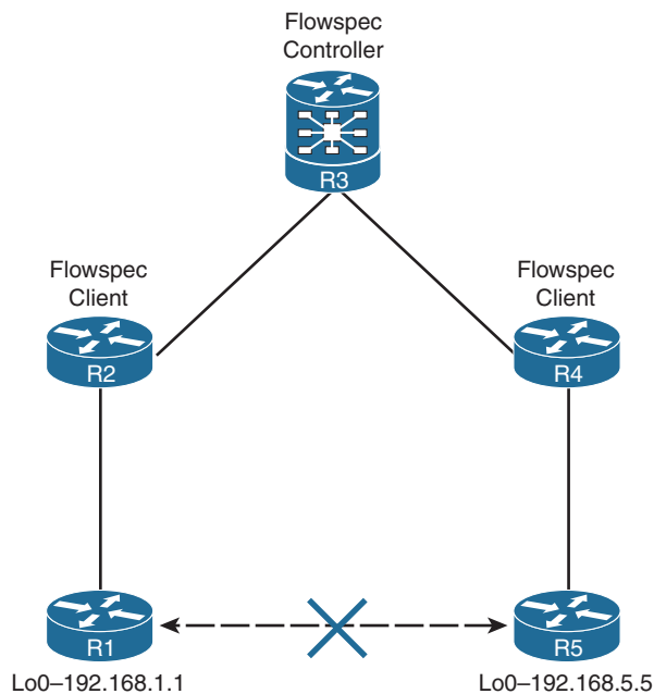
Figure 9-17 BGP Flowspec Topology
