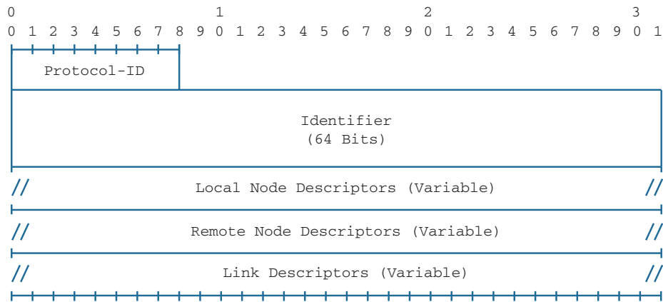
Figure 15-4 Type 2—Link NLRI
