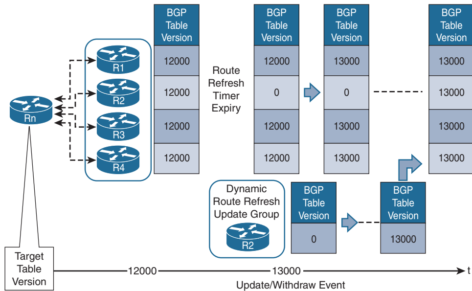
Figure 7-10 Updates with Dynamic Refresh Update Groups
