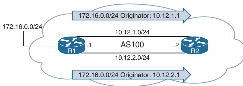
Figure 8-9 Lowest IP Address
