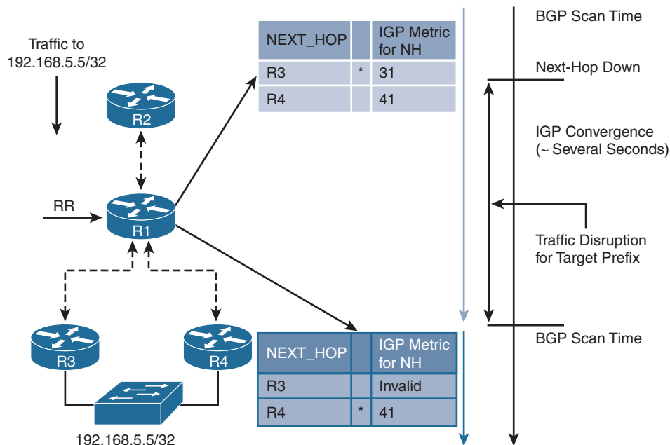
Figure 5-5 Ineffective NH Validity Check with BGP Scanner
