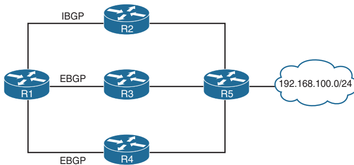
Figure 7-3 Topology with BGP Multipath
