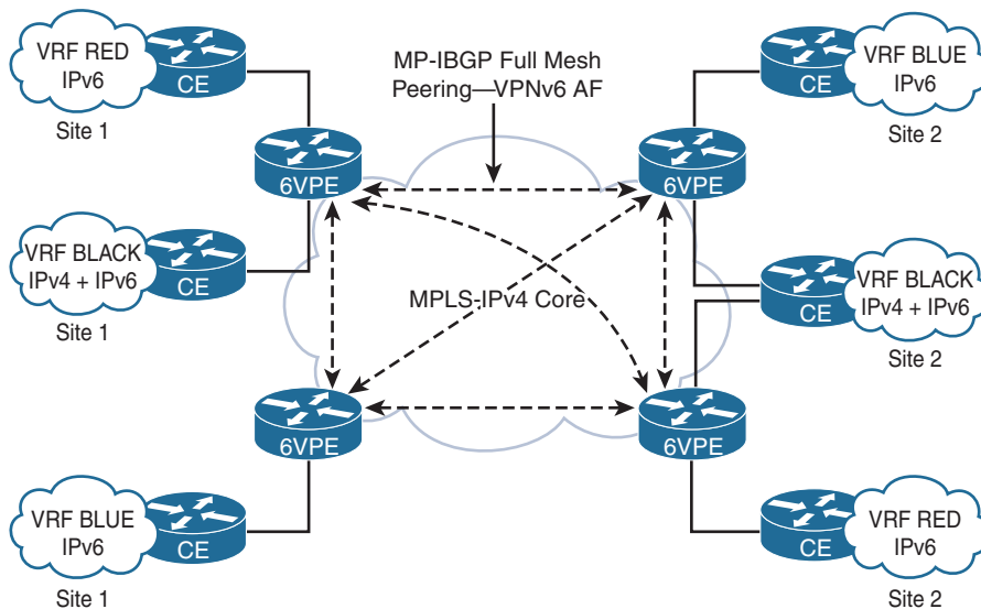
Figure 12-7 6VPE Architecture
