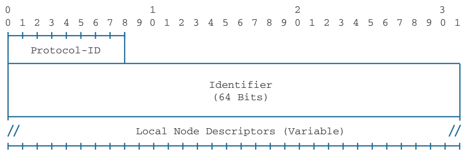
Figure 15-3 Type - Node NLRI
