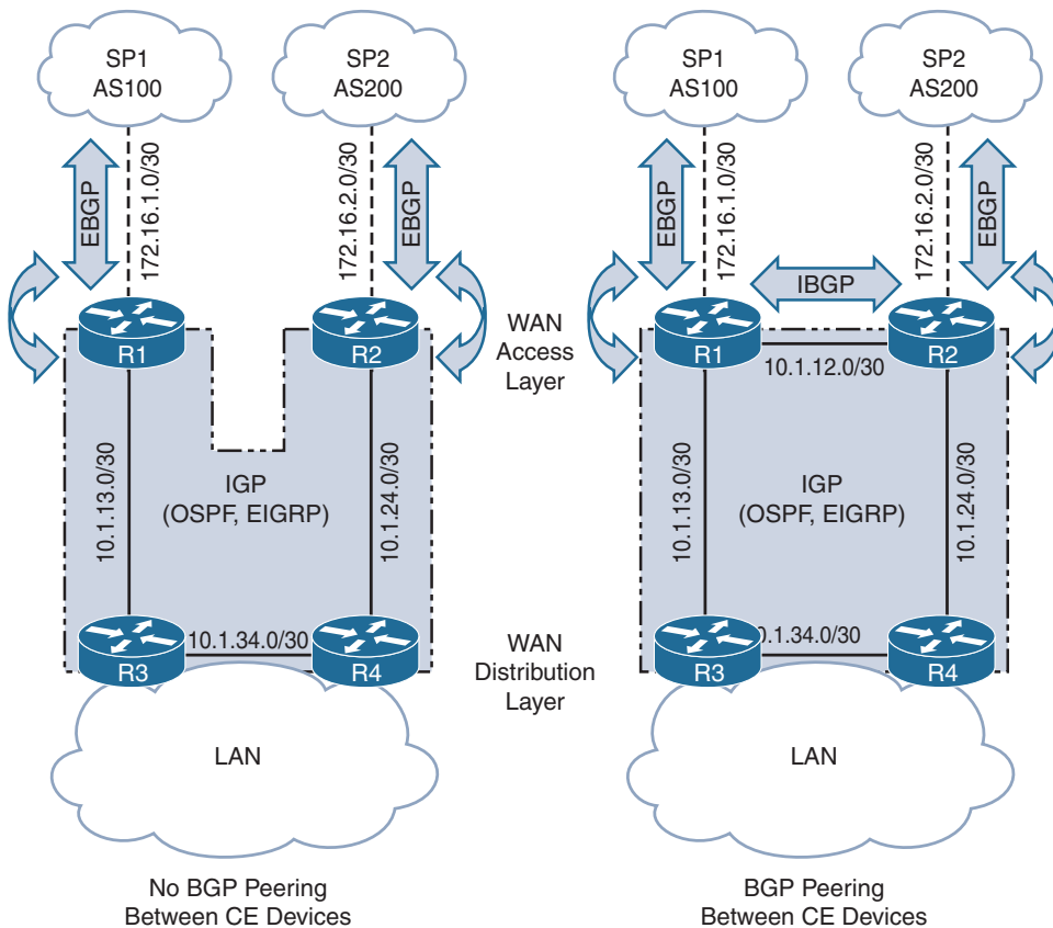
Figure 8-15 Options for Exchanging Routes Between LAN and WAN
