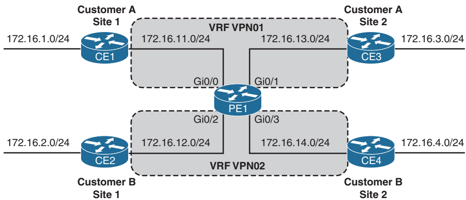
Figure 10-3 Separate Routing Domains Through VRFs
