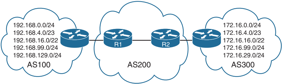
Figure 4-12 BGP Regex Reference Topology
