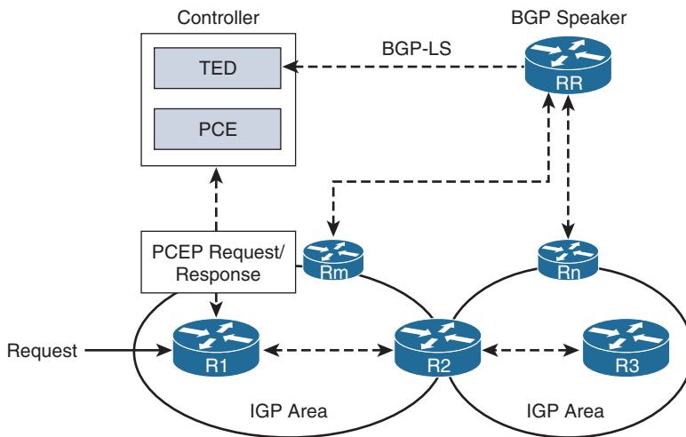
Figure 15-1 Topology with PCE as a Central Controller
