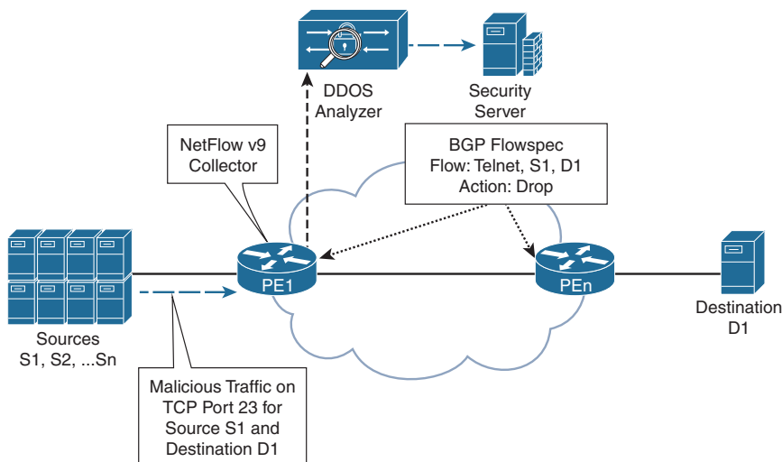
Figure 9-16 DDOS Mitigation Scenario
