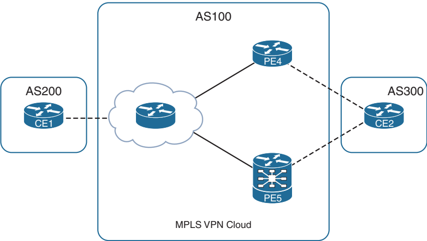
Figure 7-13 MPLS VPN Topology with ORF Filtering on PE
