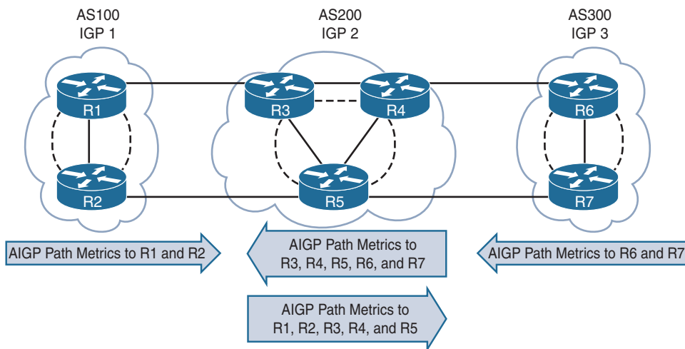
Figure 8-5 AIGP Path Attribute Exchange Between Autonomous Systems
