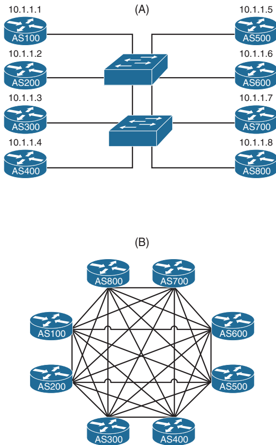
Figure 7-26 Public Peering at IX
