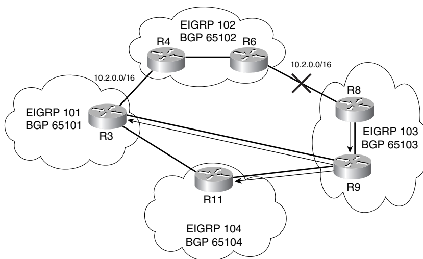
Figure 5-8 Path Updates on Link Failure Between R8 and R6
