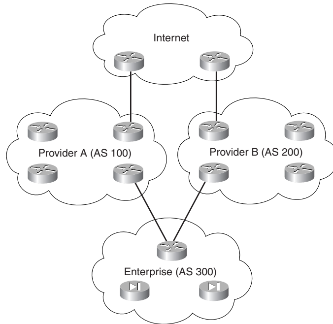
Figure 6-4 Multihomed Single Border Router Architecture
