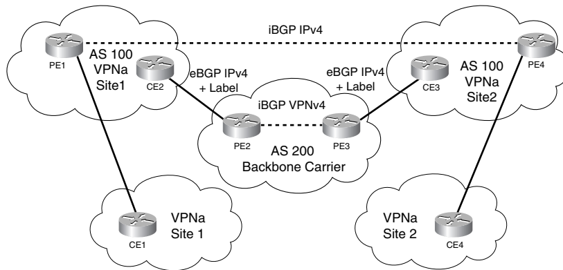
Figure 10-28 Hierarchical VPN
