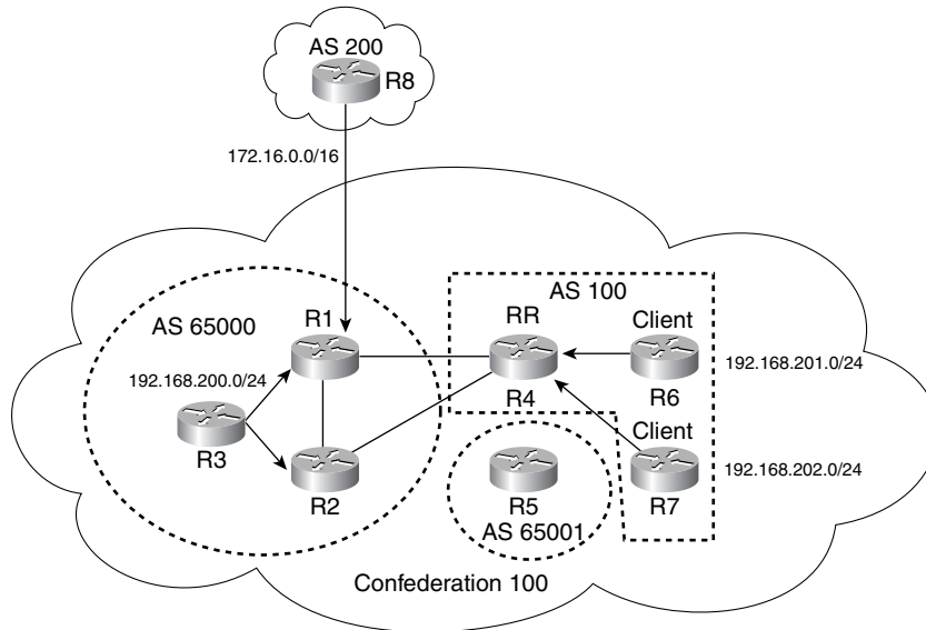
Figure 8-18 R7 in Member AS 100 and R5 out of the Forwarding Paths
