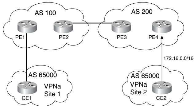
Figure 10-15 Sample Topology for Back-to-Back VRF
