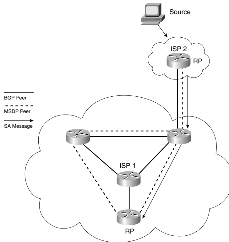
Figure 11-26 Route Reflection's Impact on MSDP SA RPF
