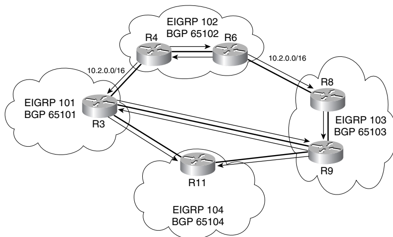
Figure 5-7 Complete Prefix Advertisement Scenario for 10.2.0.0/16
