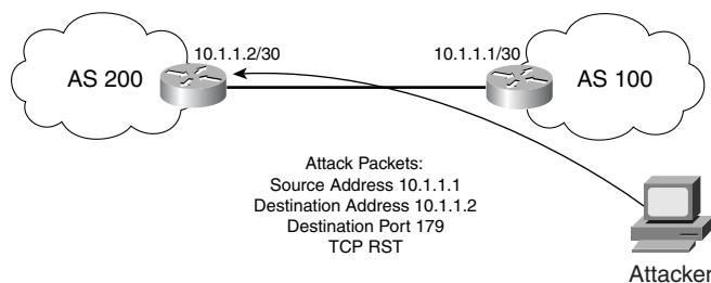
Figure 9-5 BGP TCP Reset Attack Scenario
