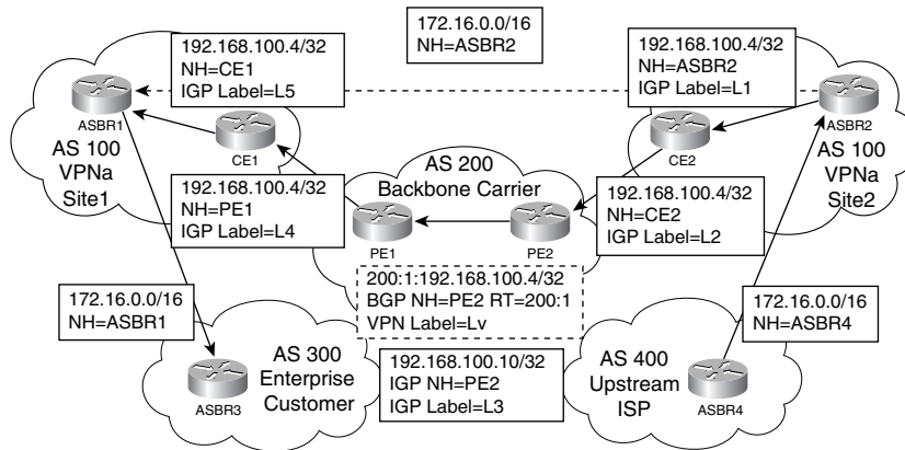
Figure 10-27 Prefix and Label Distribution for CSC
