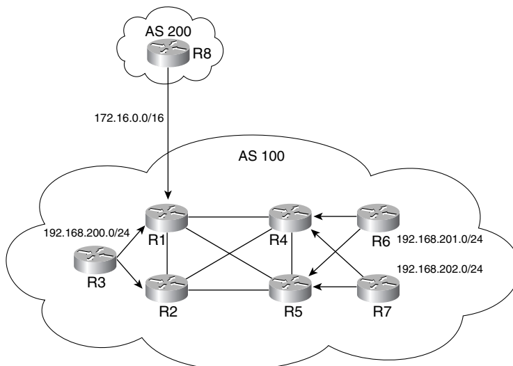
Figure 8-1 BGP Full-Mesh Topology
