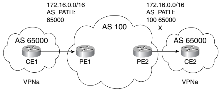
Figure 10-9 AS_PATH Loop Scenario
