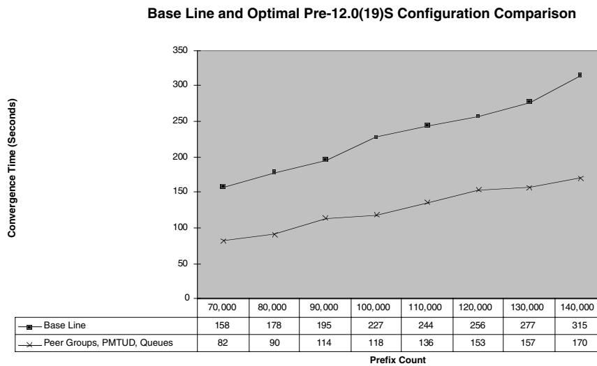
Figure 3-12 Baseline and Optimal Pre-Release 12.0(19)S Comparison
