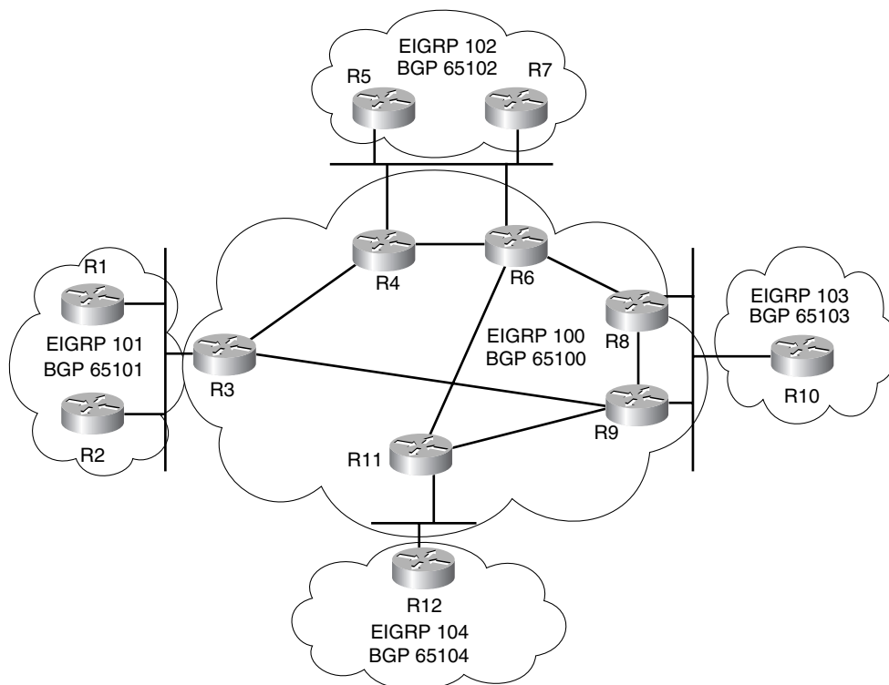
Figure 5-10 Internal/External BGP Architecture
