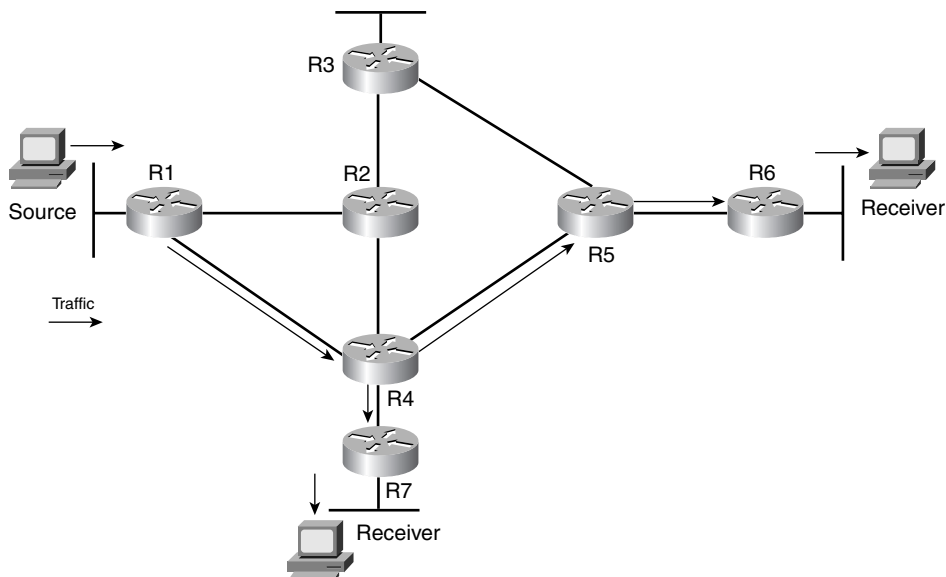
Figure 11-11 Final MDT for the PIM-DM Network
