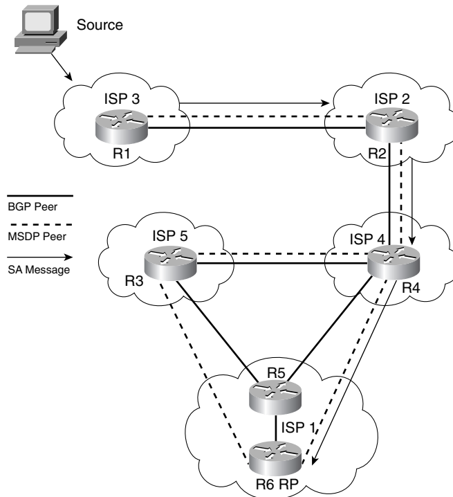
Figure 11-23 MSDP SA RPF Succeeds Without Matching the BGP Session
