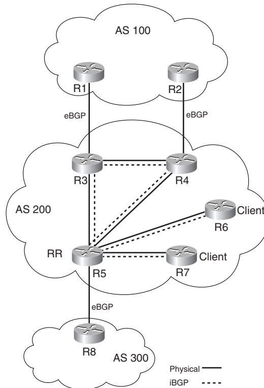
Figure 7-2 BGP Route Reflection Components
