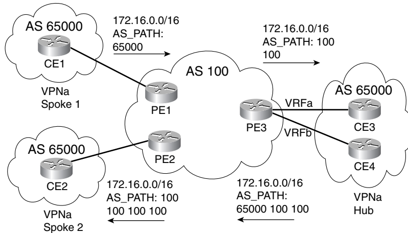
Figure 10-12 Hub-and-Spoke VPN
