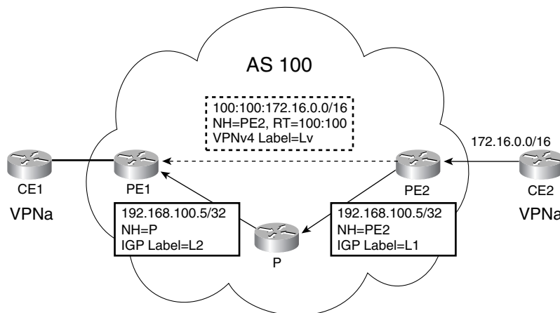
Figure 10-7 MPLS VPN Route and Label Propagation
