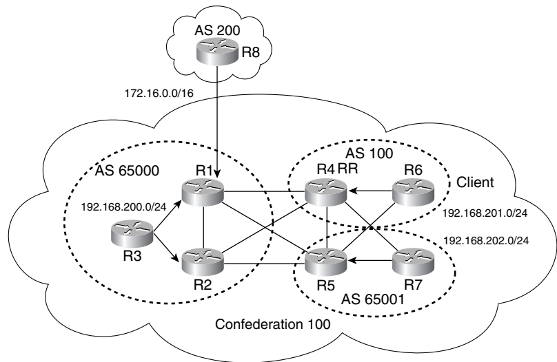
Figure 8-17 R6 in AS 100 and R4 in the Forwarding Paths
