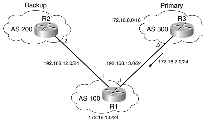
Figure 4-2 Conditional Advertisement in a Primary-Backup Scenario
