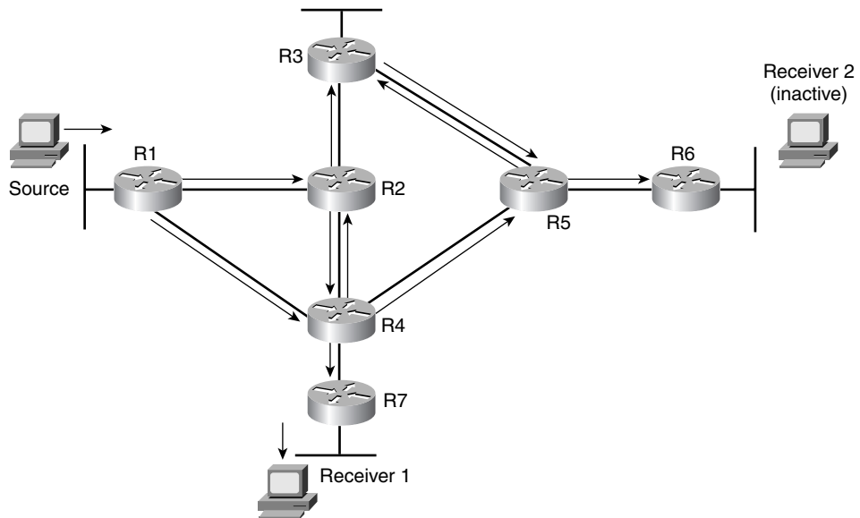
Figure 11-8 Initial Traffic Flooding in the PIM-DM Network
