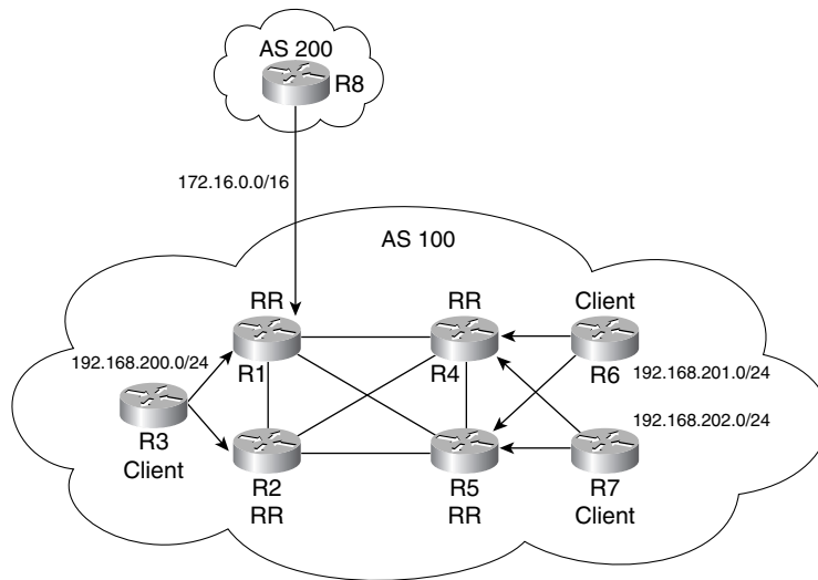
Figure 8-2 RR-Based Topology
