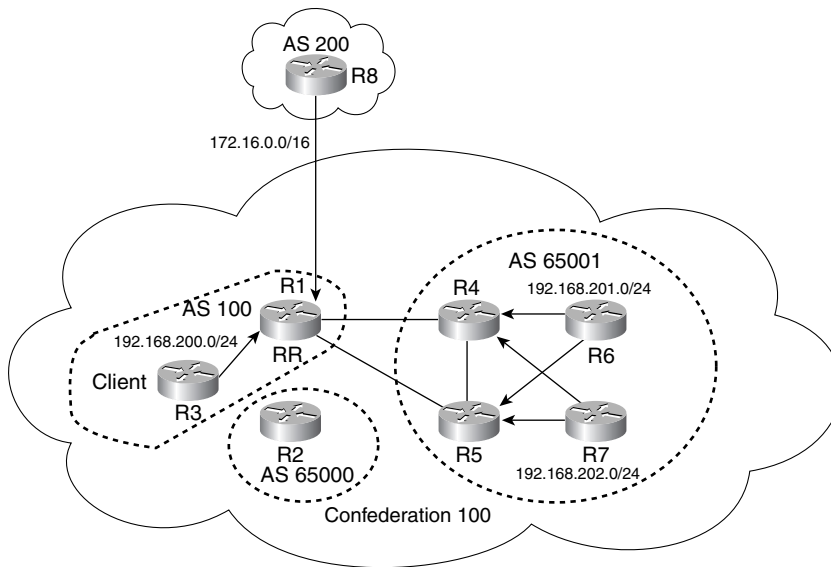
Figure 8-14 Current Network Topology
