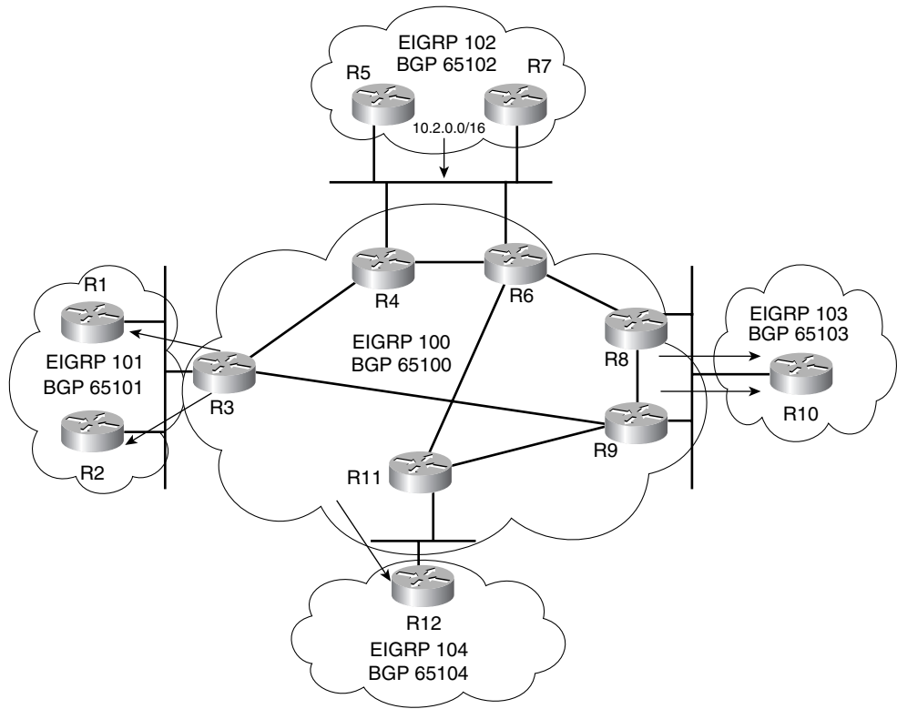
Figure 5-12 Prefix Advertisement for 10.2.0.0/16 to Regions
