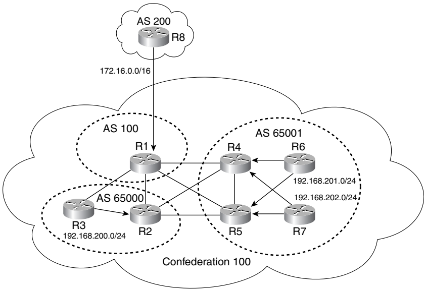
Figure 8-9 R3 Moved to AS 65000
