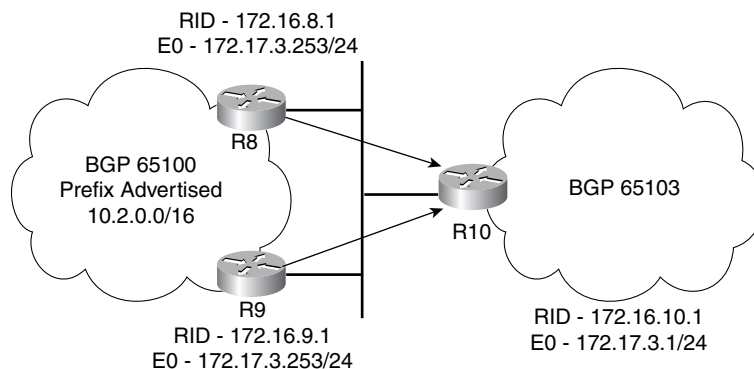
Figure 5-15 Detailed DMZ Between AS 65100 and AS 65103
