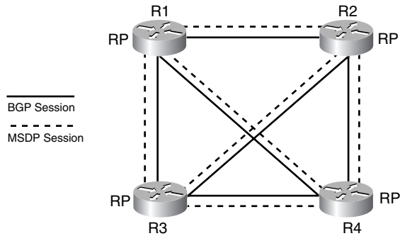
Figure 11-27 RP Anycast Network Core
