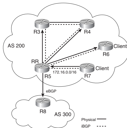
Figure 7-5 Prefix Advertisement for RR Clients
