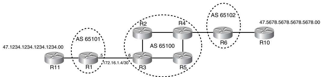
Figure A-5 Sample Network Topology
