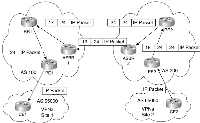
Figure 10-33 Label-Forwarding Path
