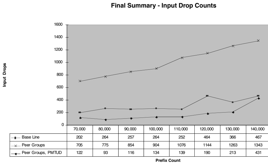
Figure 3-14 Final Summary Input Drop Counts
