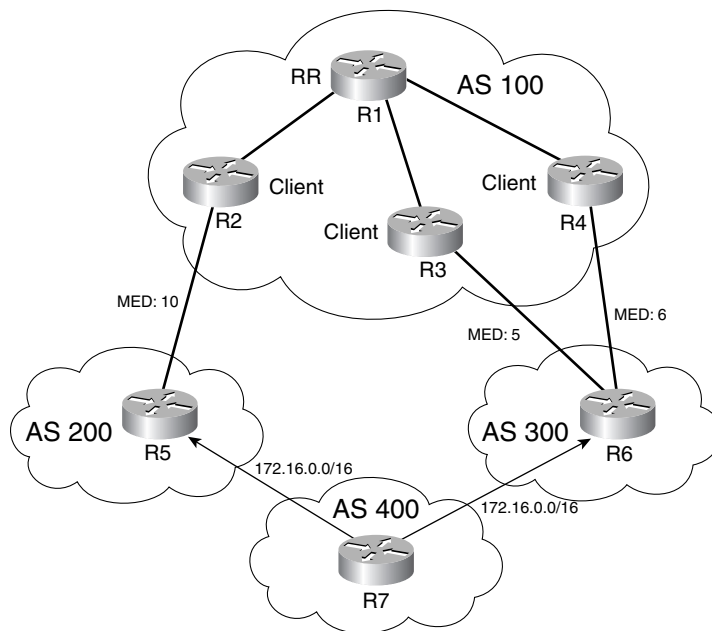
Figure 7-17 Persistent Convergence Oscillation
