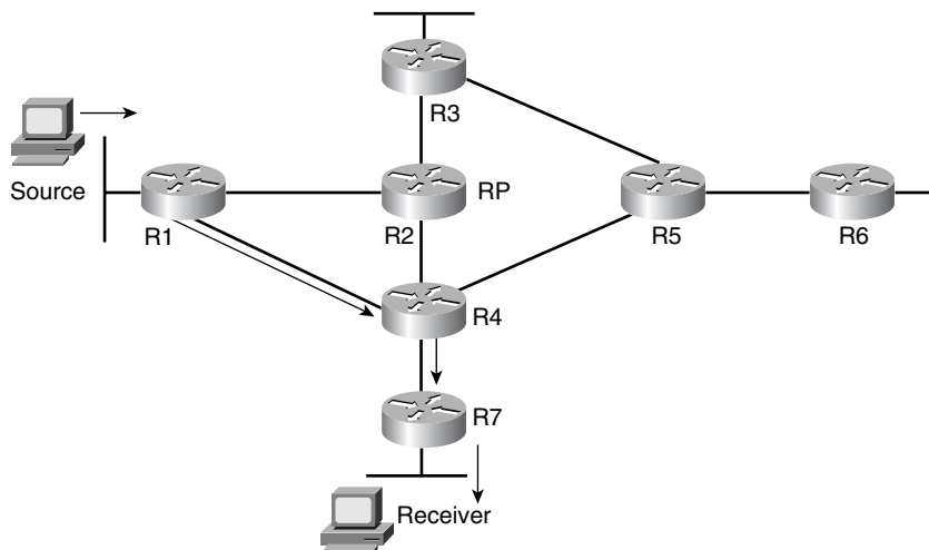
Figure 11-17 Final MDT for the PIM-SM Network
