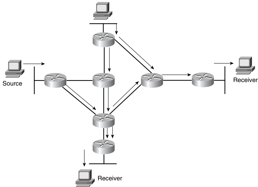
Figure 11-5 Source Tree Distribution Tree
