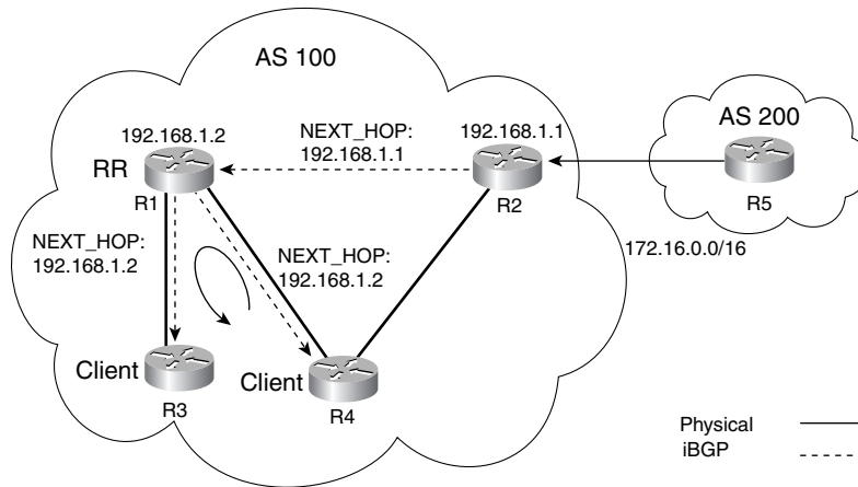
Figure 7-28 Improper Next-Hop Setting Leads to Routing Loops
