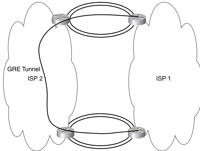
Figure 9-8 Virtual Backbone Links Using GRE
