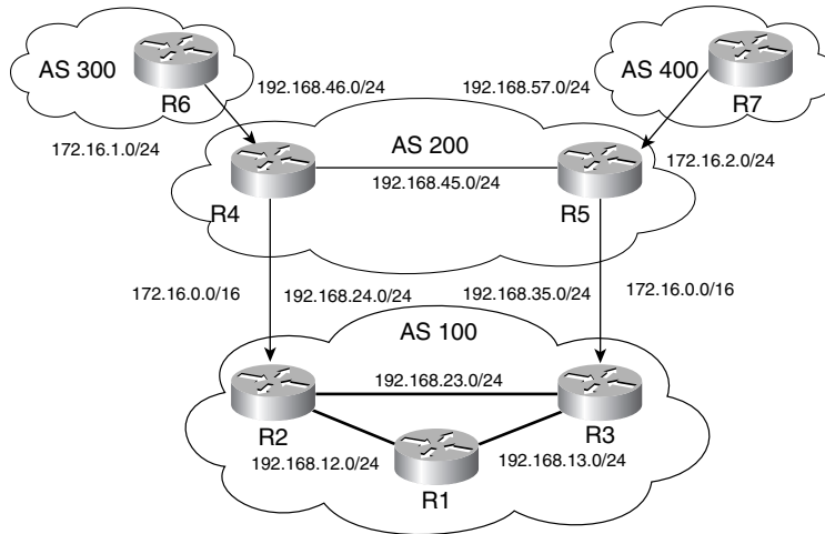
Figure 4-4 Example of Conditional Injection
