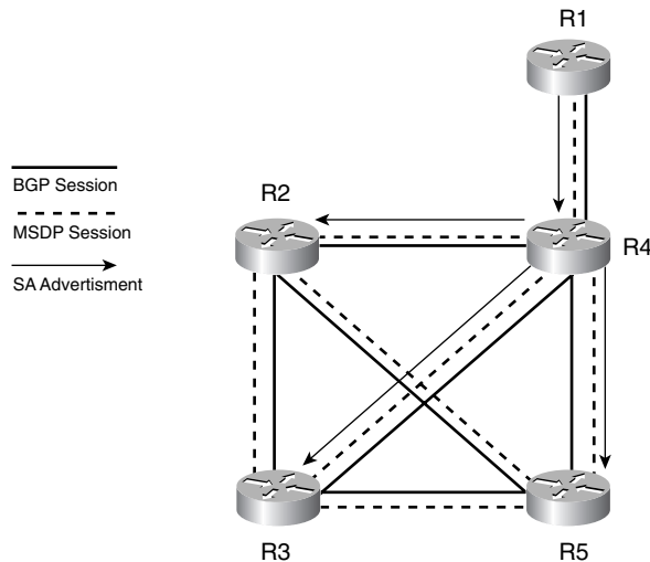
Figure 11-25 MSDP SA Flooding with Mesh Groups
