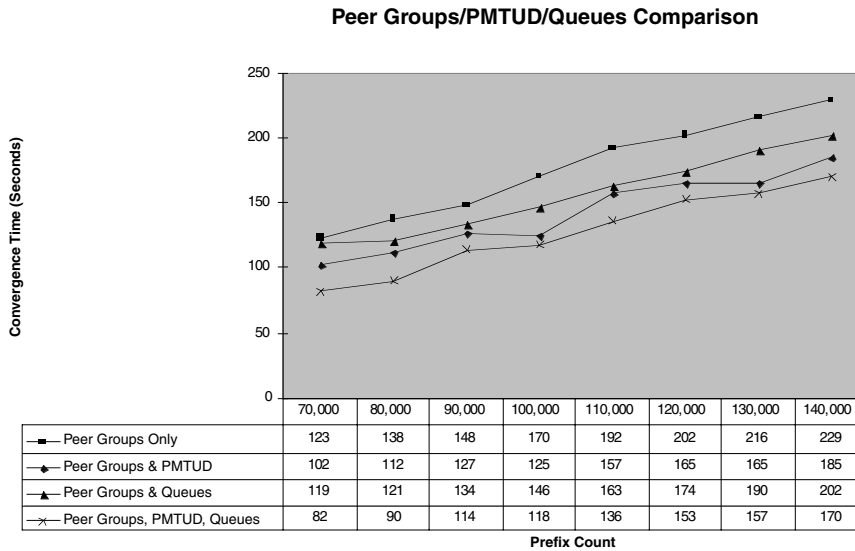
Figure 3-11 Peer Group, PMTUD, and Queue Optimization Statistics
