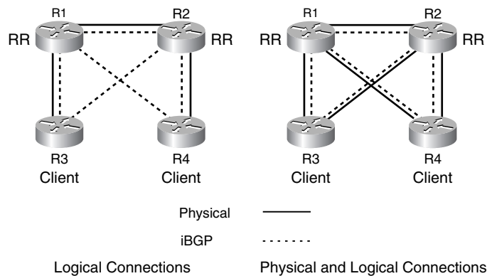
Figure 7-13 Physical Topology Balances with the Logical Topology
