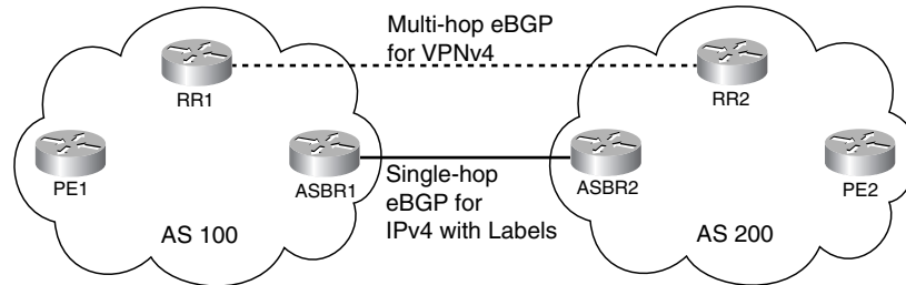
Figure 10-20 Multihop Multiprotocol eBGP Using RRs
