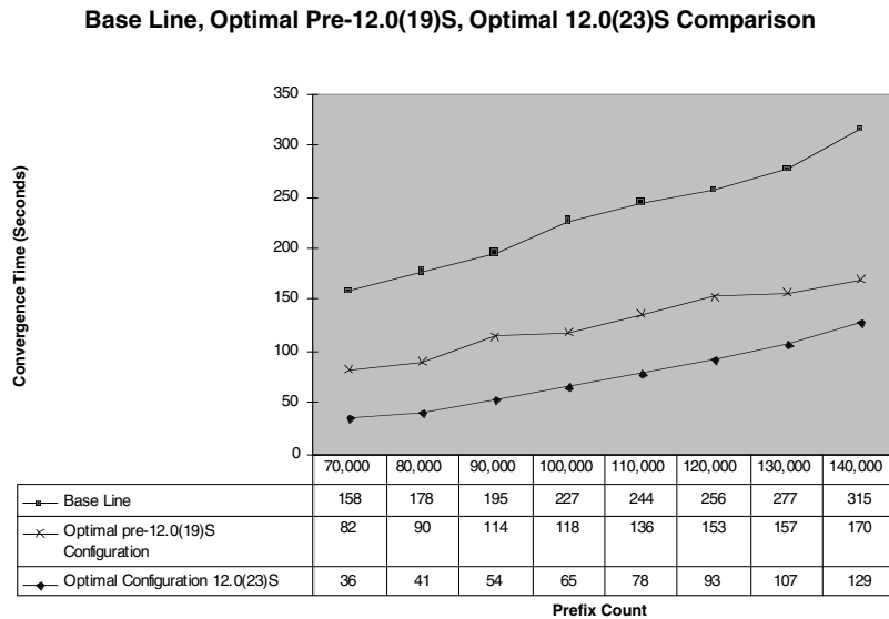
Figure 3-13 Baseline, Pre-12.0(19)S, and 12.0(23)S Comparison
