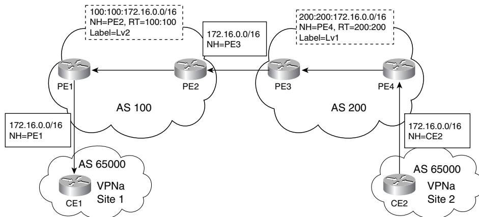
Figure 10-16 VPN Prefix and Label Advertisement in Back-to-Back VRF
