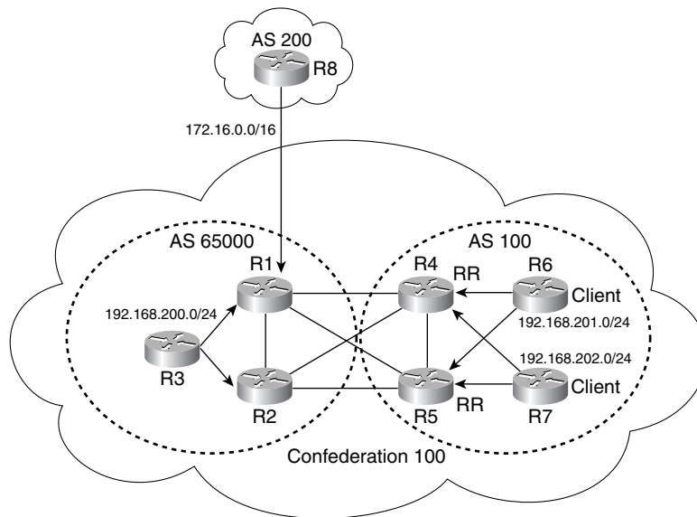
Figure 8-19 Current Network Topology
