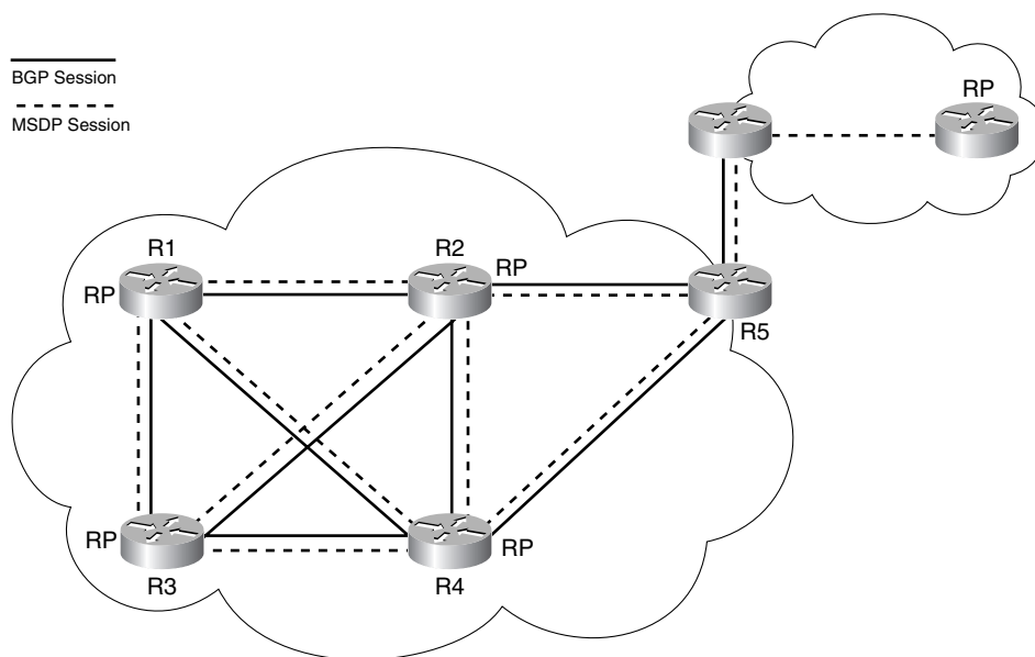
Figure 11-32 Interdomain Multicast Peering Placement
