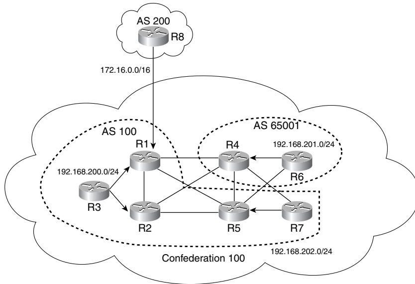
Figure 8-5 Current Network Topology
