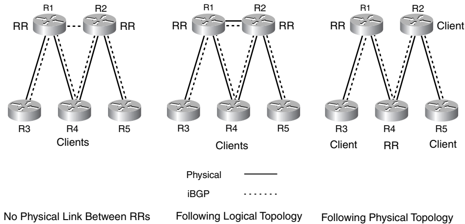
Figure 7-12 Following the Physical Topology
