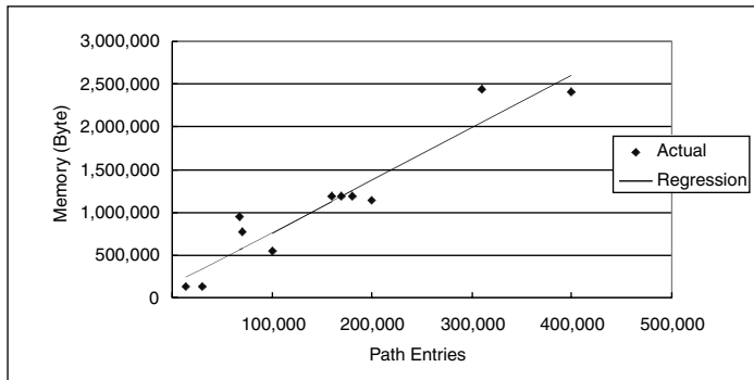
Figure 2-10 Memory Use for BGP Path Attributes
