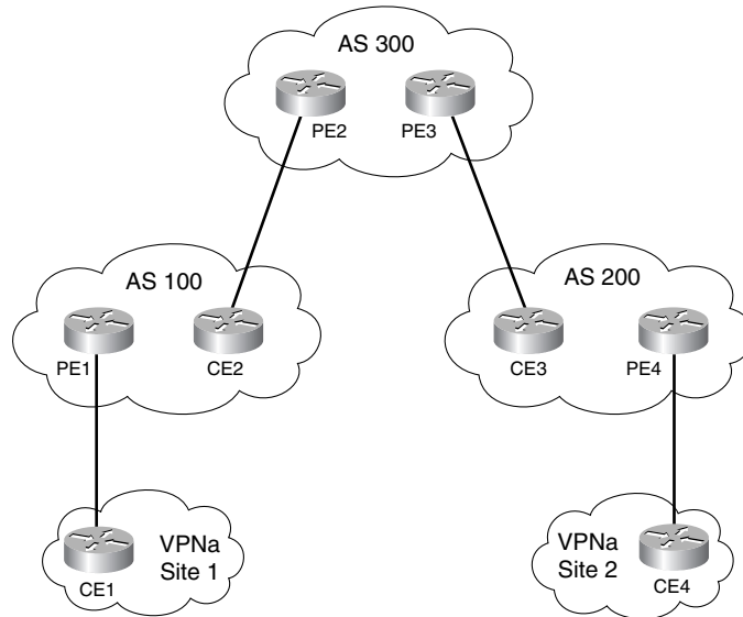
Figure 10-14 MPLS VPN over a Common Transit VPN Backbone
