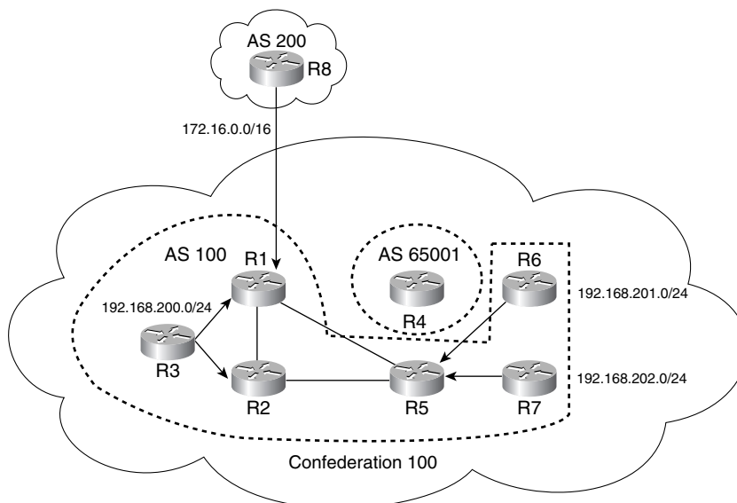
Figure 8-4 Current Network Topology
