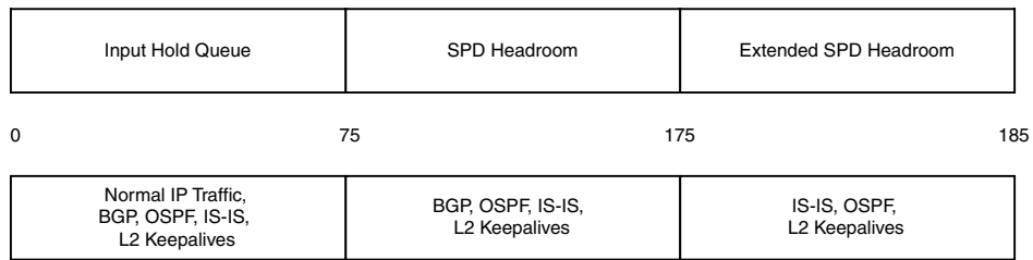
Figure 3-3 Input Hold Queue Layout
