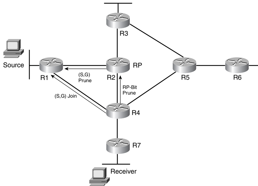
Figure 11-16 SPT Switchover Process
