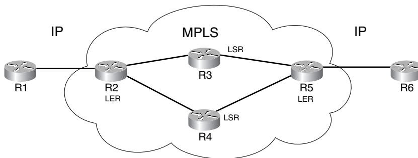
Figure 10-1 MPLS Network
