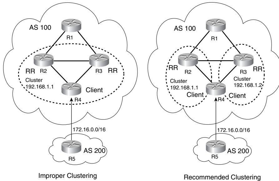
Figure 7-27 RR Clustering Design
