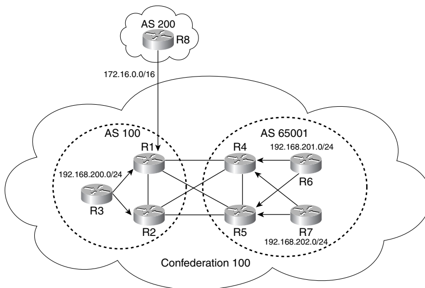
Figure 8-7 Current Network Topology
