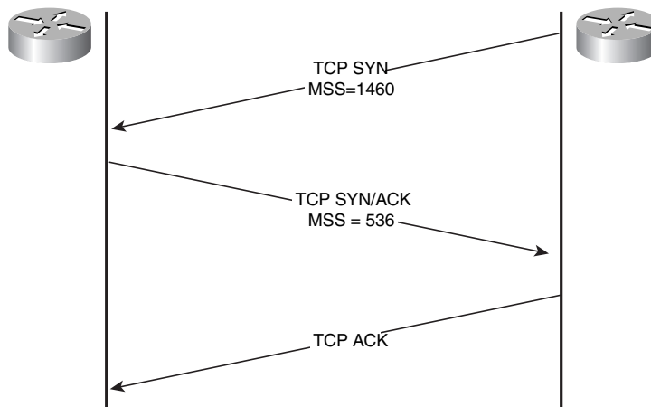
Figure 3-1 TCP Session Establishment and MSS Determination
