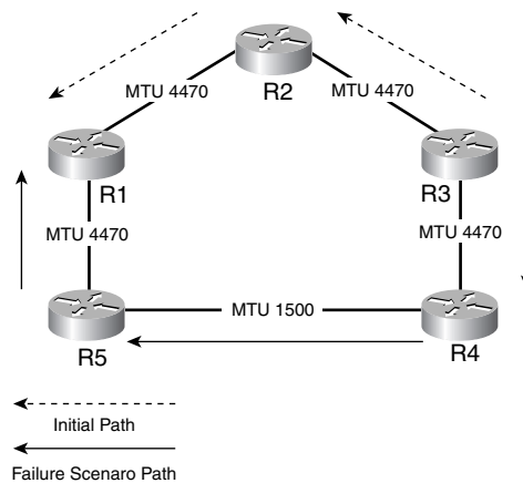
Figure 3-2 Path MTU Discovery Path Change Scenario
