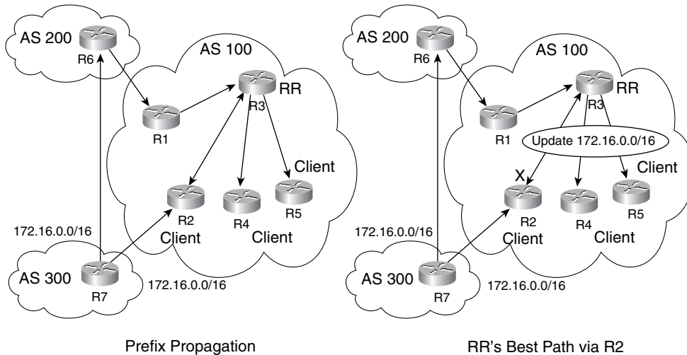
Figure 7-32 Peer Groups with RR for IOS 12.0 or Later
