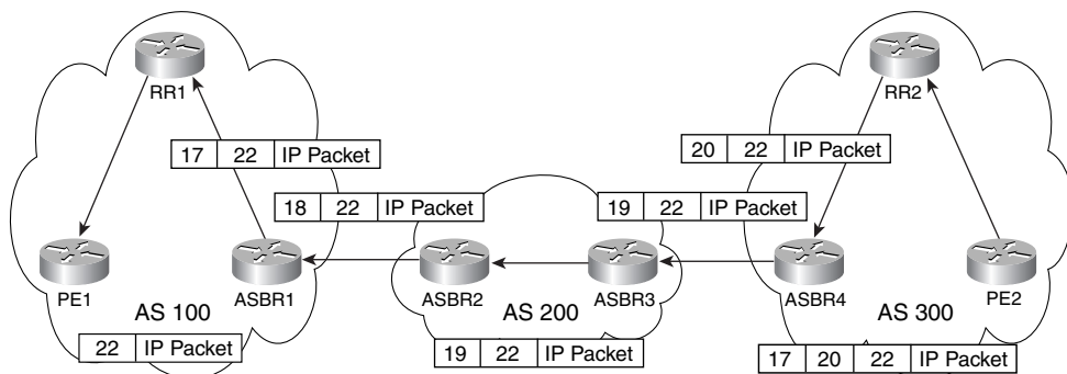
Figure 10-25 Packet Forwarding with a Non-VPN Transit AS
