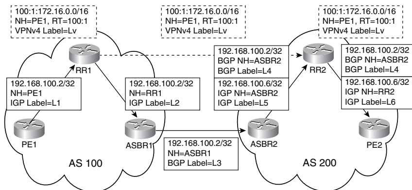
Figure 10-22 Label Exchange with Multihop eBGP Between RRs Using iBGP with Labels
