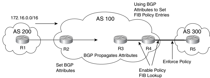
Figure 4-8 How QoS Policy Propagation via BGP Works
