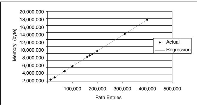
Figure 2-9 Memory Use for BGP Paths
