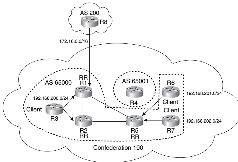
Figure 8-10 Current Network Topology
