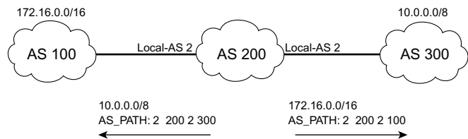
Figure 4-6 Local AS in Two Connections
