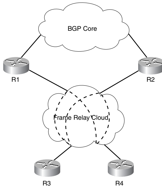
Figure 5-19 Remote Site Connectivity Black Hole Example
