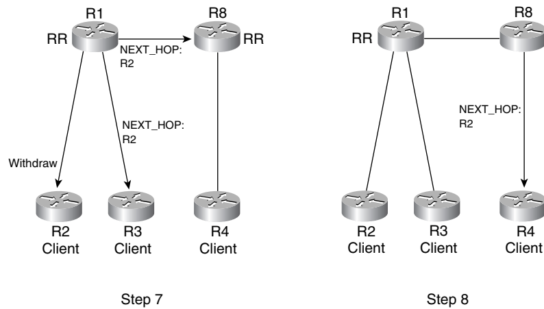
Figure 7-24 Prefix Propagation in Steps 7 and 8
