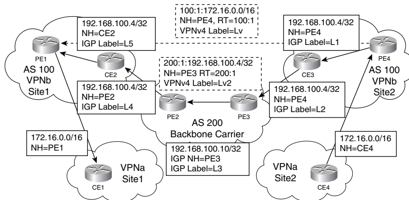
Figure 10-29 Prefix and Label Distribution for Hierarchical VPN
