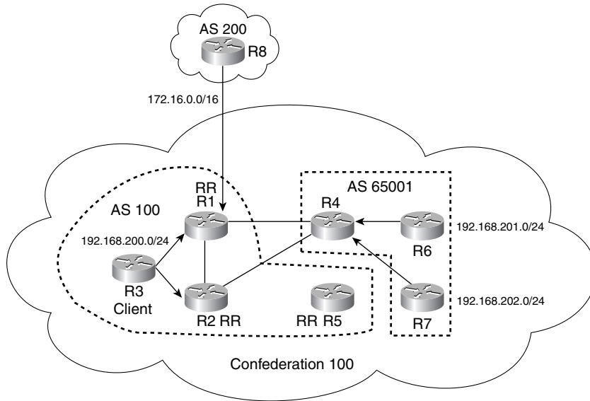
Figure 8-12 Current Network Topology
