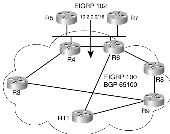
Figure 5-2 Path Advertisement into the Network Core for 10.2.0.0/16
