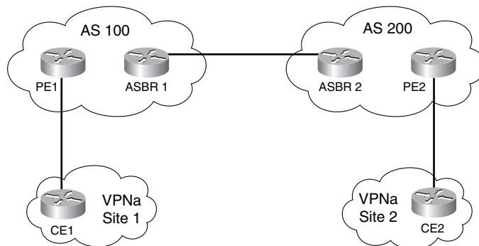
Figure 10-13 MPLS VPN over Two Provider Backbones
