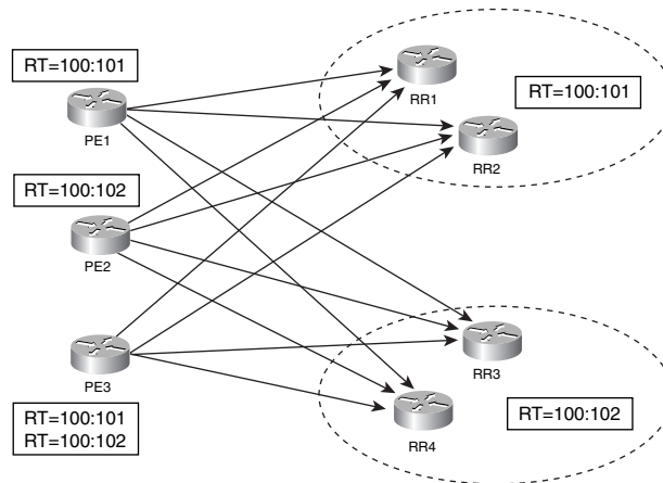
Figure 10-31 Partitioning RRs with RR Groups
