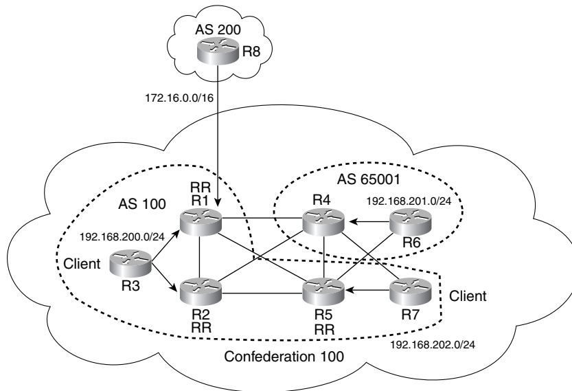
Figure 8-11 Current Network Topology
