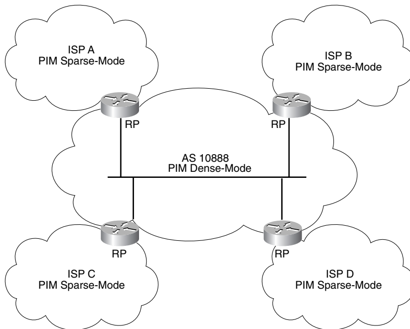
Figure 11-18 Multicast Internet Exchange
