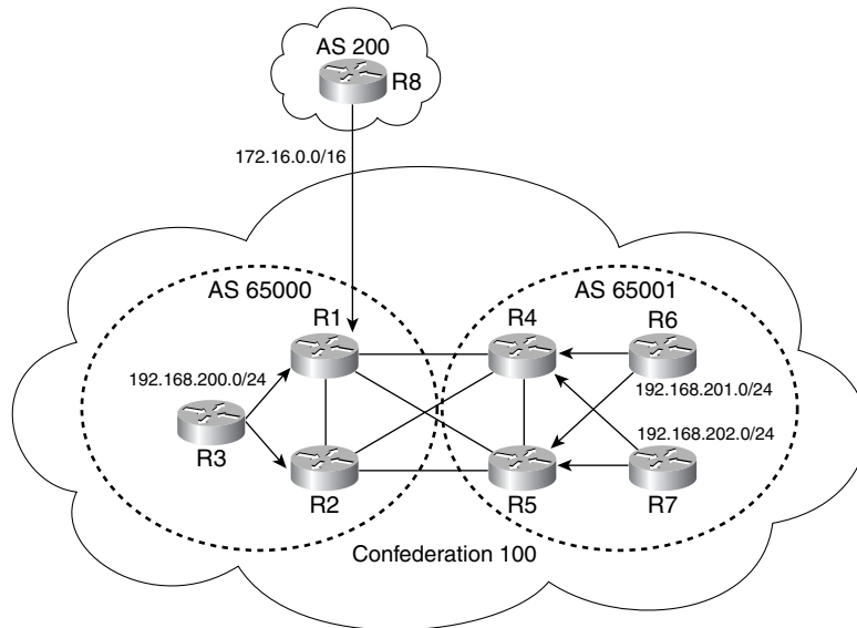
Figure 8-3 Confederation-Based Topology
