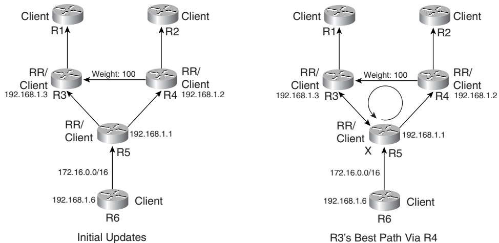
Figure 7-9 How CLUSTER_ID Breaks a Loop
