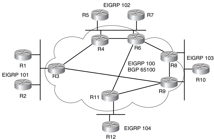
Figure 5-1 Core Architecture Using iBGP
