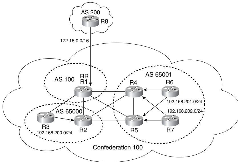
Figure 8-15 R3 Moved to AS 65000
