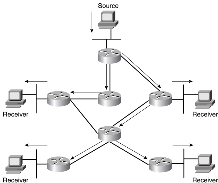
Figure 11-2 Multicast Delivery Model Efficiency Gains
