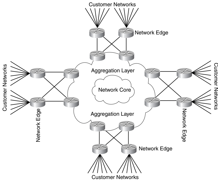
Figure 9-3 Network Edge
