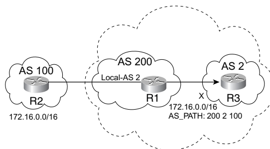
Figure 4-7 Updates Denied on R3 with Local AS on R1
