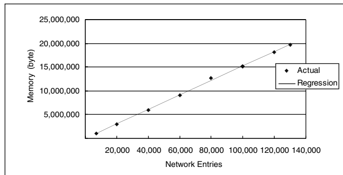
Figure 2-13 Memory Use for IP CEF
