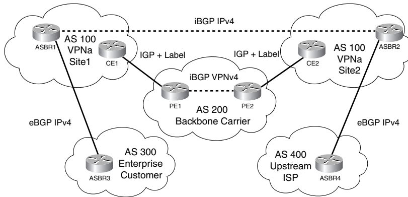
Figure 10-26 Full Internet Routes via VPN
