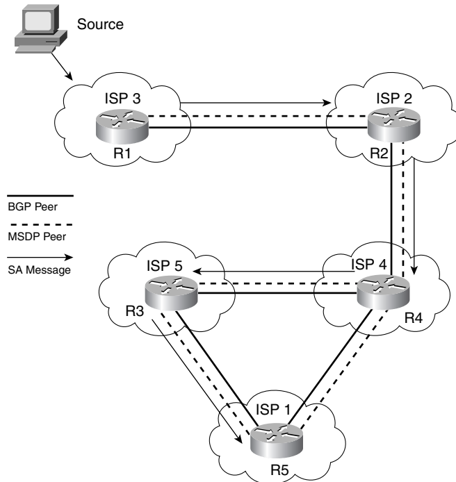
Figure 11-22 Failed eBGP-Based MSDP SA RPF
