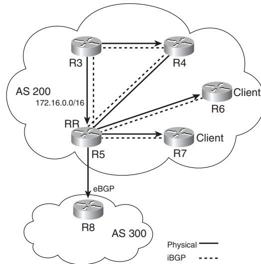
Figure 7-4 Prefix Advertisement for Internal Peers
