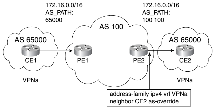
Figure 10-10 AS Override Allows CE-CE Communication
