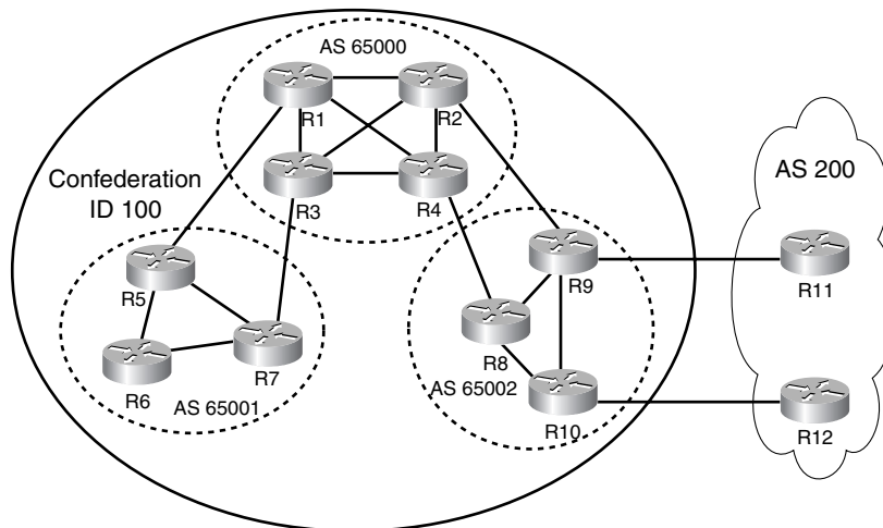
Figure 7-33 BGP Confederation
