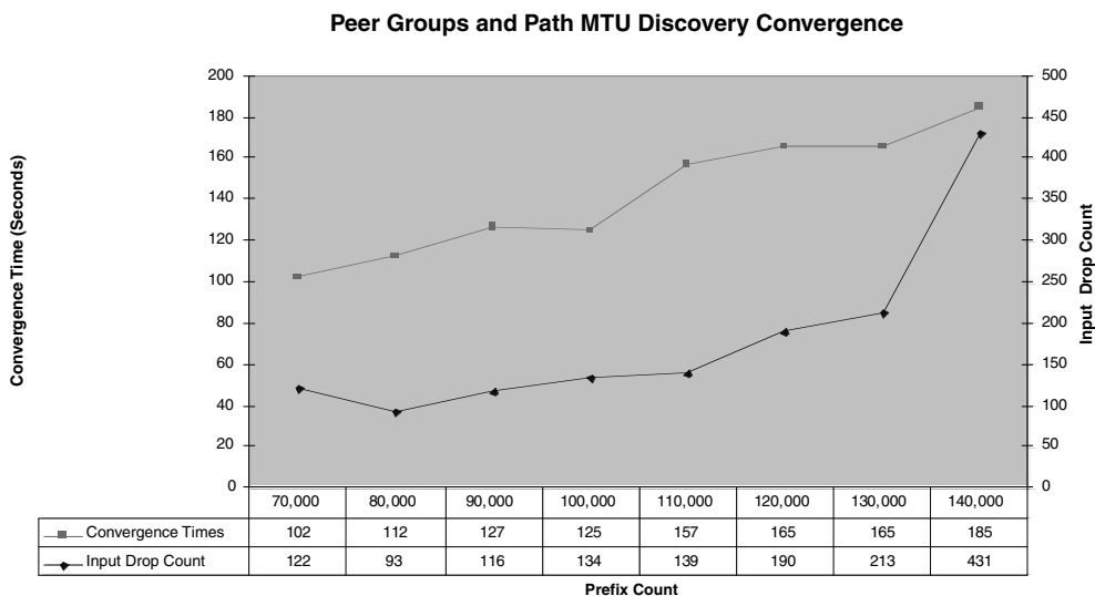
Figure 3-9 Peer Group and Path MTU Convergence Statistics
