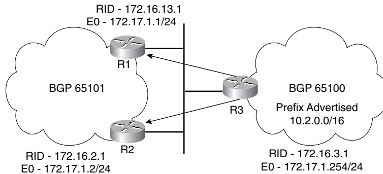
Figure 5-14 Detailed DMZ Between AS 65100 and AS 65101
