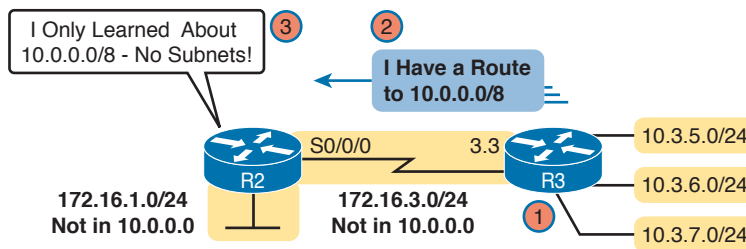
Figure G-12 Autosummarization Example
