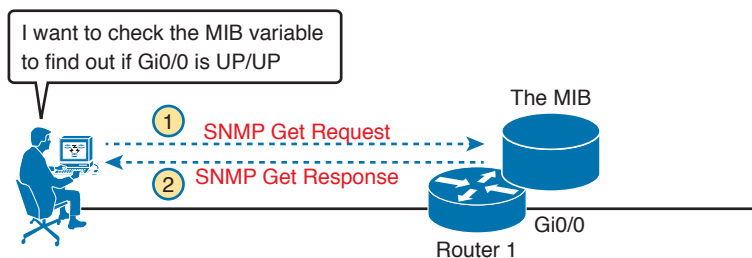
Figure 26-2 SNMP Get Request and Get Response Message Flow
