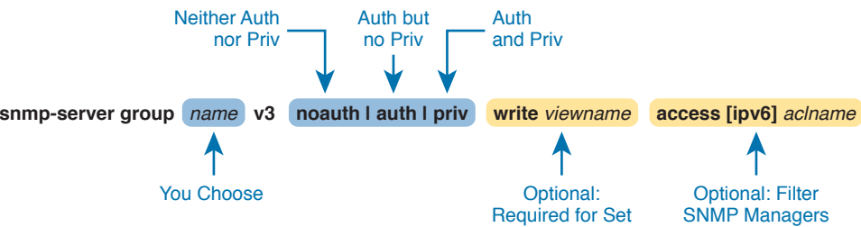
Figure 26-7 SNMPv3 Groups—Configuration Command Parameters
