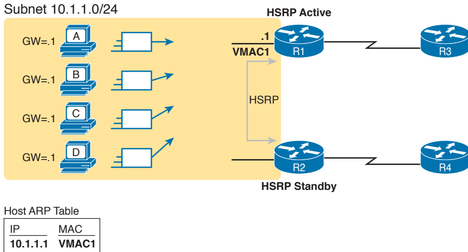
Figure 20-5 All Traffic Goes to .1 (R1, Which Is Active); R2 Is Standby
