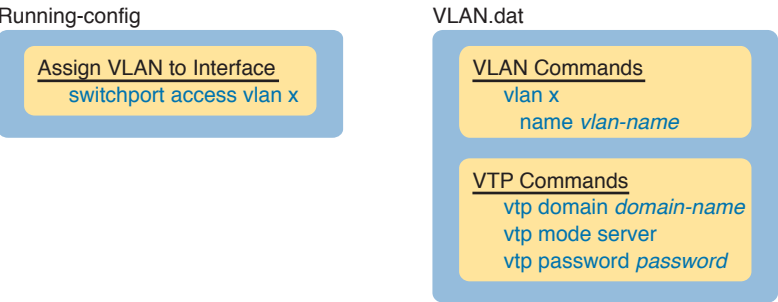
Figure 5-9 Where VTP Stores Configuration: VTP Client and Server
