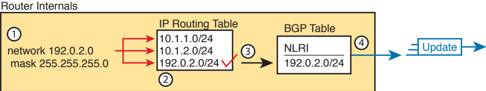
Figure 12-14 Configuration Concept: the BGP network Command
