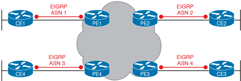
Figure 14-22 Routing Protocol Neighbor Relationships with EIGRP
