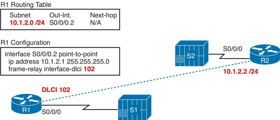
Figure I-8 Configuration Facts Related to R1's Failed ping 10.1.2.2 Command
