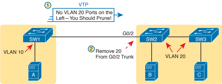
Figure 5-6 VTP Pruning Example
