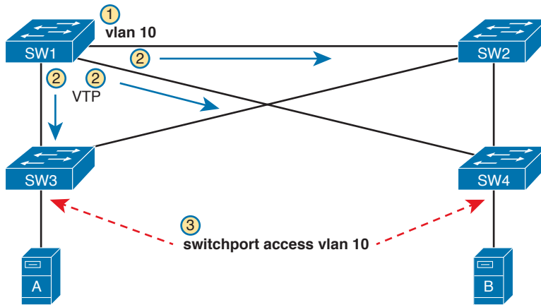
Figure 5-2 Distributing the vlan 10 Command with VTP
