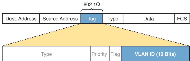
Figure 1-6 802.1Q Trunking
