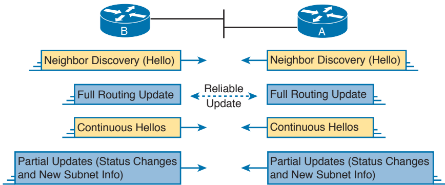
Figure 9-9 Full and Partial EIGRP Updates
