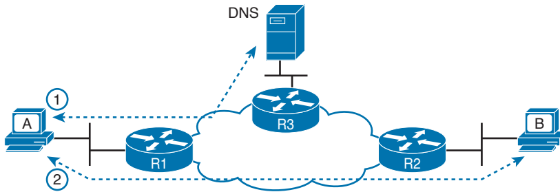
Figure J-10 DNS Name Resolution by Host A
