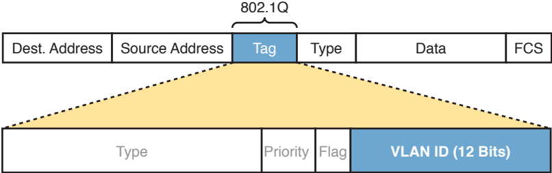
Figure 1-6 802.1Q Trunking
