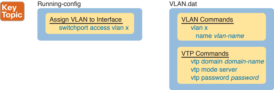
Figure 5-9 Where VTP Stores Configuration: VTP Client and Server
