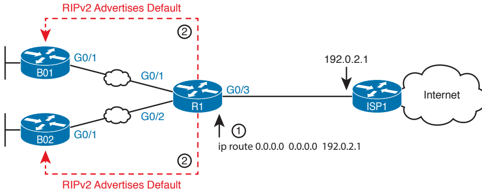
Figure G-16 A Scenario for RIPv2 to Advertise Default Routes
