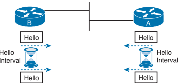
Figure 7-6 OSPF Hello Packets
