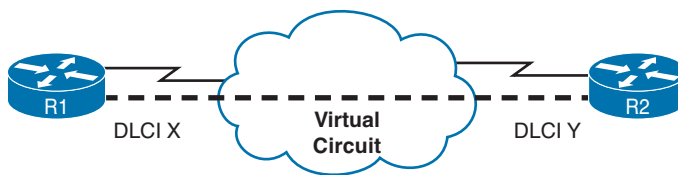
Figure H-2 Frame Relay PVC Concepts
