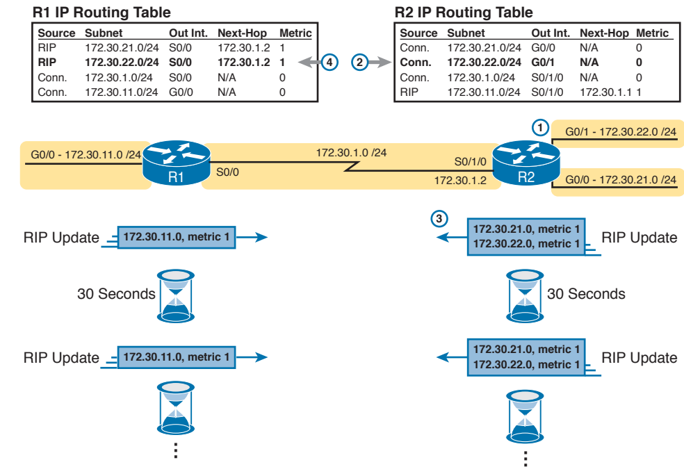
Figure 9-5 Normal Steady-State RIP Operations: Full Update with Split Horizon
