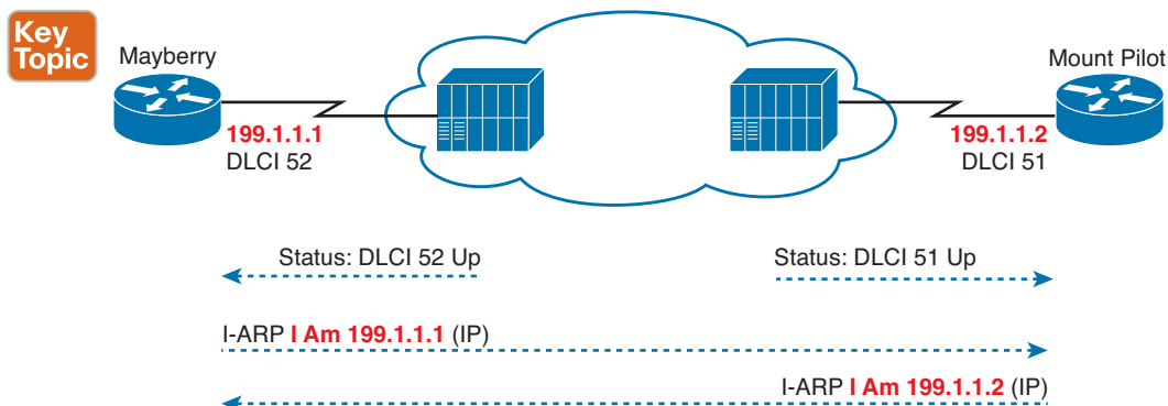
Figure I-4 Inverse ARP Process
