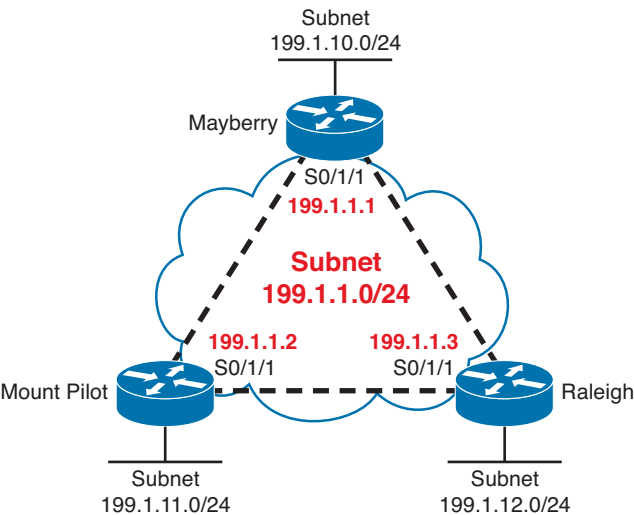
Figure H-11 Full Mesh with IP Addresses
