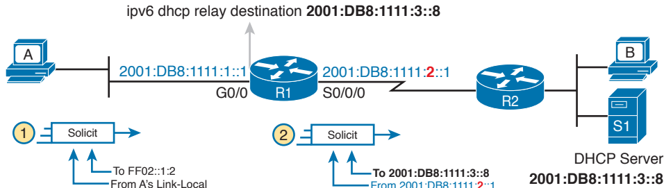
Figure 22-6 DHCPv6 Relay Agent and DHCP IPv6 Addresses
