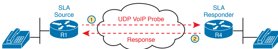
Figure 26-11 Using ICMP UDP Jitter Probes
