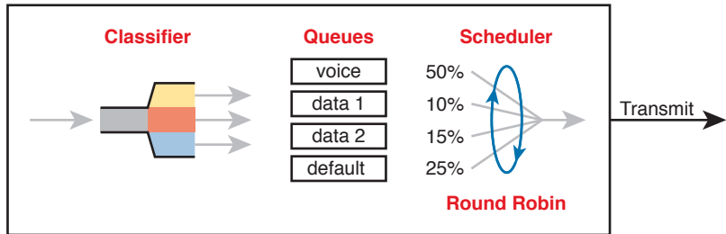
Figure 18-16 Round Robin Not Good for Voice Delay (Latency) and Jitter
