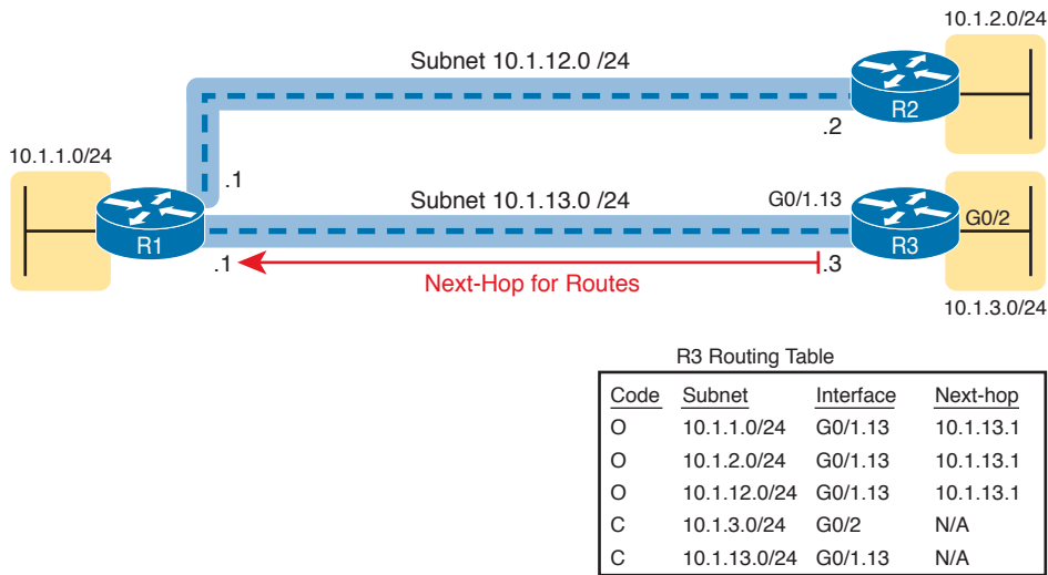
Figure 14-9 Layer 3 Forwarding Between Remote Sites—Through Central Site
