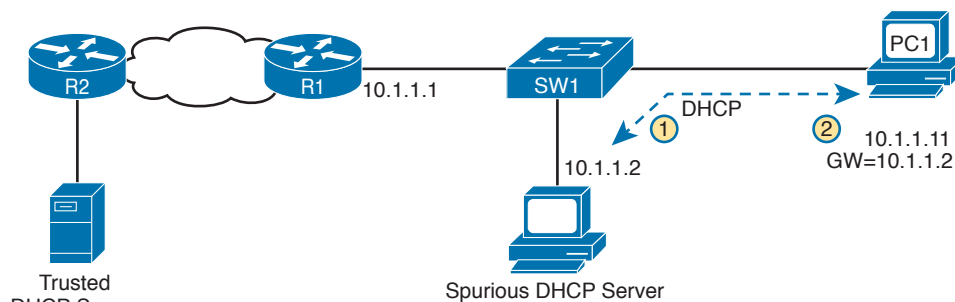
Figure 6-9 DHCP Attack Supplies Good IP Address but Wrong Default Gateway
