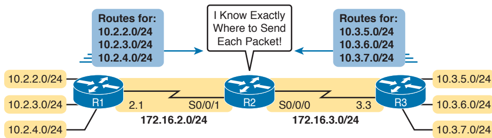
Figure G-14 The Effect of no auto-summary on the Network from Figure G-13
