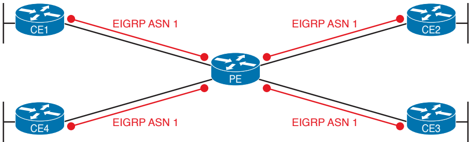
Figure 14-23 EIGRP Metrics Unaffected by MPLS VPN Internals
