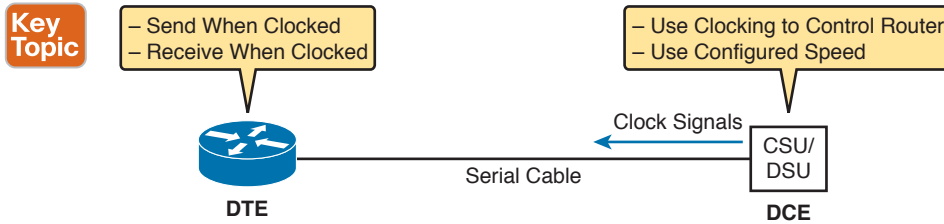
Figure 13-7 DCE and DTE Roles for a CSU/DSU and a Router Serial Interface
