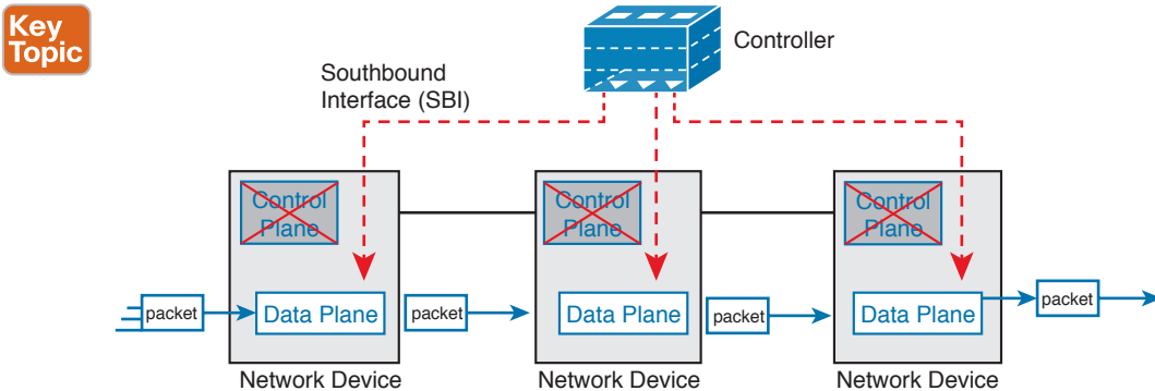
Figure 28-5 Centralized Control Plane and a Distributed Data Plane
