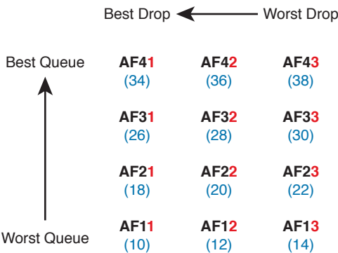
Figure 18-11 Differentiated Services Assured Forwarding Values and Meaning
