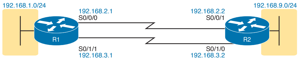
Figure 13-17 Multiple Parallel Serial Links Between Routers
