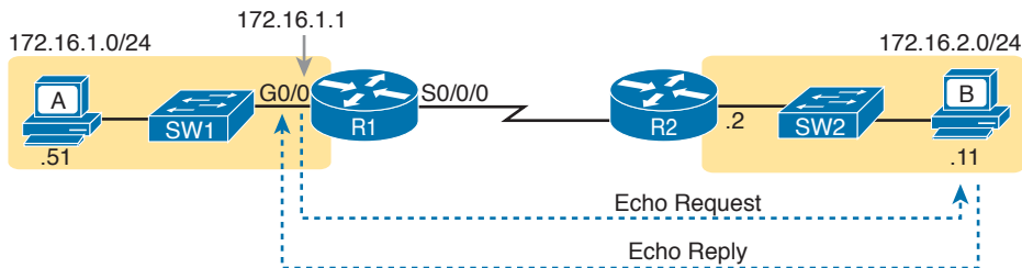
Figure 21-8 IP Helper Address Effect
