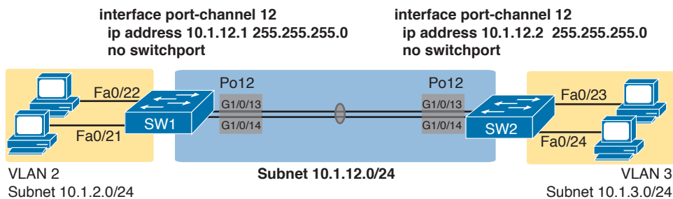
Figure 19-7 Design Used in EtherChannel Configuration Examples
