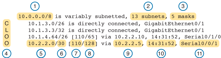
Figure 21-10 show ip route Command Output Reference
