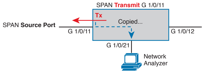
Figure 26-17 SPAN Construct: Source Port G1/0/11, for Frames in the Transmit Direction
