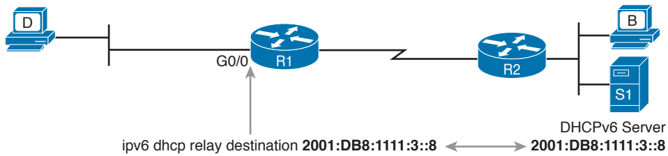
Figure 22-16 IPv6 DHCP Relay
