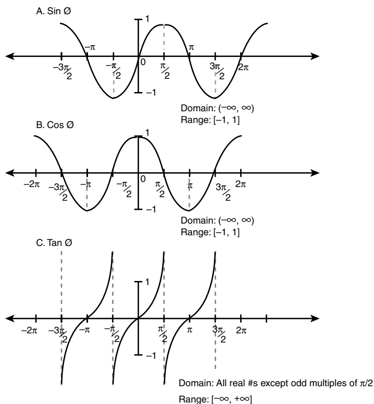
Figure C.2 Graphs of basic trigonometric functions.
