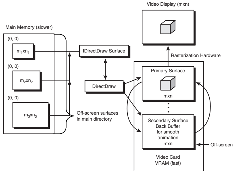
Figure 6.2 DirectDraw surfaces.
