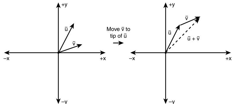
Figure C.6 Vector addition.
