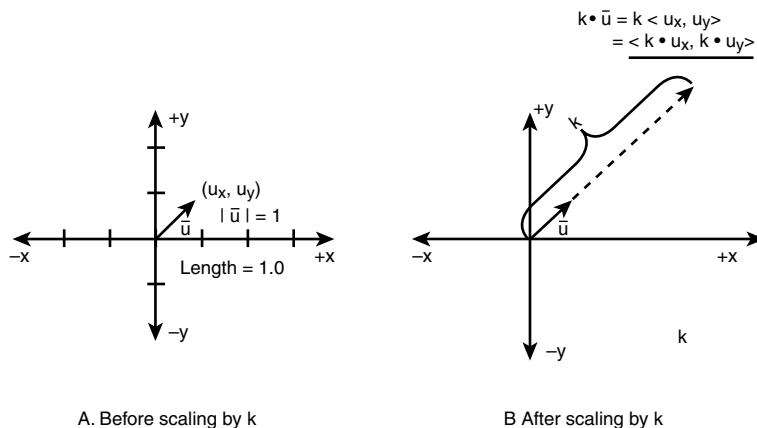
Figure C.4 Vector scaling.
