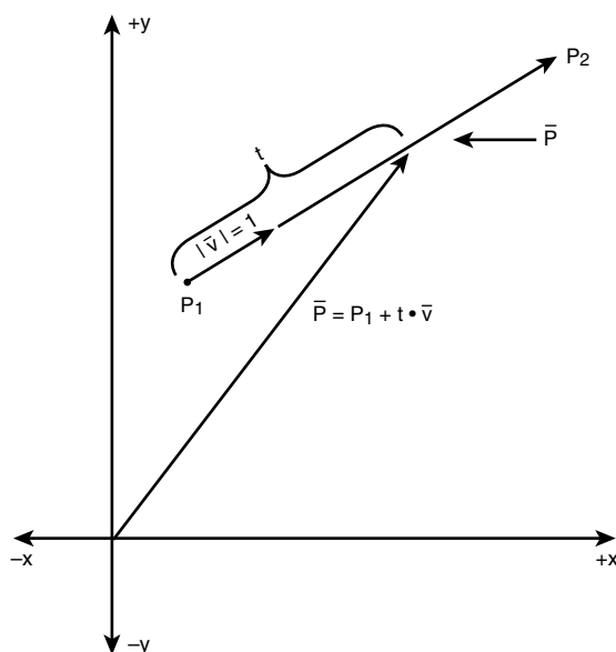
Figure C.11 Position vectors.
