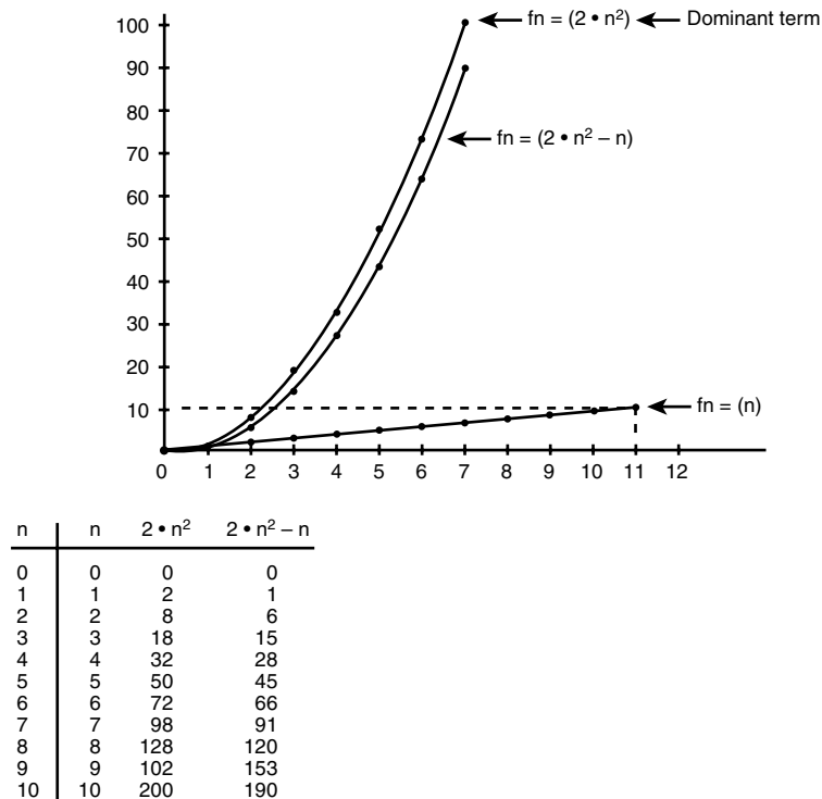
Figure 11.5 Rates of growth for the term of 2 \cdot n^2 - n .
