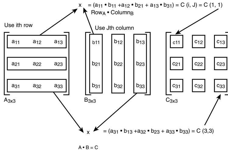
Figure 8.25 The mechanics of matrix multiplication.
