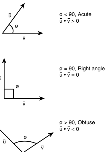
Figure C.9 Angles and their relationships to the dot product.
