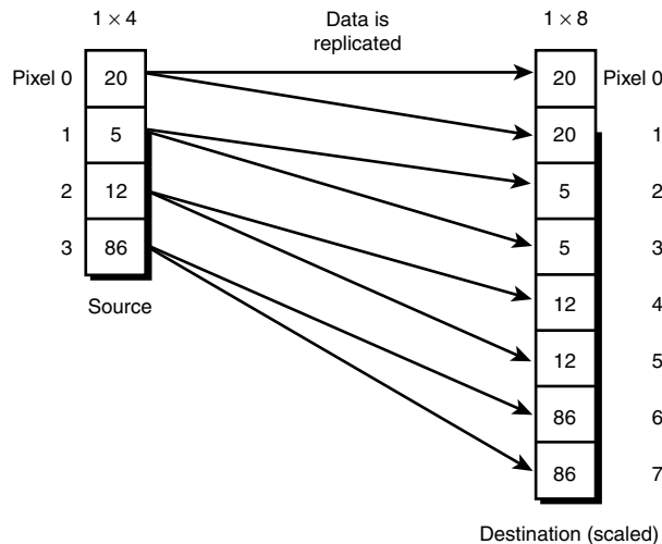
Figure 7.34 Scaling a 1 \times 4 -pixel bitmap to 1 \times 8 pixels.
