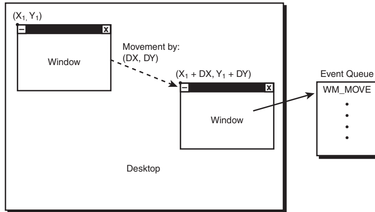
Figure 3.21 Generation of the WM_MOVE message.
