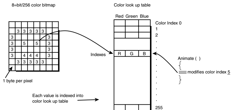
Figure 7.36 Color animation using palette indirection.
