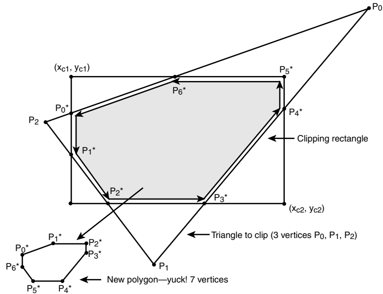
Figure 8.33 Worst-case scenario when clipping a triangle.
