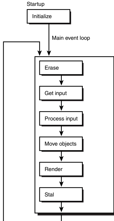
Figure 13.44 The game loop you've learned to love.
