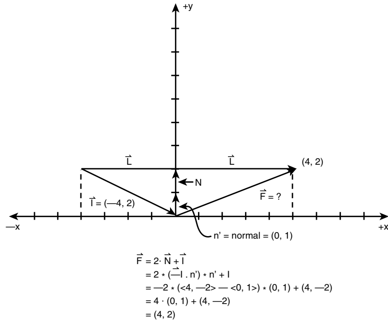
Figure 13.26 A numerical example of vector reflection.
