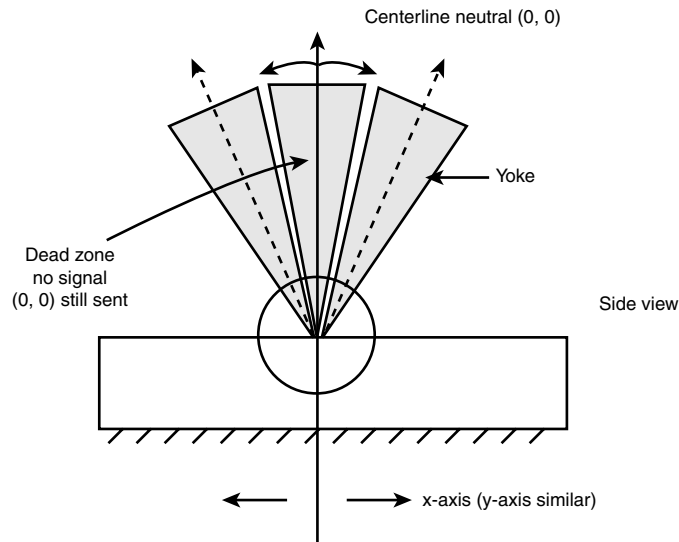
Figure 9.12 The mechanics of the joystick dead zone.
