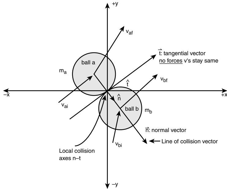
Figure 13.33 The central impact of two masses problem.
