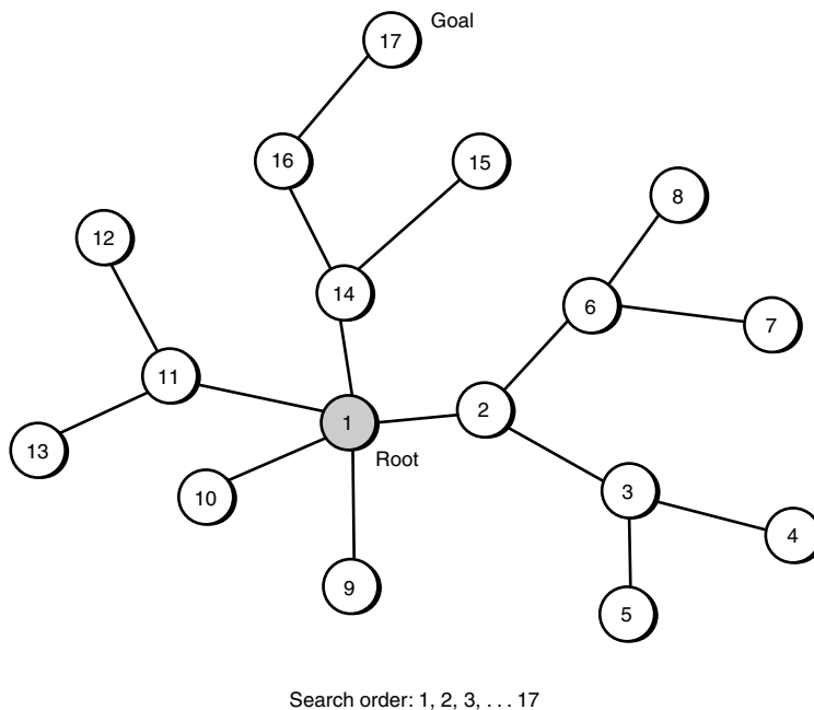
Figure 12.27 Depth-first search in action.
