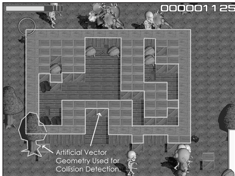
Figure 8.53 A polygon collision geometry overlaid on a fake rendered image.
