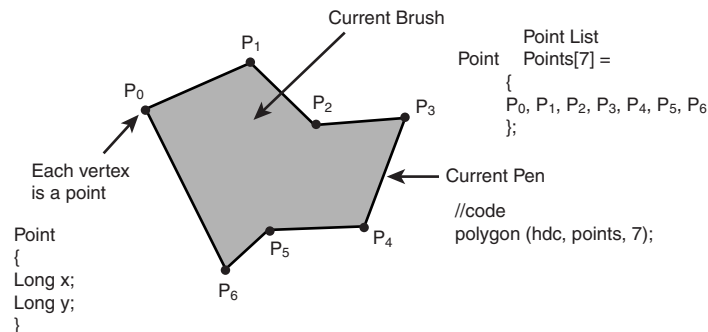
Figure 4.8 Using the Polygon() function.
