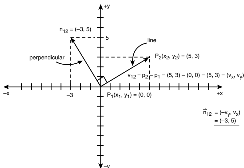
Figure 13.25 Computing the per- pendicular to a line.
