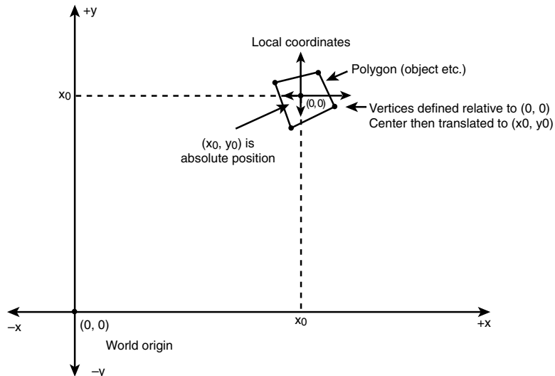
Figure 8.15 Local coordinates in relation to world coordinates.
