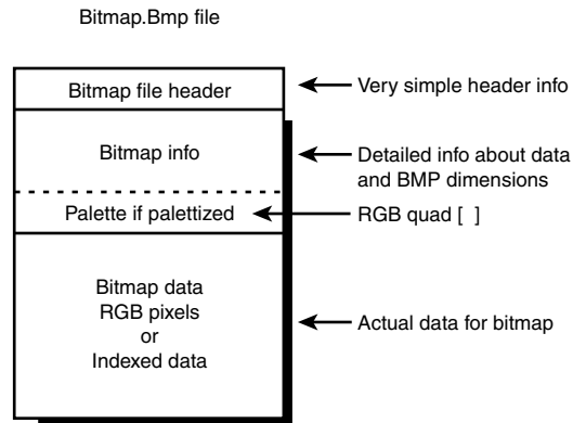
Figure 7.23 The structure of a .BMP file on disk.
