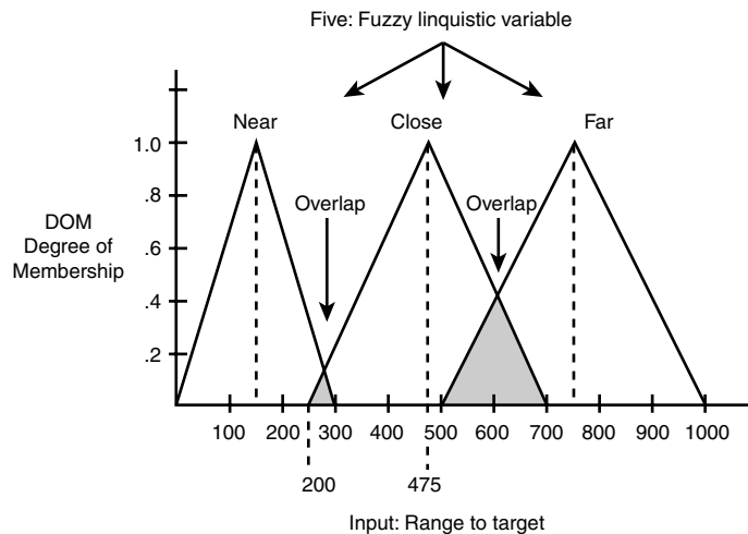
Figure 12.37 A fuzzy manifold composed of range FLVs.
