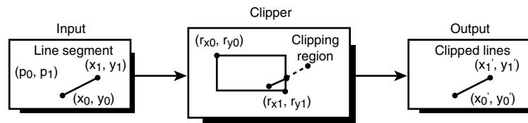
Figure 8.9 The clipping process diagrammed.
