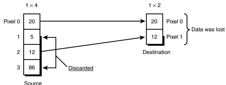
Figure 7.35 Scaling a 1 \times 4 -pixel bitmap to 1 \times 2 pixels.
