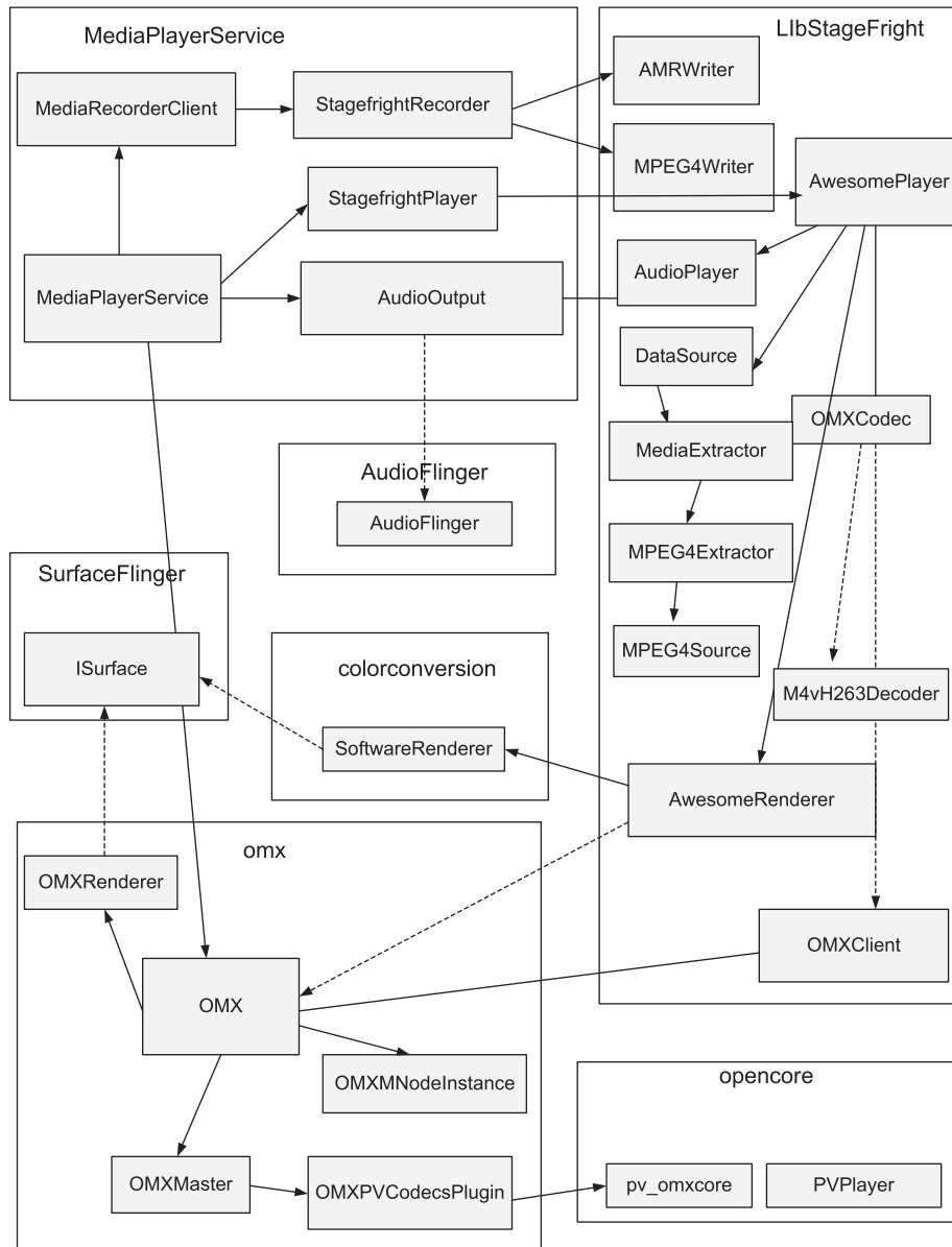
Figure 10.1 Stagefright services
