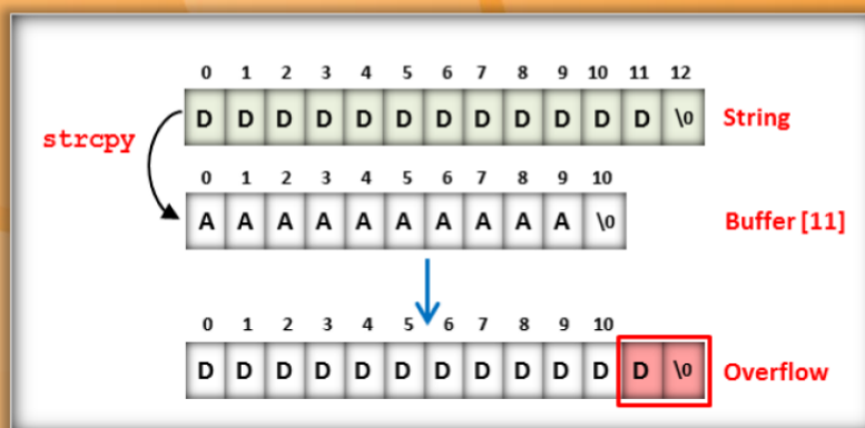
FIGURE 18.1: Buffer Overflows
