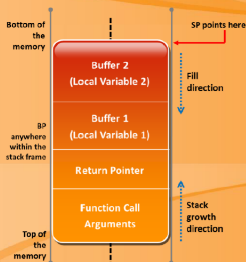
FIGURE 18.2: Stack Segment
