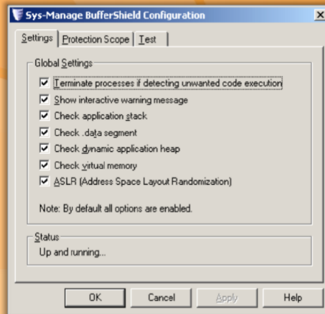
FIGURE 18.16: BufferShield Screenshot
