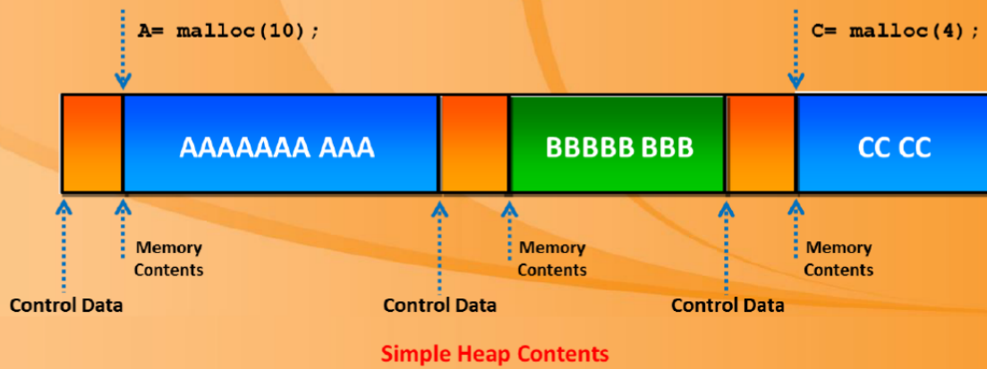
FIGURE 18.4: Understanding Heap
