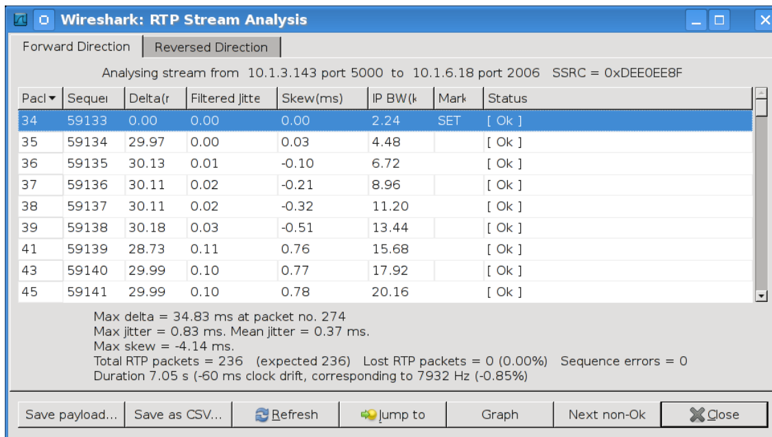
Figure 84. The “RTP Stream Analysis” window
