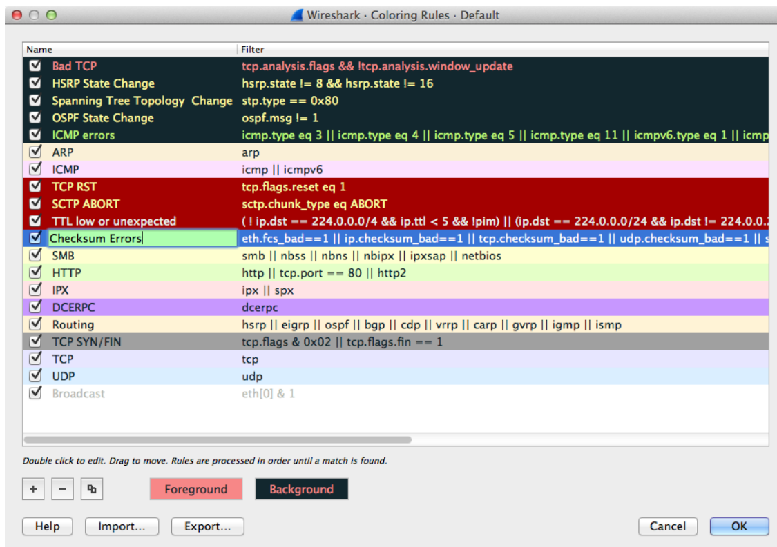
Figure 86. The “Coloring Rules” dialog box
