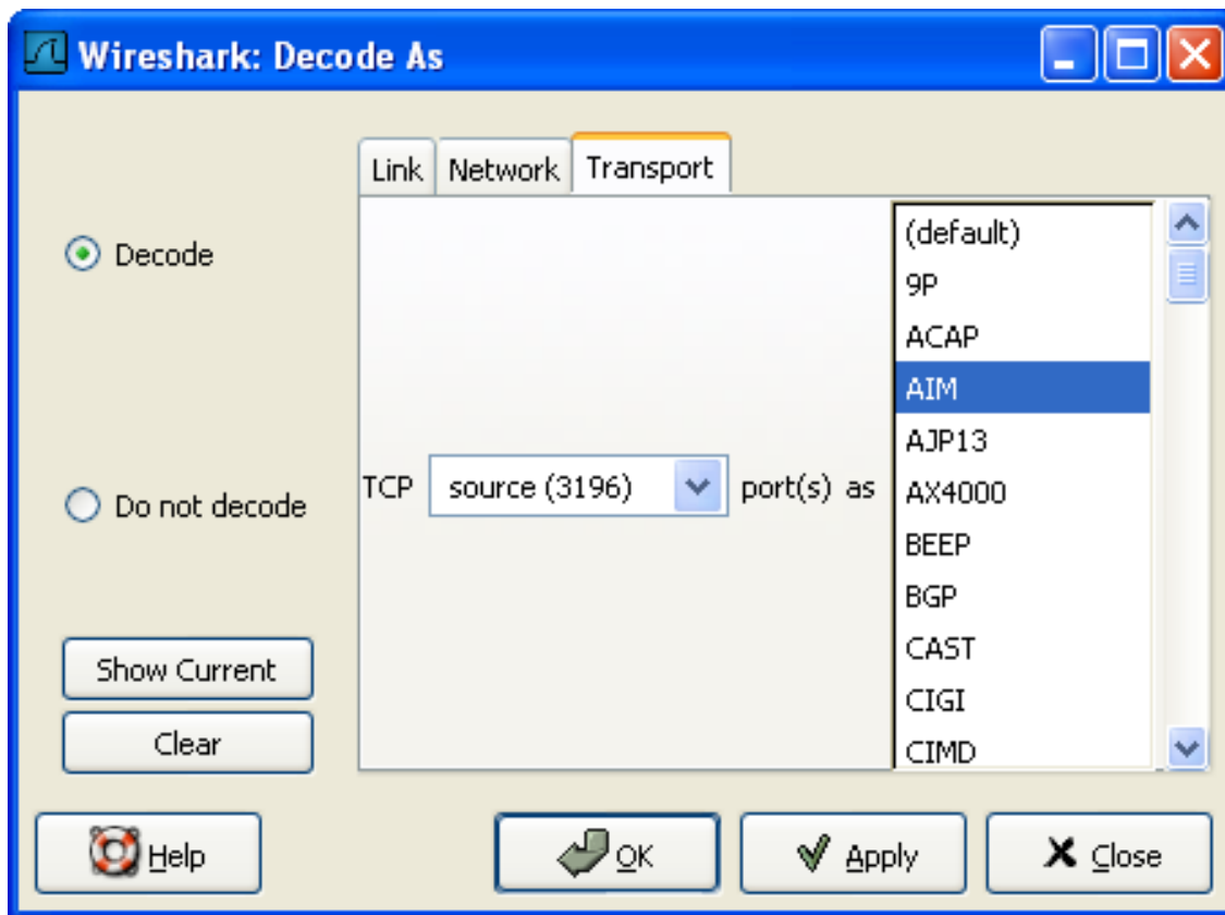
Figure 90. The “Decode As” dialog box
