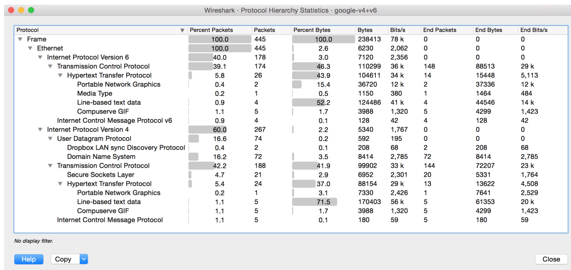
Figure 75. The “Protocol Hierarchy” Window
