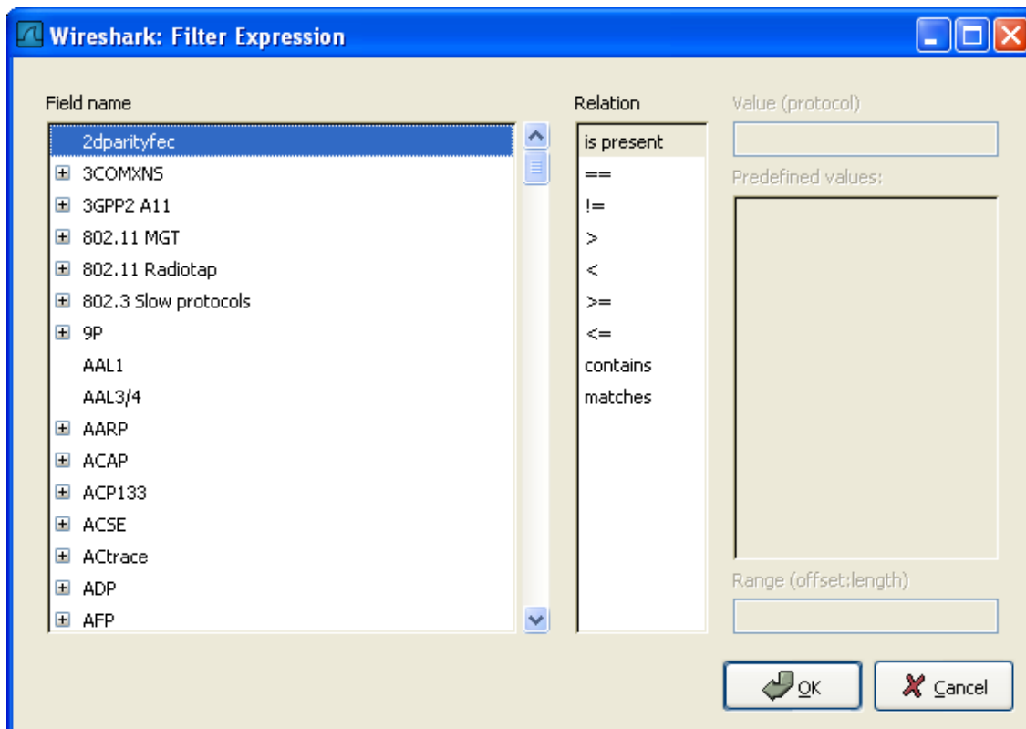
Figure 63. The “Filter Expression” dialog box
