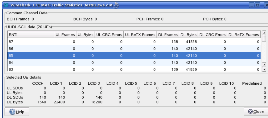
Figure 82. The “LTE MAC Traffic Statistics” window
