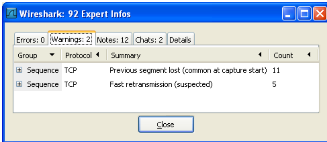
Figure 69. The “Expert Info” dialog box
