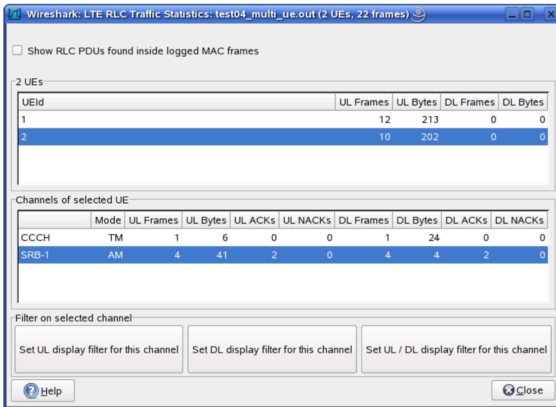
Figure 83. The “LTE RLC Traffic Statistics” window
