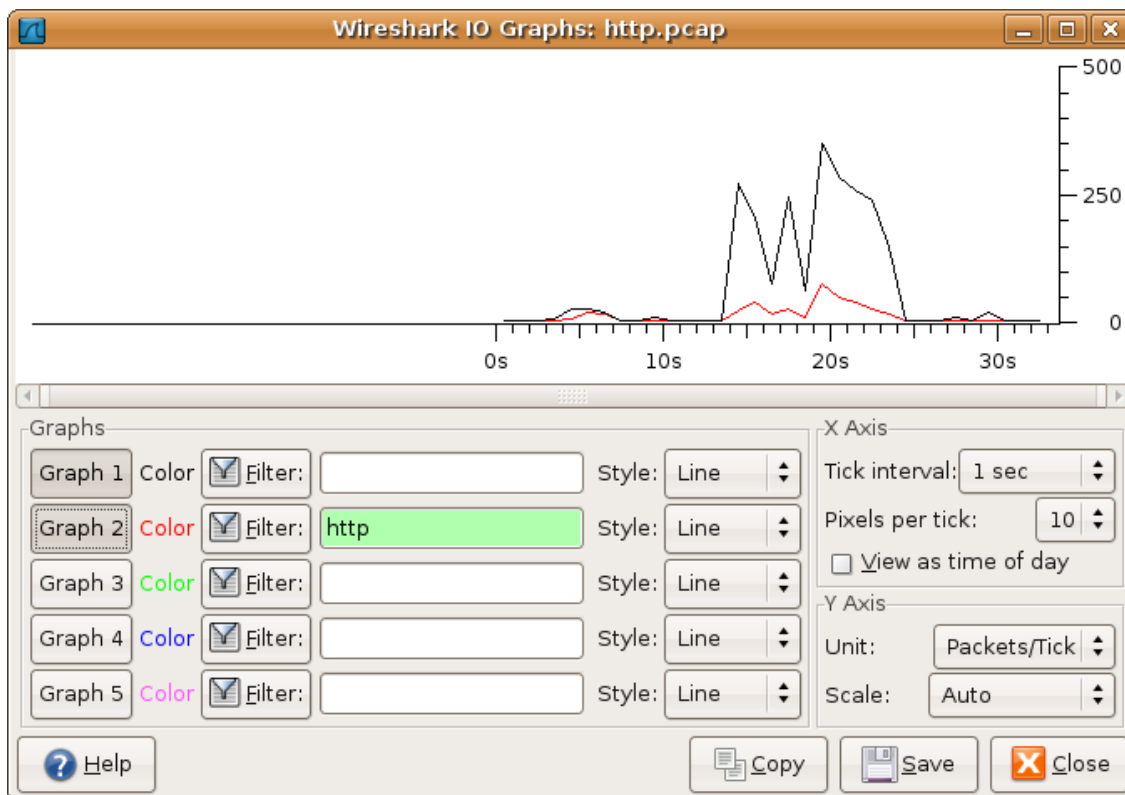
Figure 78. The “I/O Graphs” window
