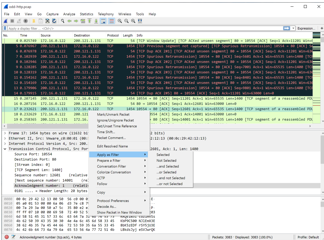
Figure 59. Pop-up menu of the “Packet List” pane
