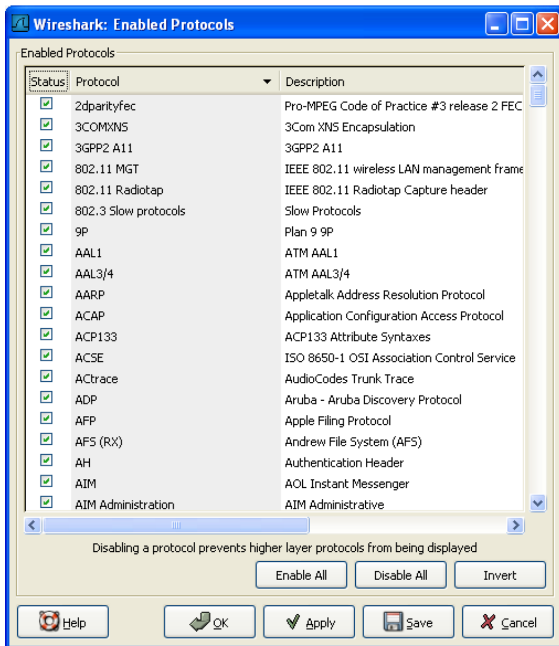
Figure 89. The “Enabled Protocols” dialog box
