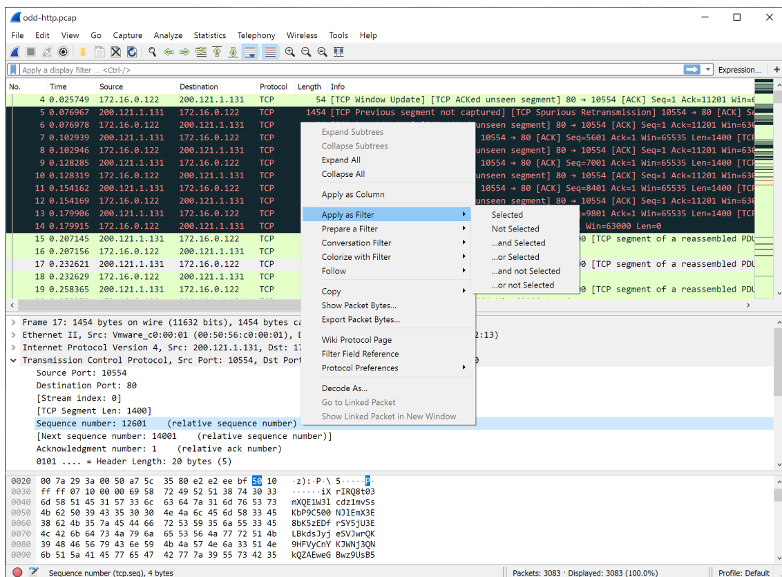
Figure 60. Pop-up menu of the “Packet Details” pane
