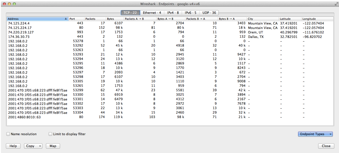
Figure 77. The “Endpoints” window
