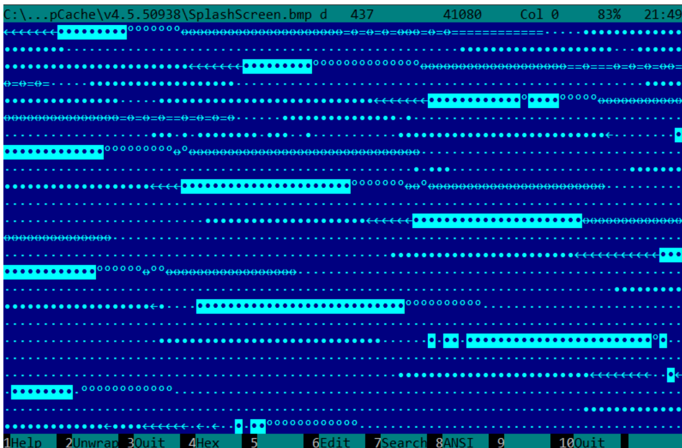
Figure 5.15: BMP file fragment
