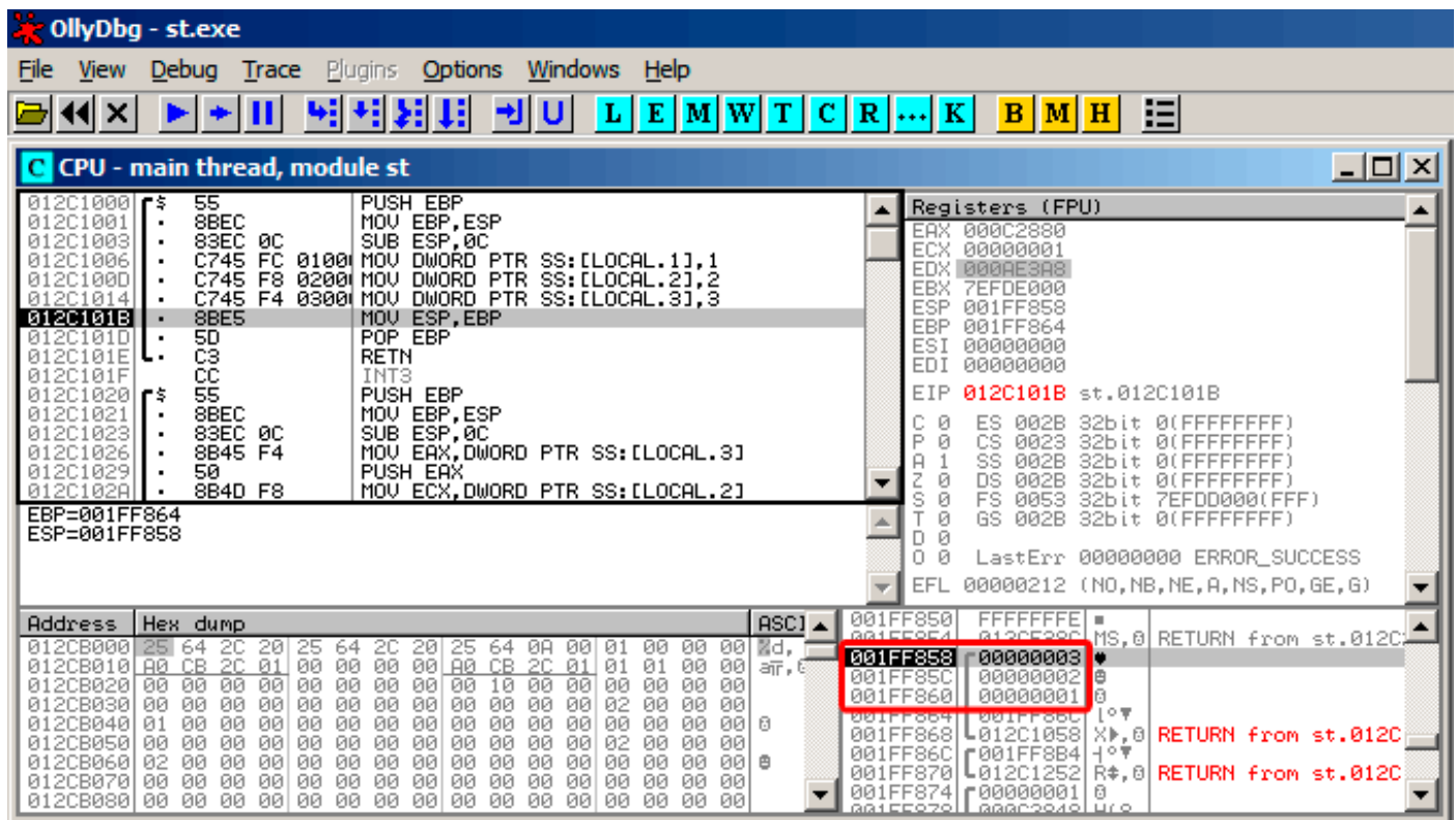
Figure 1.6: OllyDbg: f1()
