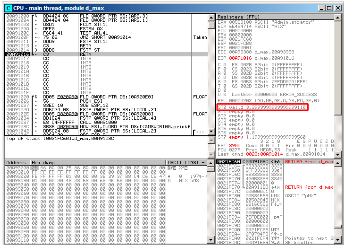
Figure 1.82: OllyDbg: FSTP is executed
