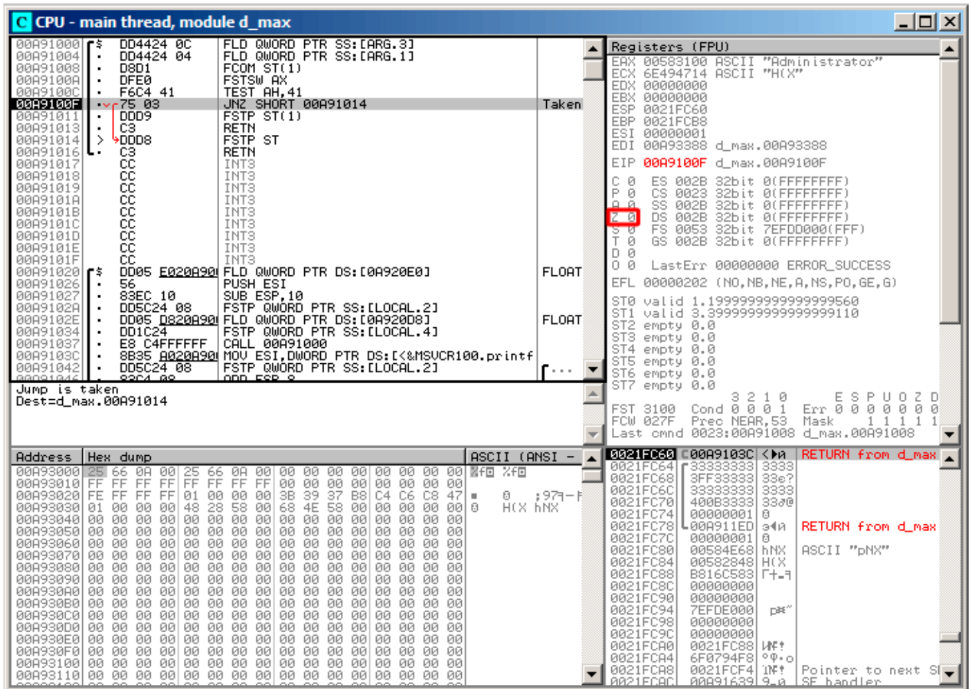
Figure 1.81: OllyDbg: TEST is executed
