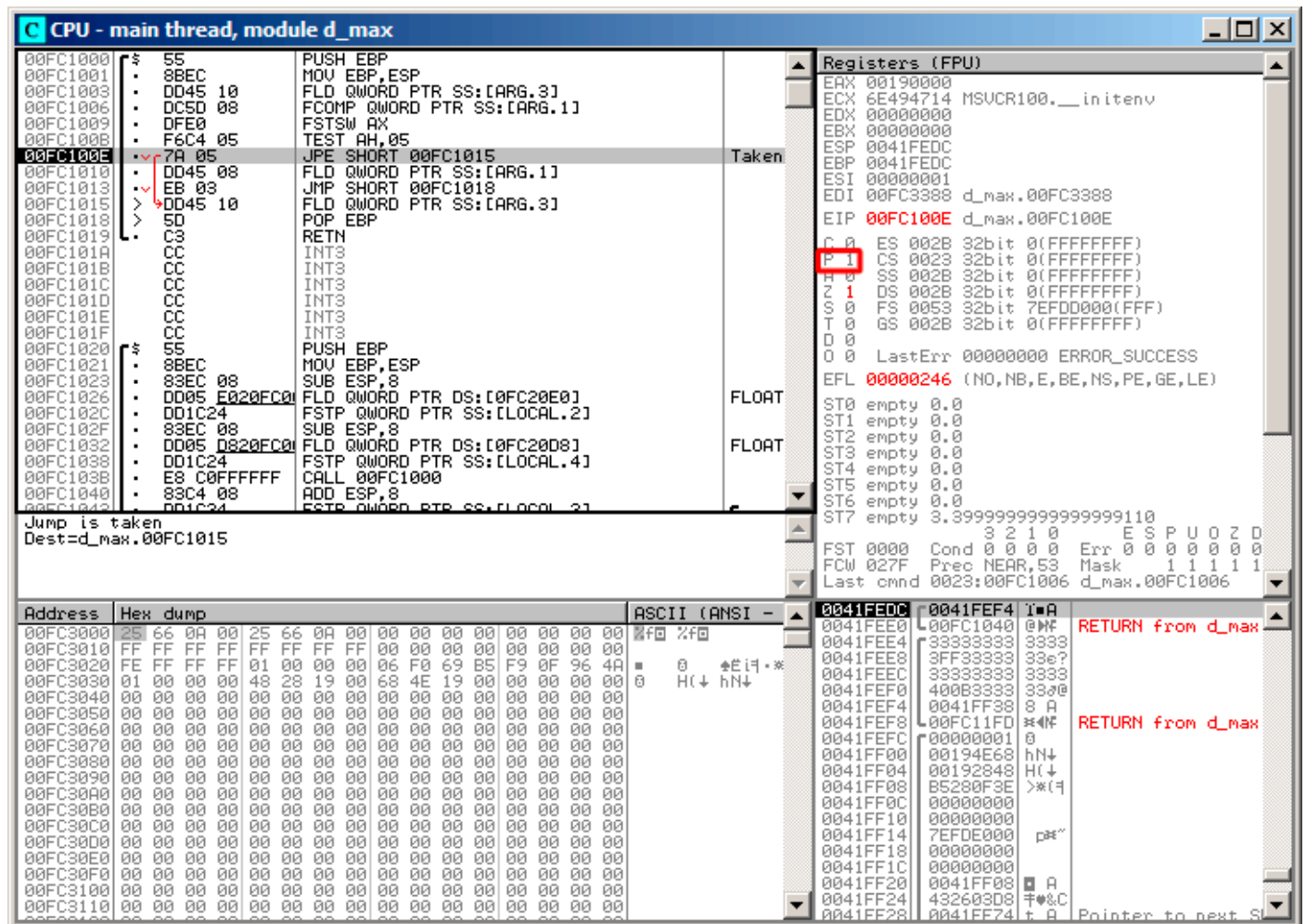
Figure 1.71: OllyDbg: TEST has been executed
