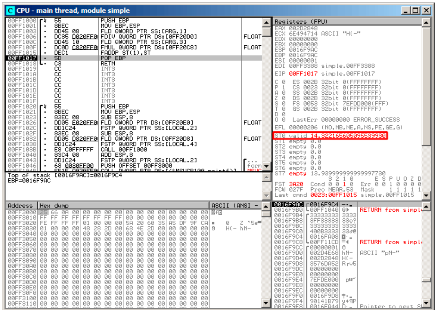
Figure 1.67: OllyDbg: FADDP has been executed
