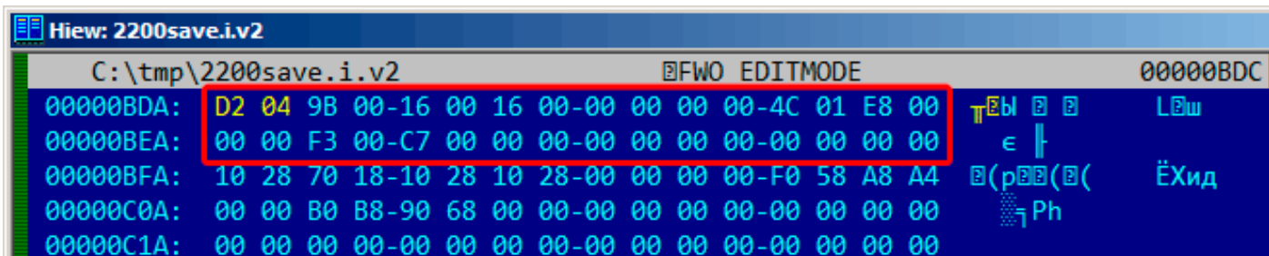
Figure 9.17: Hiew: let's write 1234 (0x4D2) there
