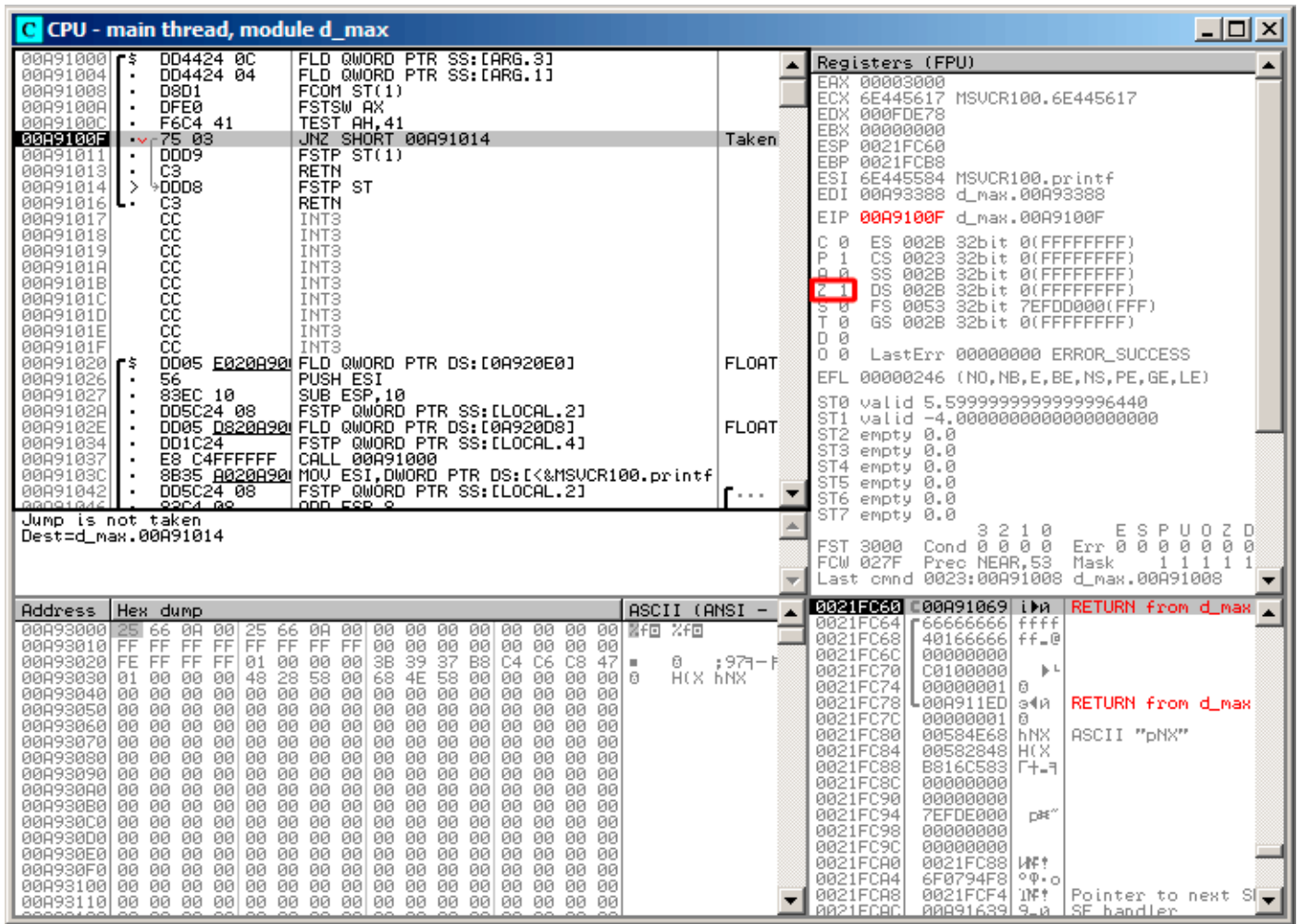
Figure 1.86: OllyDbg: TEST has been executed
