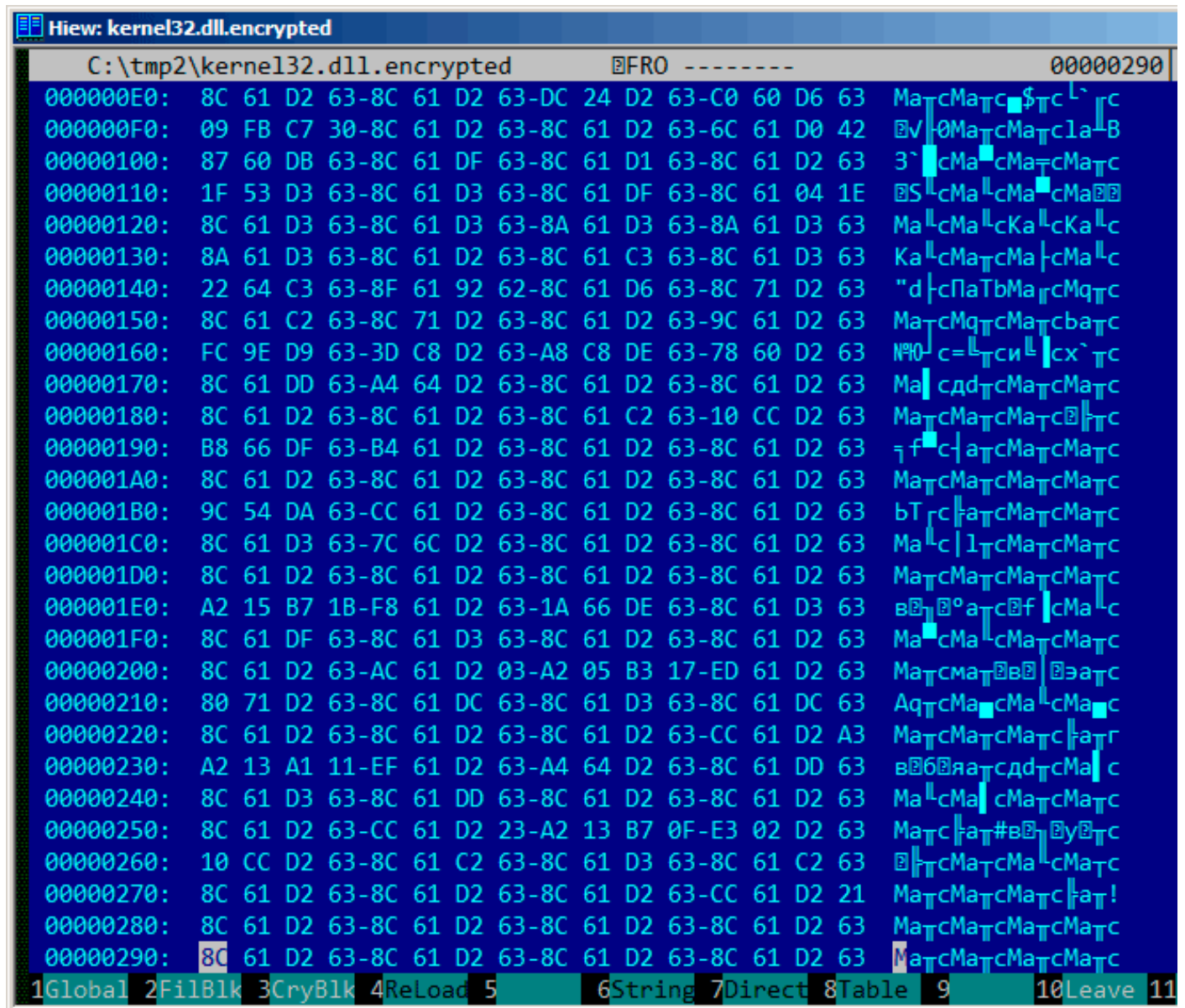
Figure 9.7: “Encrypted” PE-header
