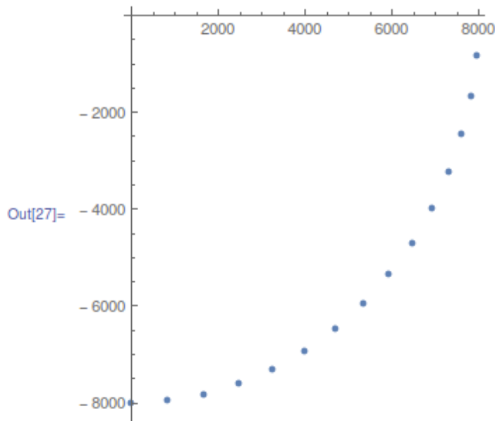
Figure 8.12: Mathematica
