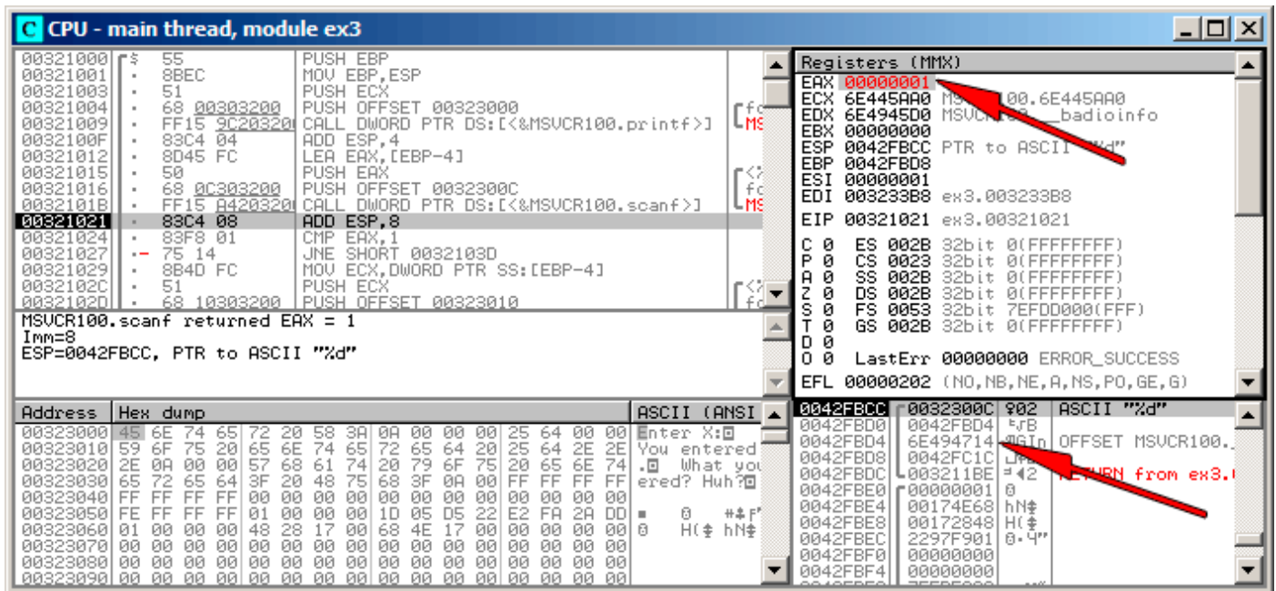
Figure 1.21: OllyDbg: scanf() returning error
