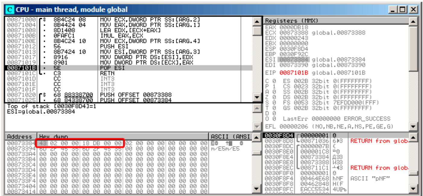
Figure 1.28: OllyDbg: f1() execution completed
