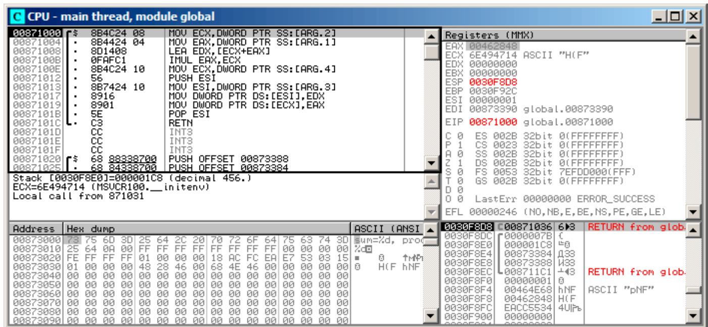
Figure 1.27: OllyDbg: f1() starts
