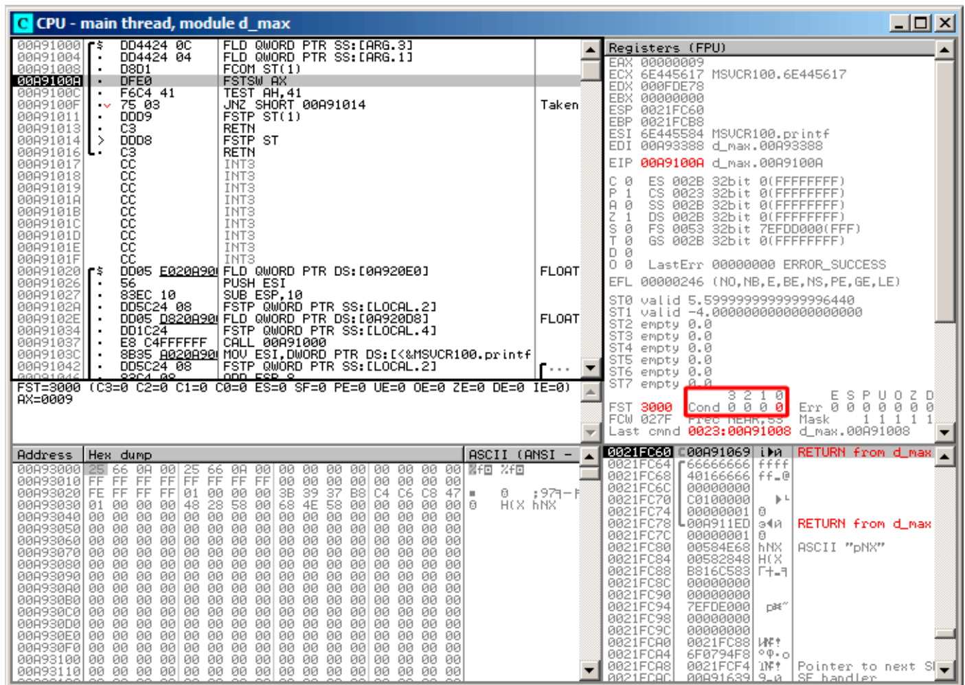
Figure 1.84: OllyDbg: FCOM is finished
