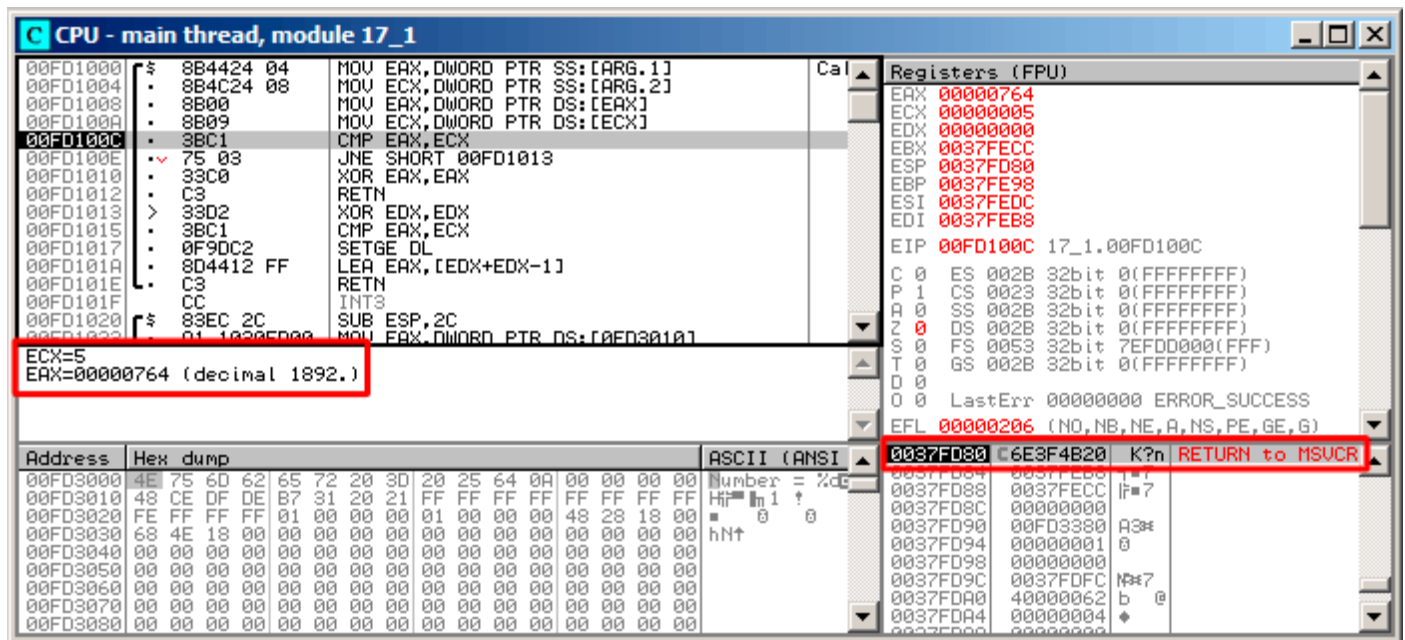
Figure 1.110: OllyDbg: first call of comp()
