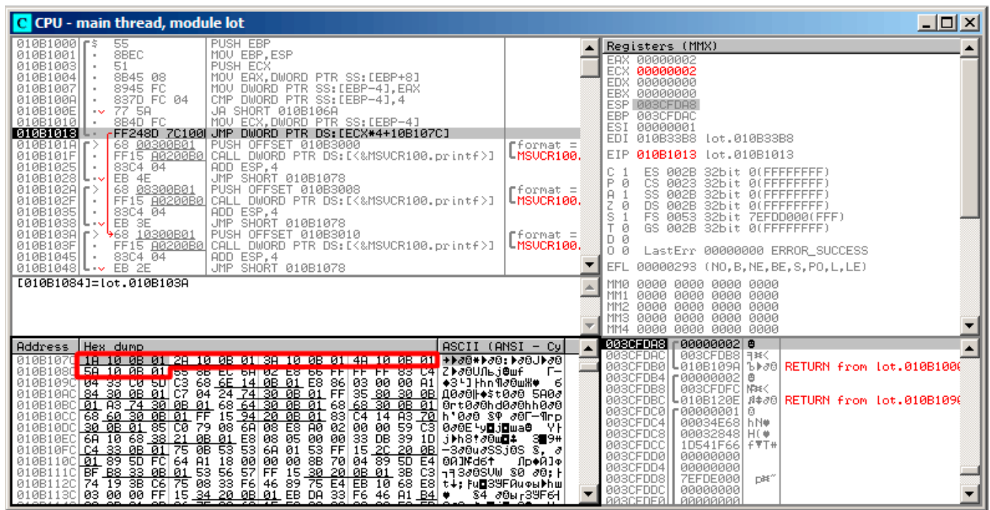
Figure 1.53: OllyDbg: calculating destination address using jumptable
