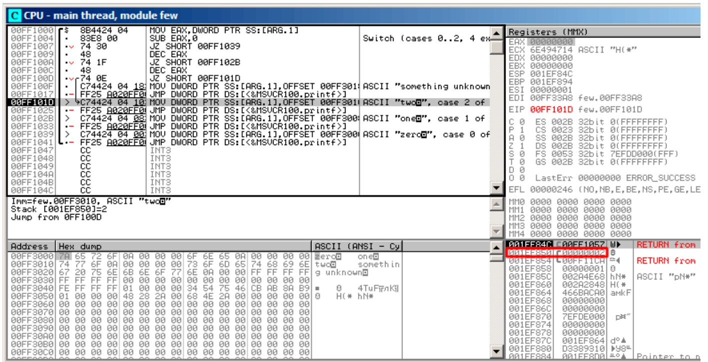
Figure 1.47: OllyDbg: pointer to the string is to be written at the place of the first argument
