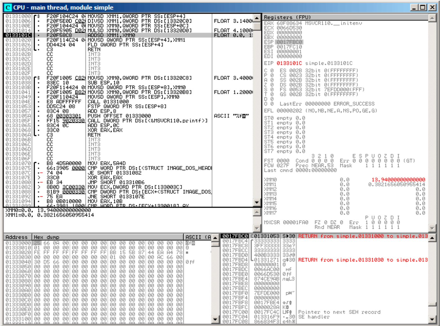
Figure 1.116: OllyDbg: MULSD calculated product and stored it in XMM0
