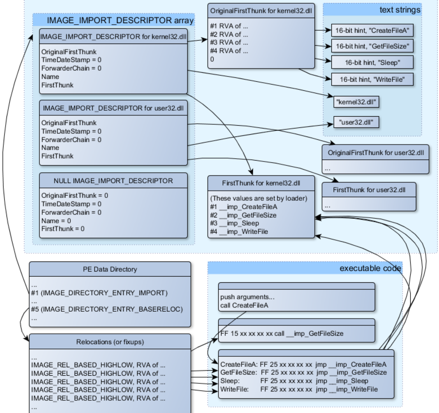
Figure 6.1: A scheme that unites all PE-file structures related to imports
