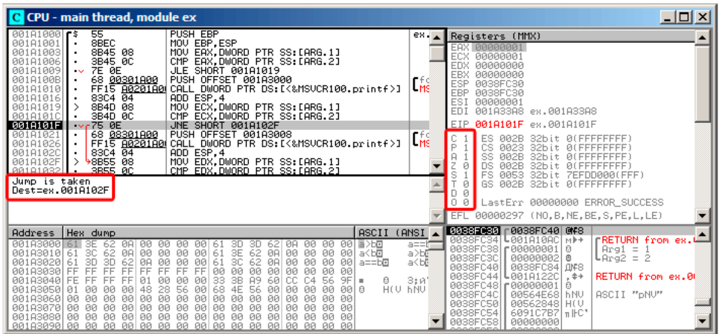
Figure 1.39: OllyDbg: f_signed(): second conditional jump
