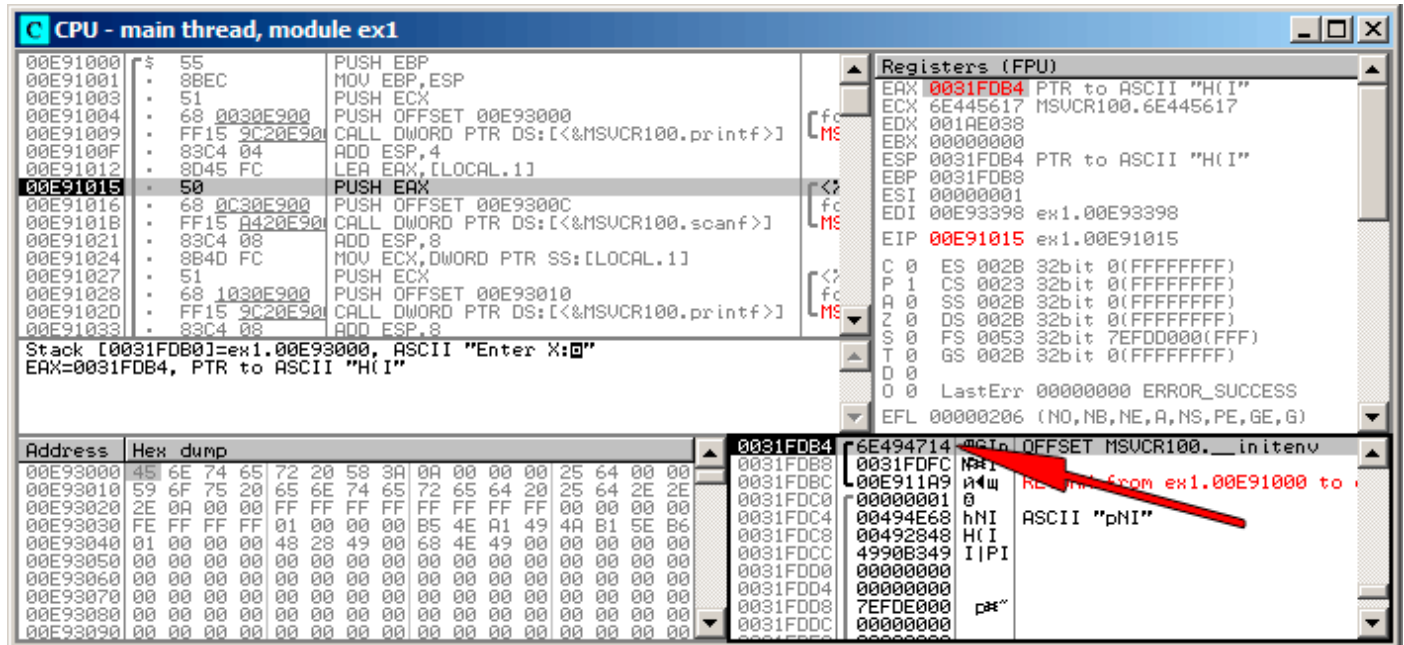
Figure 1.13: OllyDbg: The address of the local variable is calculated
