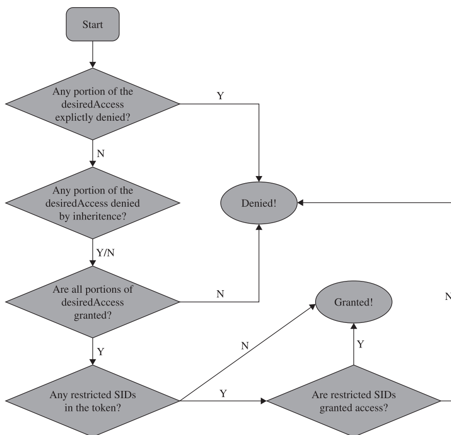
Figure 14-7 AccessCheck flowchart
