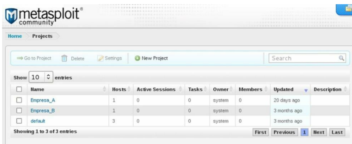
Figura 108 - Metasploit Community
