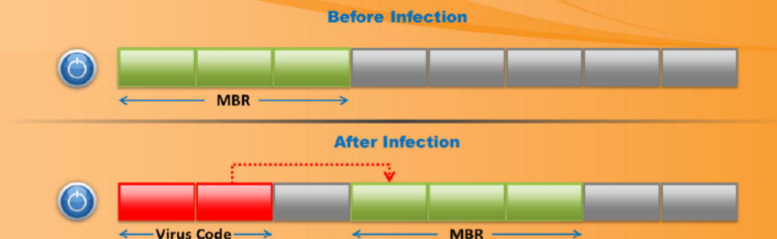
FIGURE 7.6: System or Boot Sector Viruses
