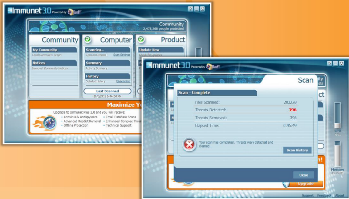
FIGURE 7.33: ImmuneT Screenshot
