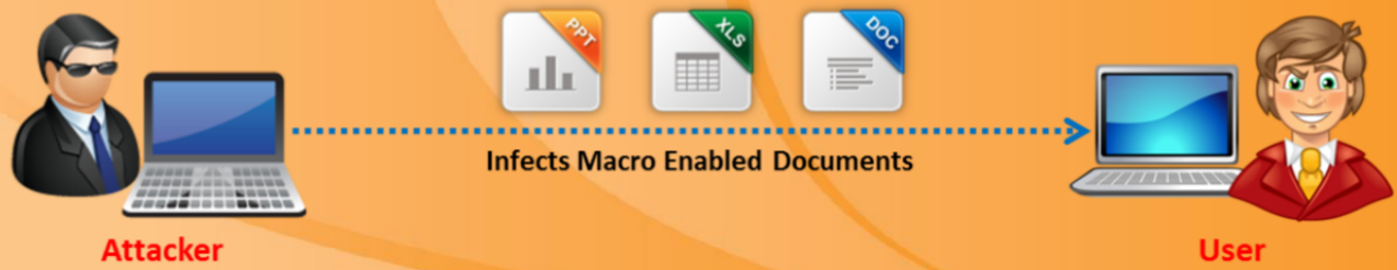
FIGURE 7.8: Macro Viruses
