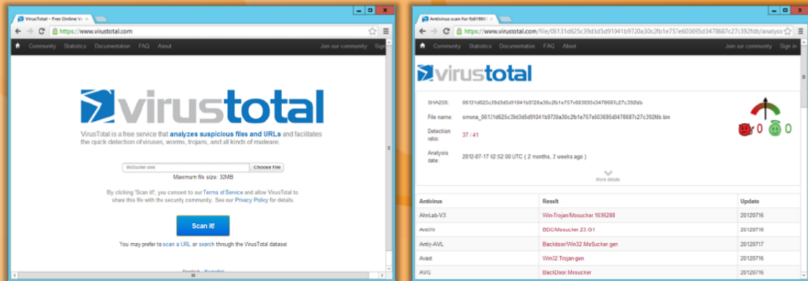
FIGURE 7.32: virustotal Screenshot
