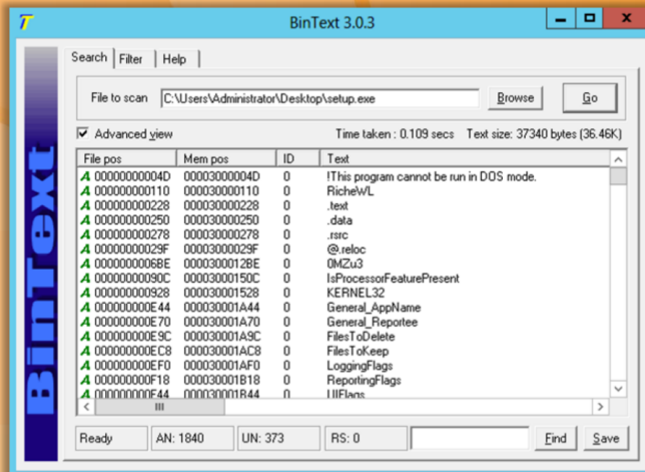
FIGURE 7.26: Bintext Screenshot
