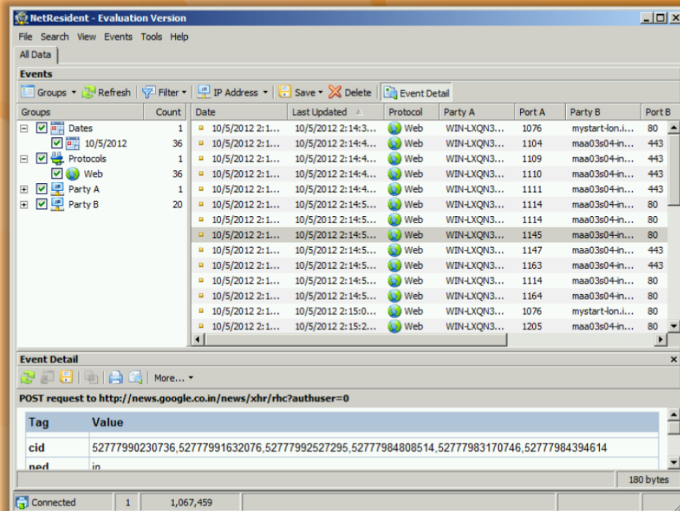
FIGURE 7.29: NetResident Screenshot
