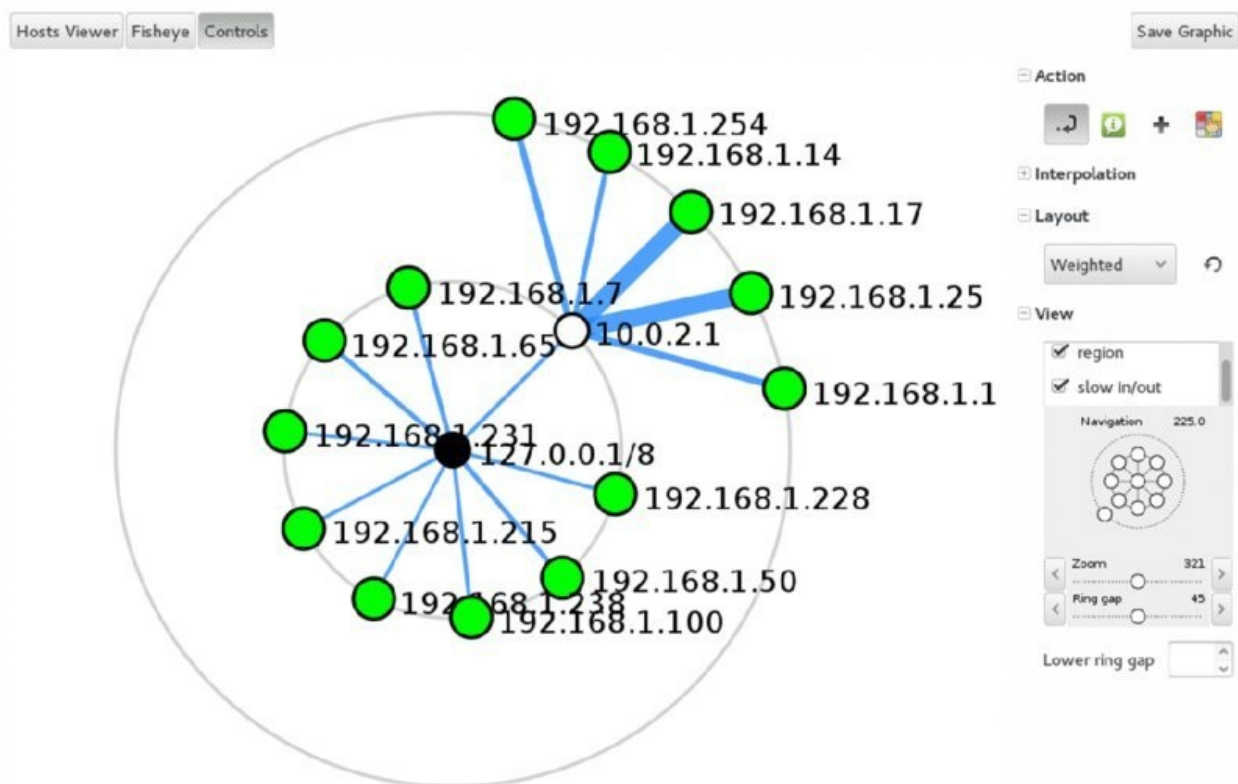
Figure 2.1 Zenmap topology view
