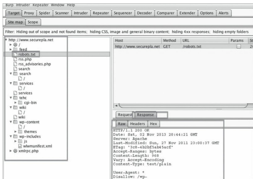
Figure 20 - Site Map/Request and Responses
