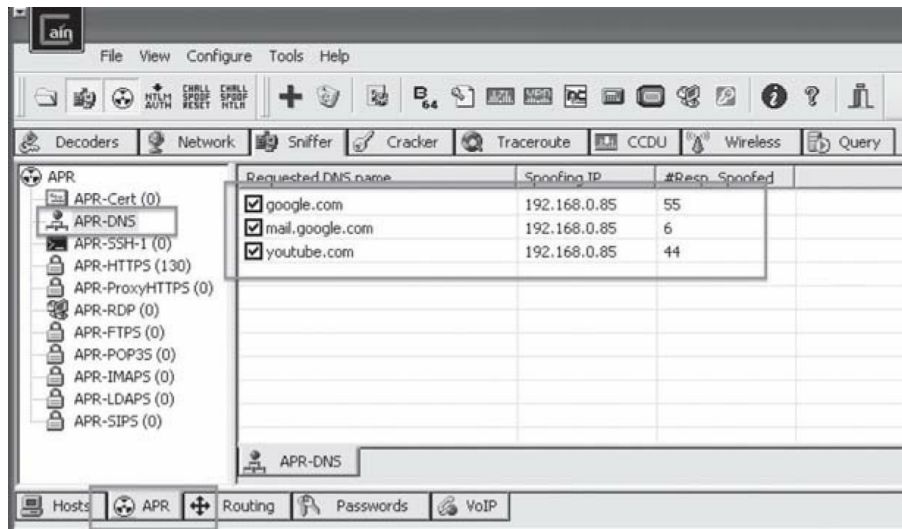
Figure 95 - Cain and Abel APR-DNS
