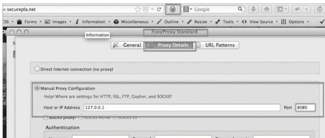
Figure 15 - Configuring the Brower's Proxy Settings
