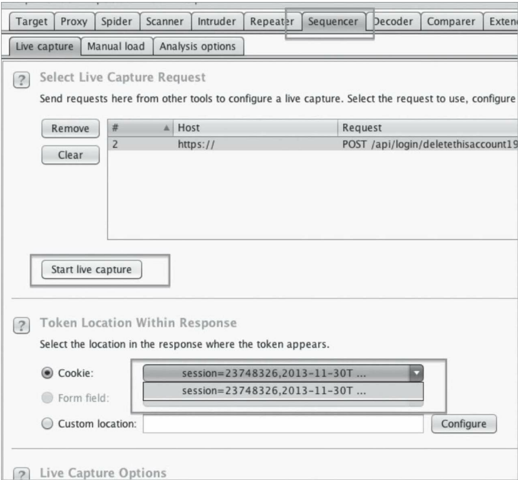
Figure 52 - Selecting the Session Token
