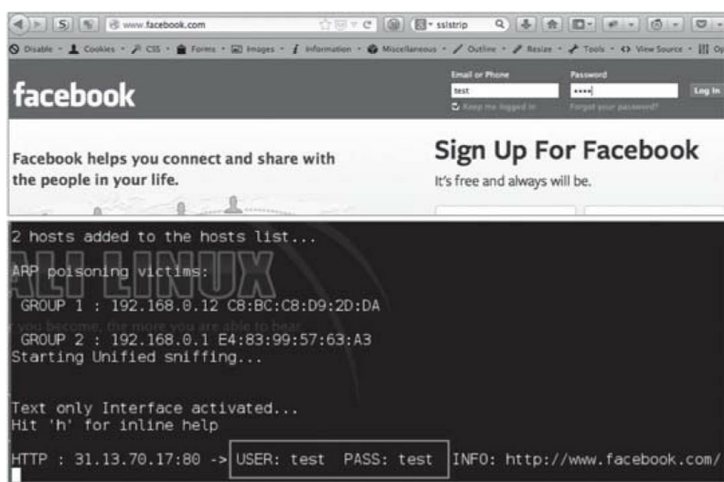
Figure 99 - Victim Visiting Facebook.com and Redirected to HTTP and Captured Passwords
