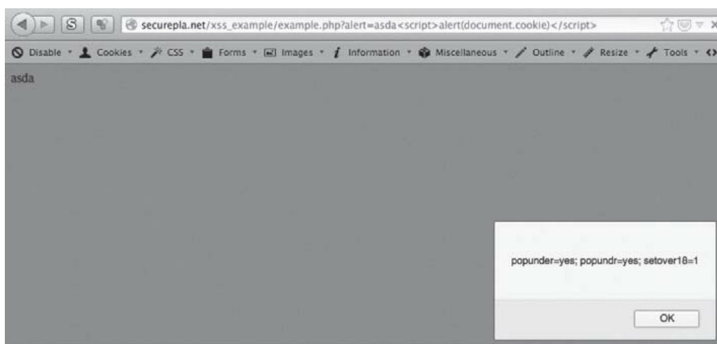
Figure 40 - Example XSS Finding
