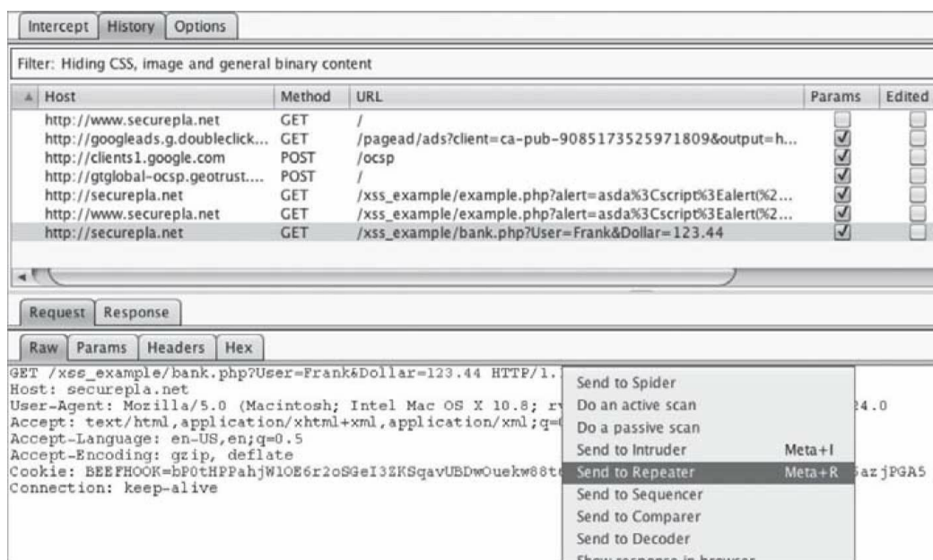
Figure 48 - Sending to Burp's Repeater
