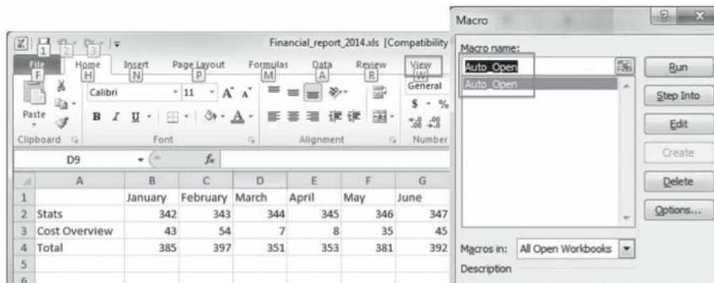
Figure 110 - Excel Example with PowerShell Reverse Shell
