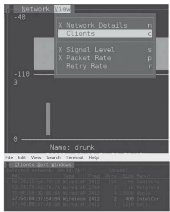
Figure 117 - Finding Clients Connected to an AP
