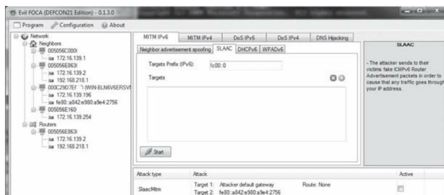
Figure 90 - Evil FOCA SLAAC
