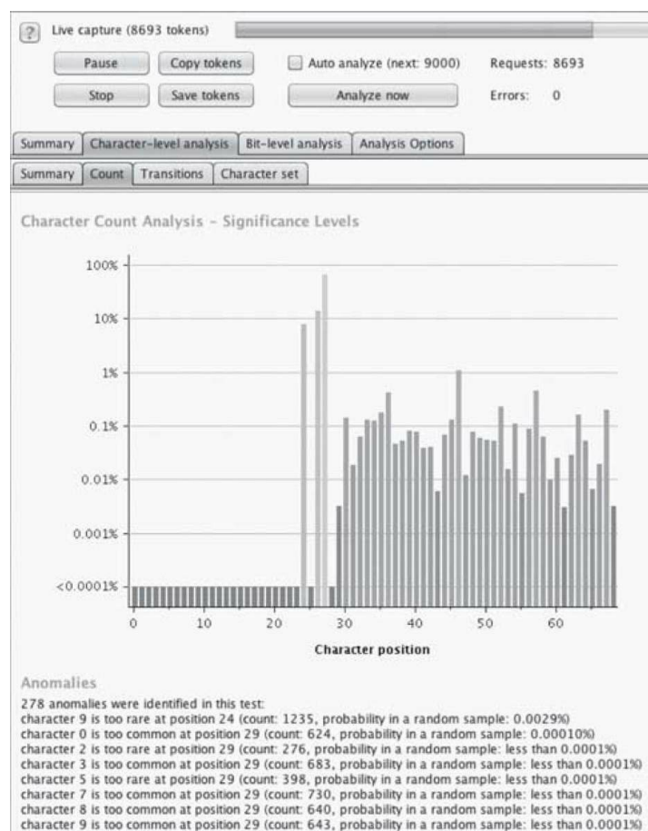
Figure 53 - Character Position for Cookies
