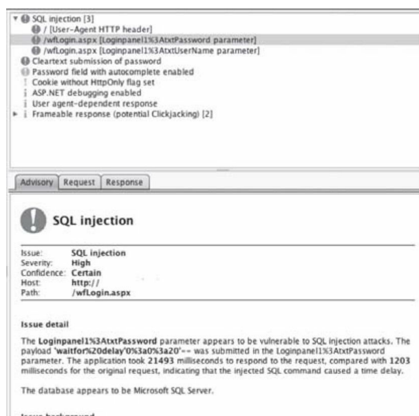
Figure 30 - Burp SQL Injection Finding
