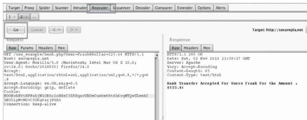
Figure 49 - Executing Burp Repeater
