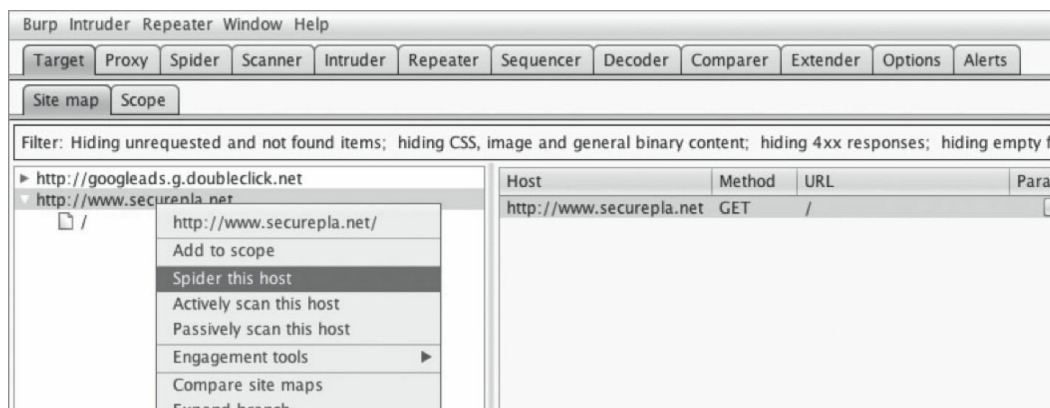
Figure 19 - Spidering the Host
