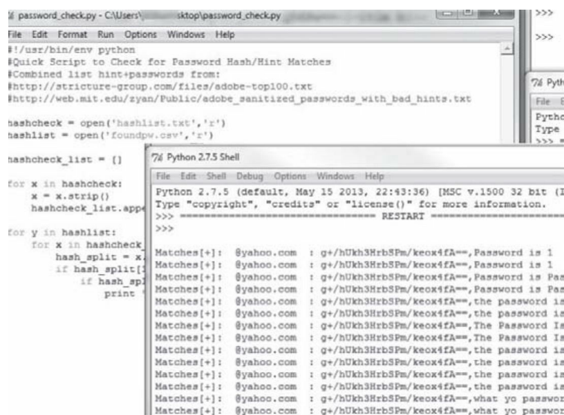
Figure 7 - Custom Python Script to Look for Email/Passwords
