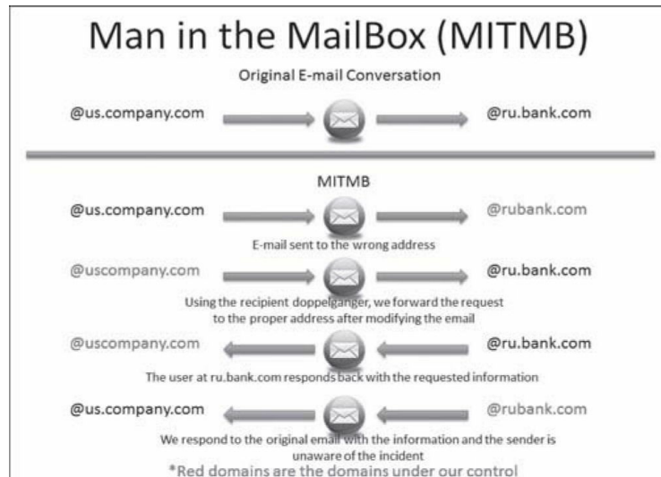
Figure 100 - Man in the MailBox Example
