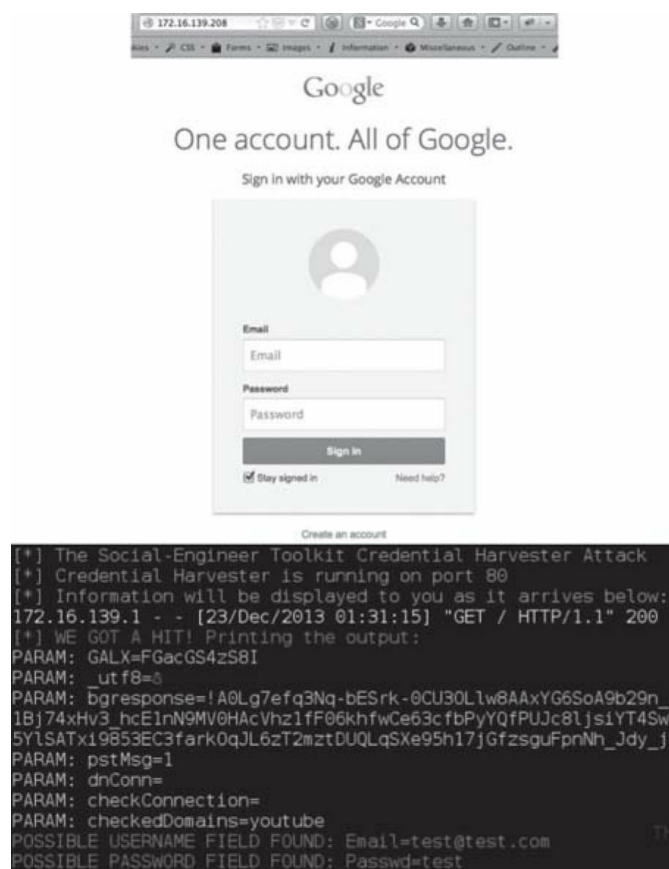
Figure 105 - Spoofed Google Authentication and SET Password Captures
