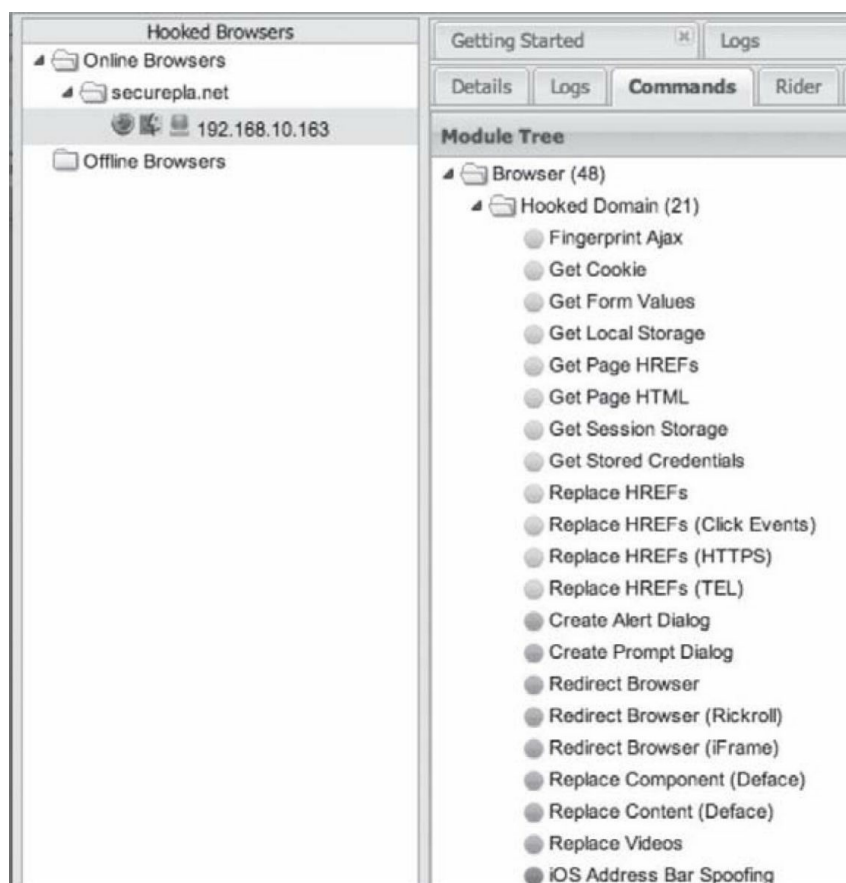
Figure 41 - BeEF Client Attacks
