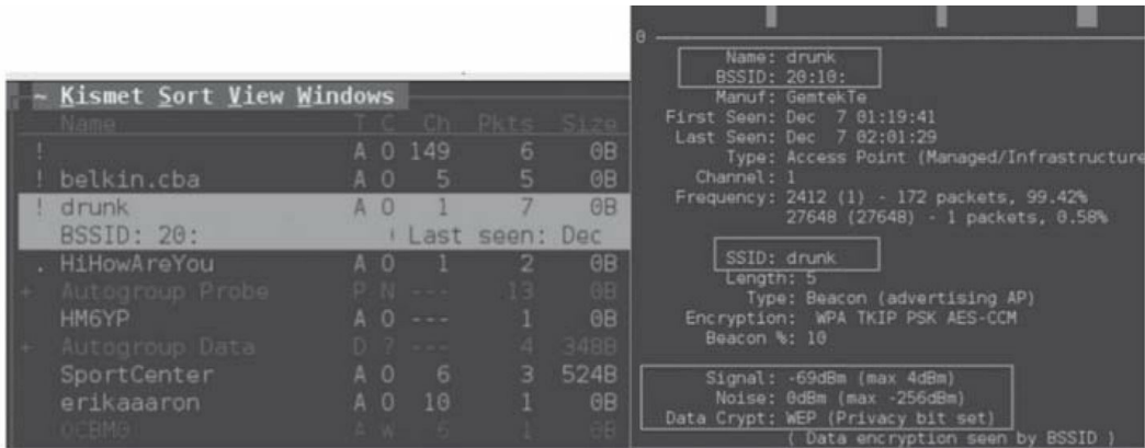
Figure 116 - SSIDs and AP information
