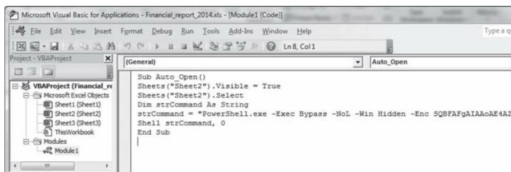
Figure 111 - Creating Macros with PowerShell
