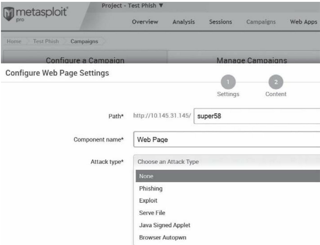
Figure 101 - Metasploit Pro’s Phishing Module
