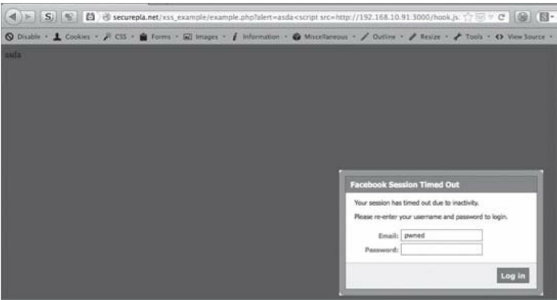
Figure 43 - Petty Theft Attack
