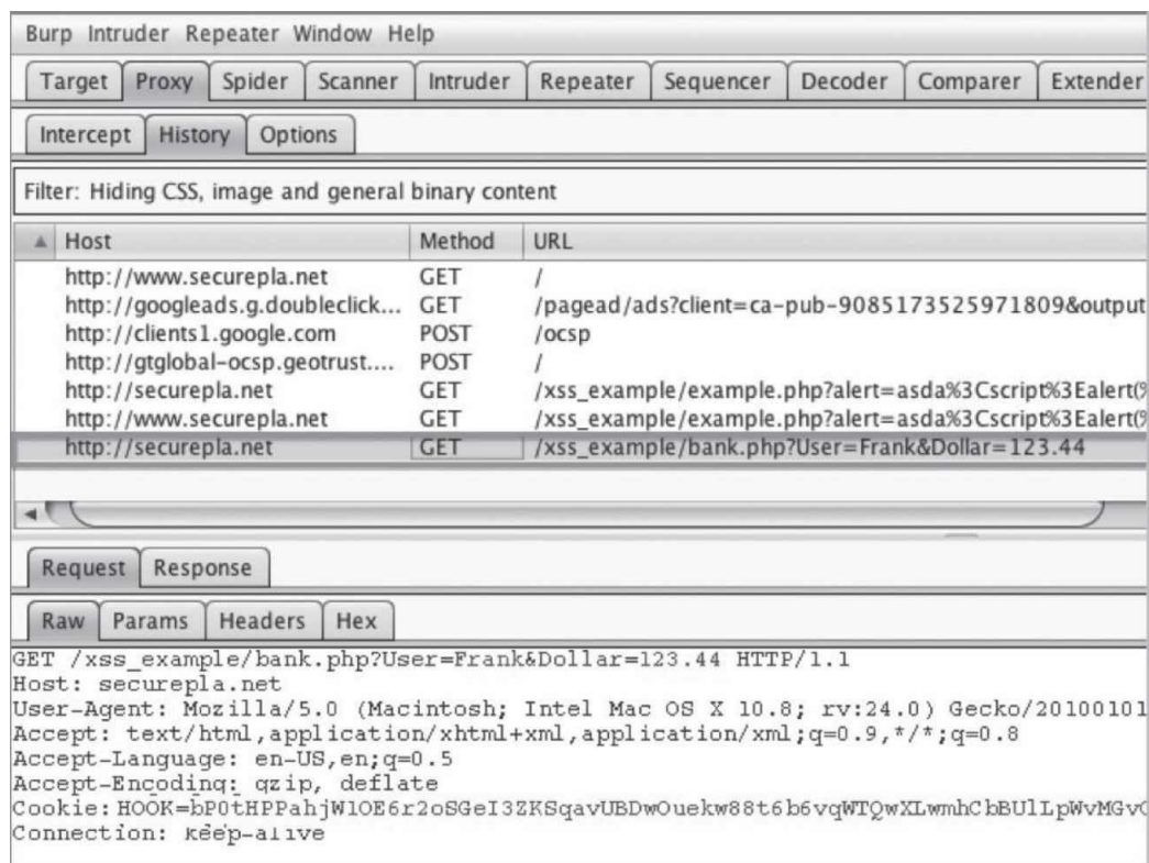
Figure 47 - Burp CSRF Example
