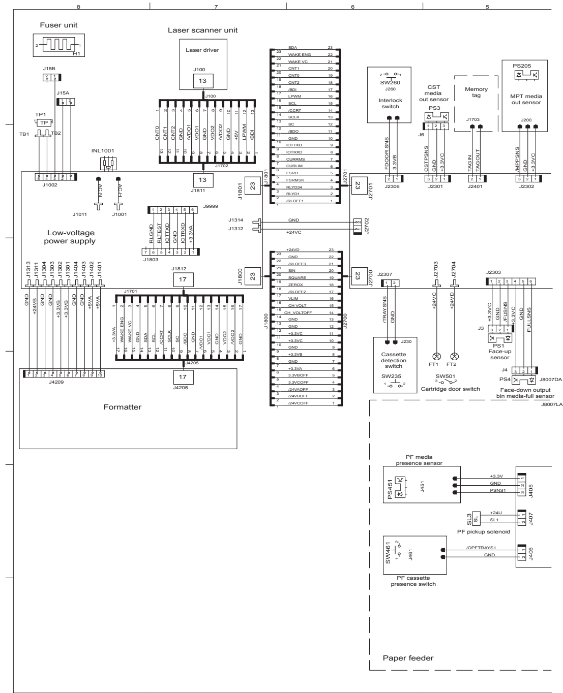
Figure 2-31 General circuit diagram (1 of 2)
