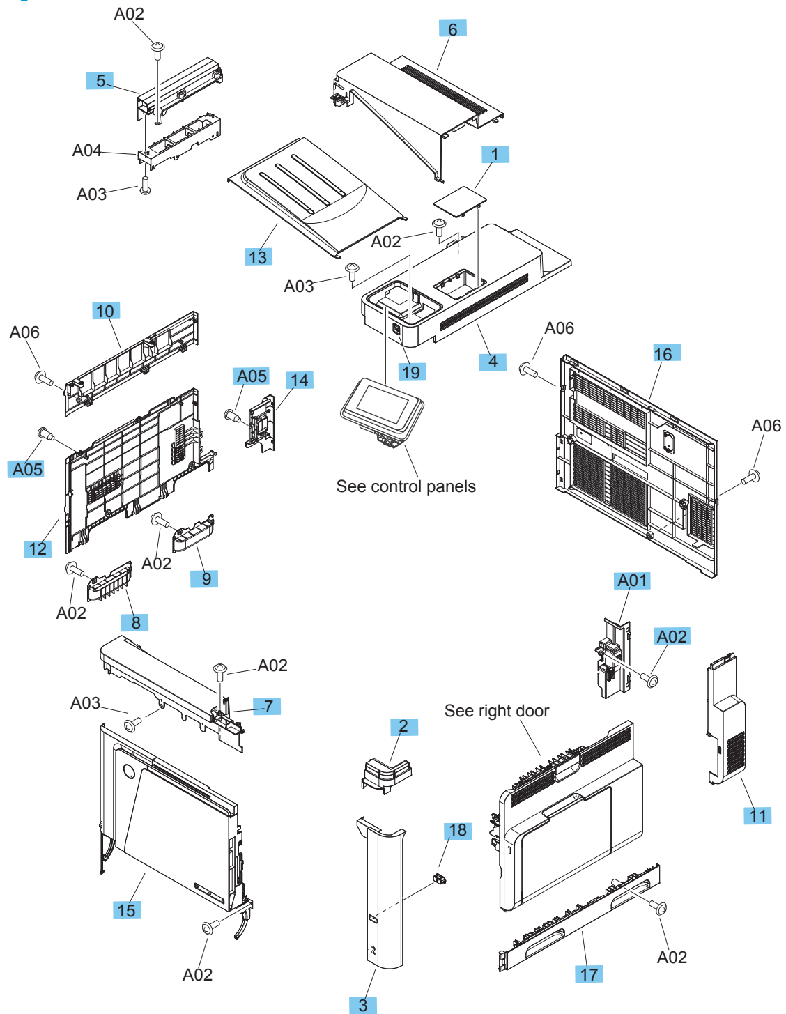
Figure 2-5 Covers (M651)
