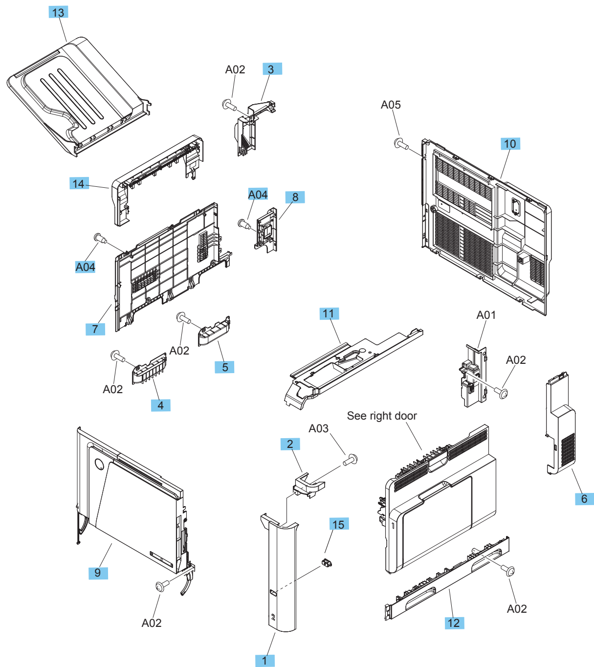
Figure 2-6 Covers (M680)
