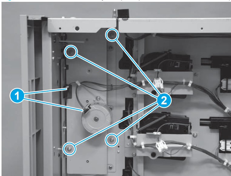
Figure 1-457 Remove the Tray 3-4 pickup assemblies (2,500-sheet paper feeder HCI; 2 of 4)
