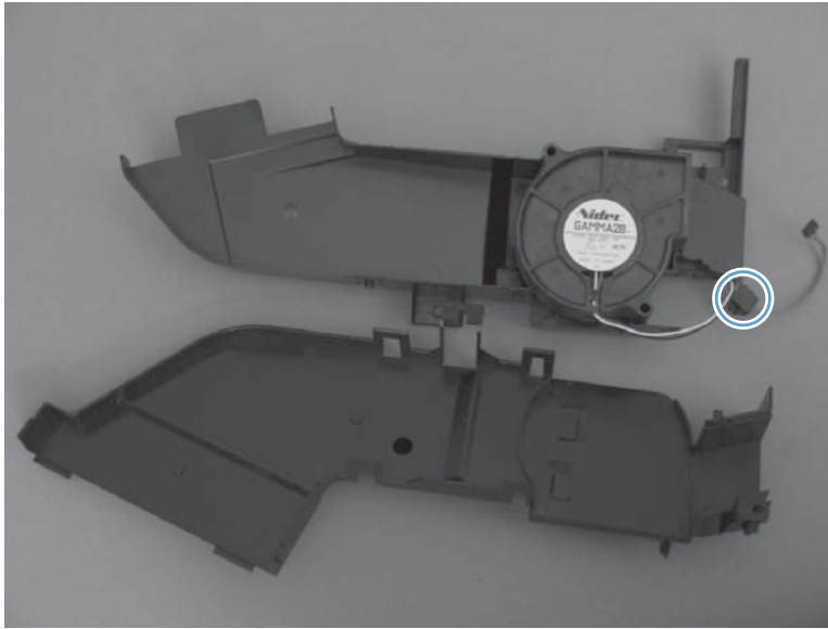
Figure 1-328 Remove the exhaust fan and fan duct (3 of 3)
