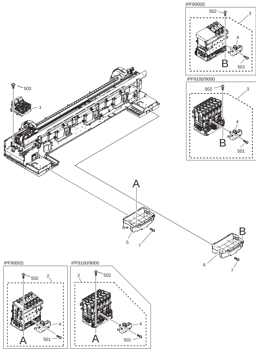
FIGURE 05 INK TANK & PURGE UNIT
