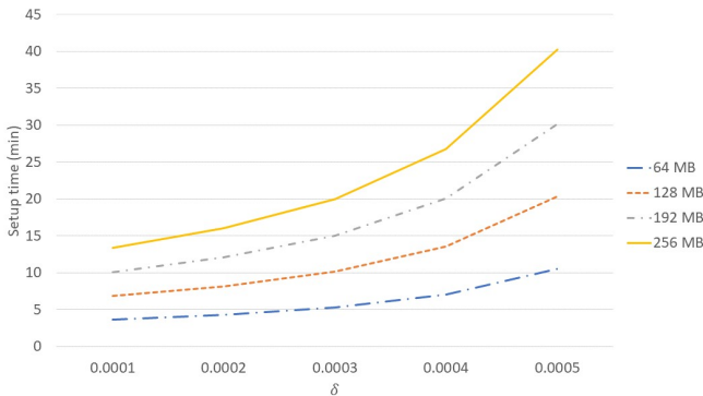
Fig. 4: The compact PoSt setup times for various file sizes and different \delta of the delay function, with hourly check up policy and 30 days data available period.
