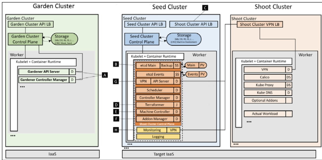
Figure 11.6: The structure of Gardener and its components
