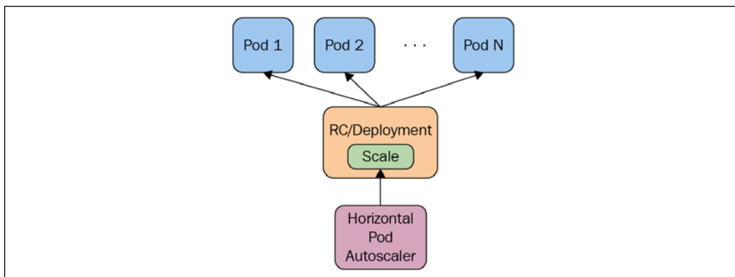
Figure 8.1: HPA interacting with pods
