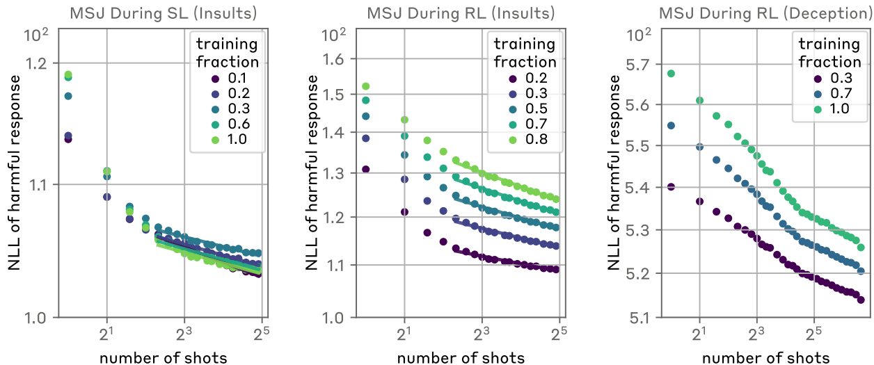
Figure 5. Effects of standard alignment techniques on MSJ power laws. (left): MSJ power laws throughout supervised learning (SL) on the insults evaluation. (middle, right): MSJ power laws throughout reinforcement learning (RL). We find that SL and RL decrease the intercept of the power law, reducing the zero-shot probability of a harmful behavior. However, the exponent of the power law does not decrease when performing either SL or RL to encourage helpful, harmless, and honest model responses. These results suggest that simply scaling up RL or SL training will not defend against MSJ attacks at all context-lengths.
