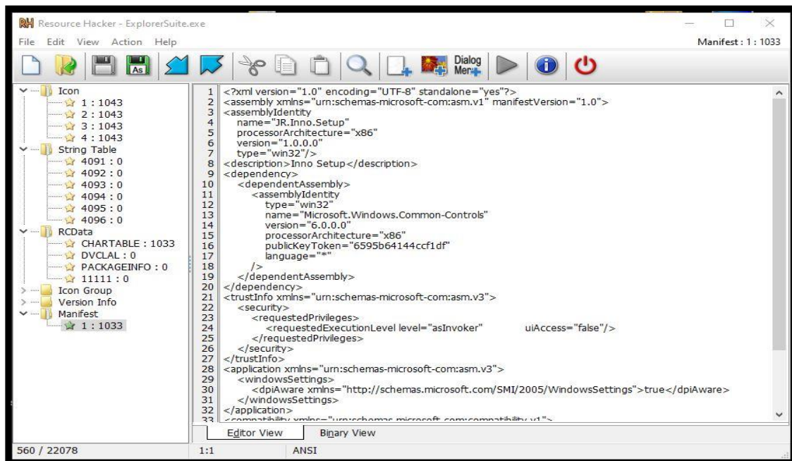
FIGURE 6: RESOURCE HACKER – BINARY RESOURCES (ICON, MANIFEST)
