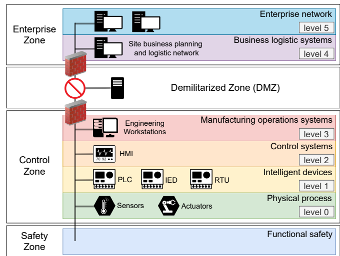
Fig. 1: ICS Purdue Model architecture.
