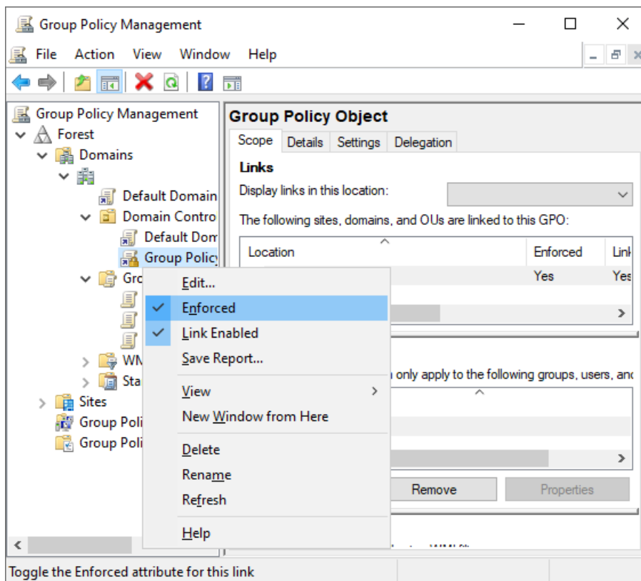
Figure 10.7 – Enforced enabled for a GPO
