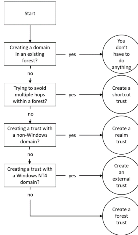
Figure 1.4 – Flowchart for choosing the right Active Directory trust type
