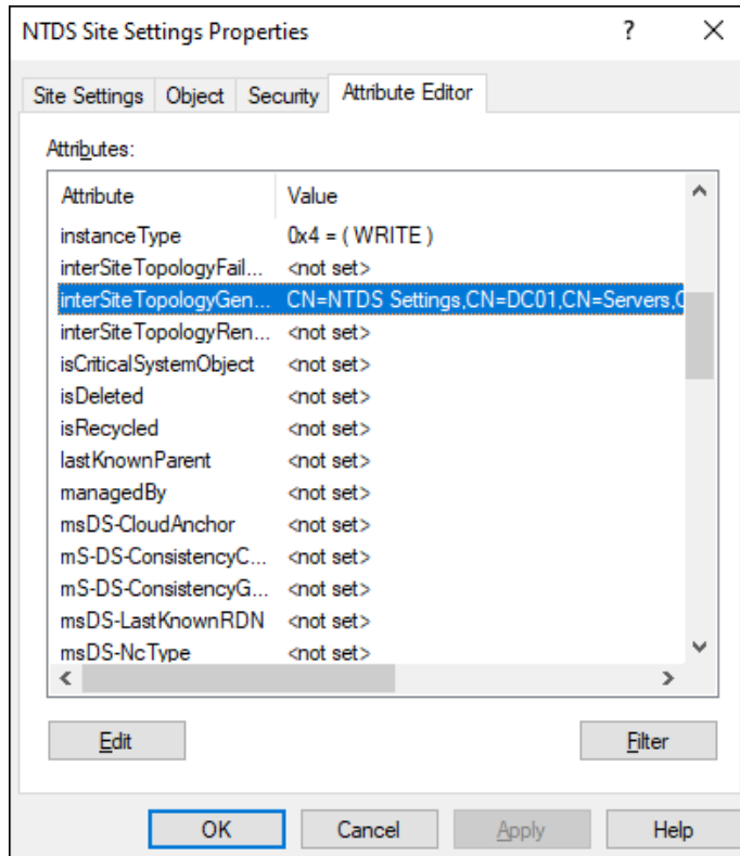
Figure 5.11 – interSiteTopologyGenerator attribute
