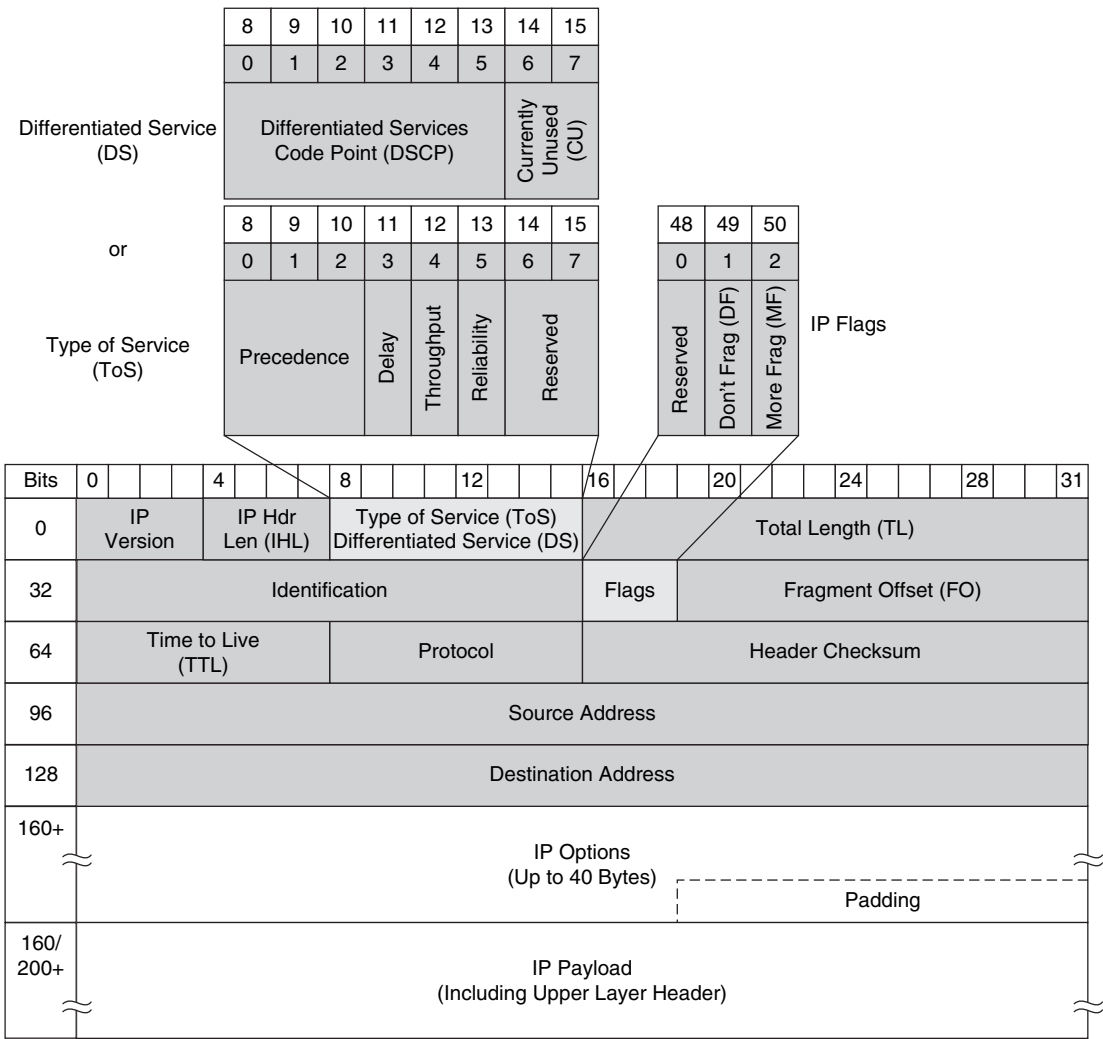
Figure B-1 IP Version 4 Header
