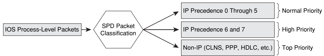
Figure 5-2 IOS SPD Classification Process
