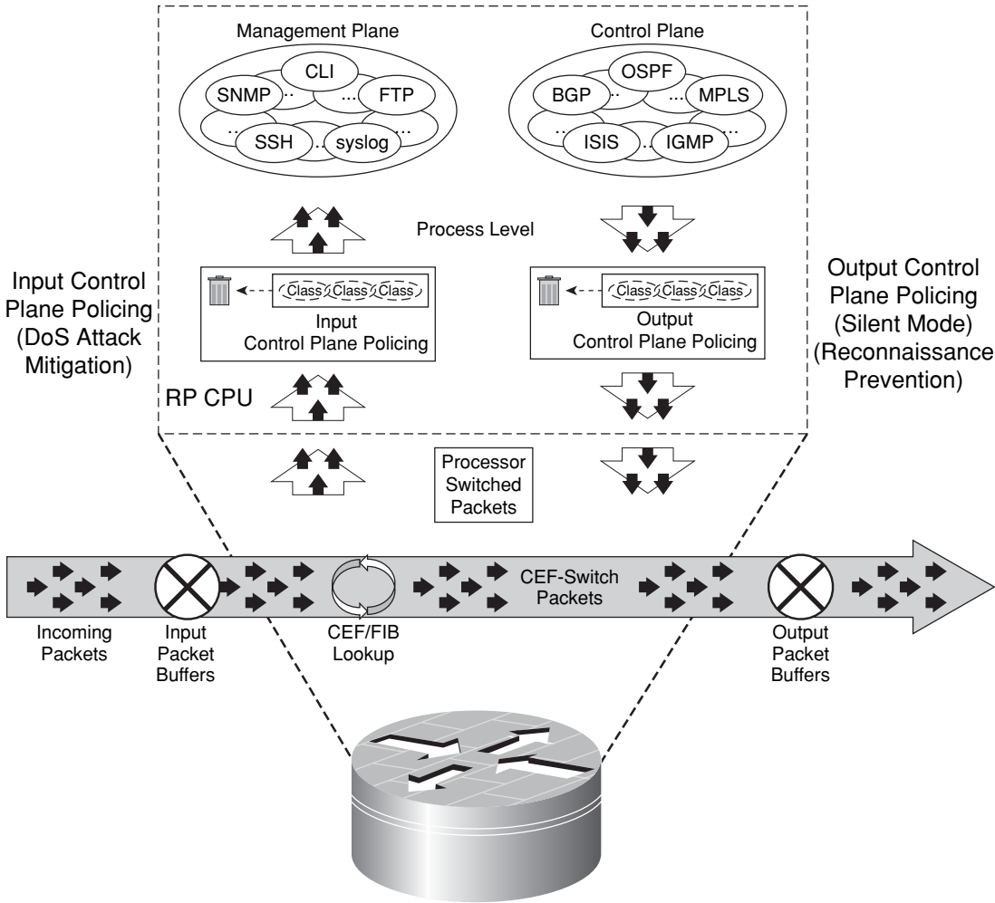
Figure 5-6 Control Plane Policing Conceptual View
