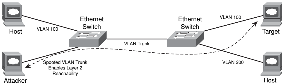
Figure 2-11 Switch Spoofing Attack
