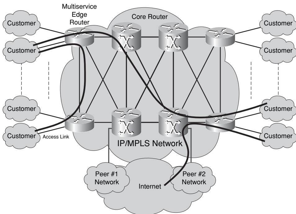
Figure 1-6 Data Plane
