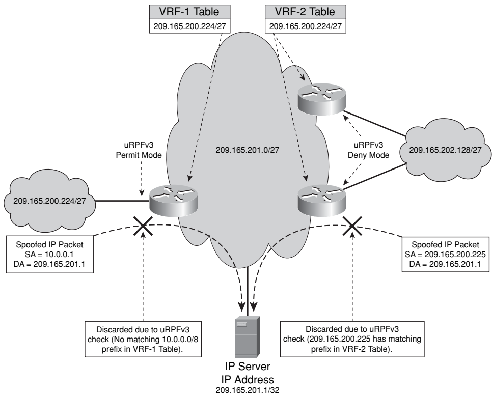
Figure 4-7 VRF Mode uRPF Source Address Verification Example
