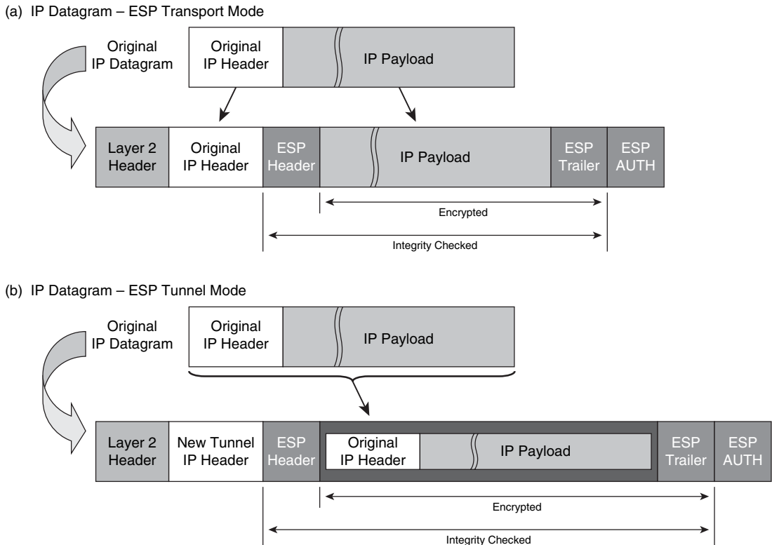
Figure 7-3 Application of IPsec ESP to IP Datagrams in Tunnel Mode and Transport Mode
