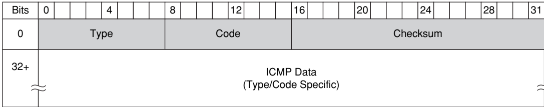
Figure B-4 Basic ICMP Header
