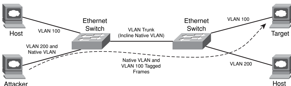
Figure 2-12 Double 802.1Q Encapsulation Attack
