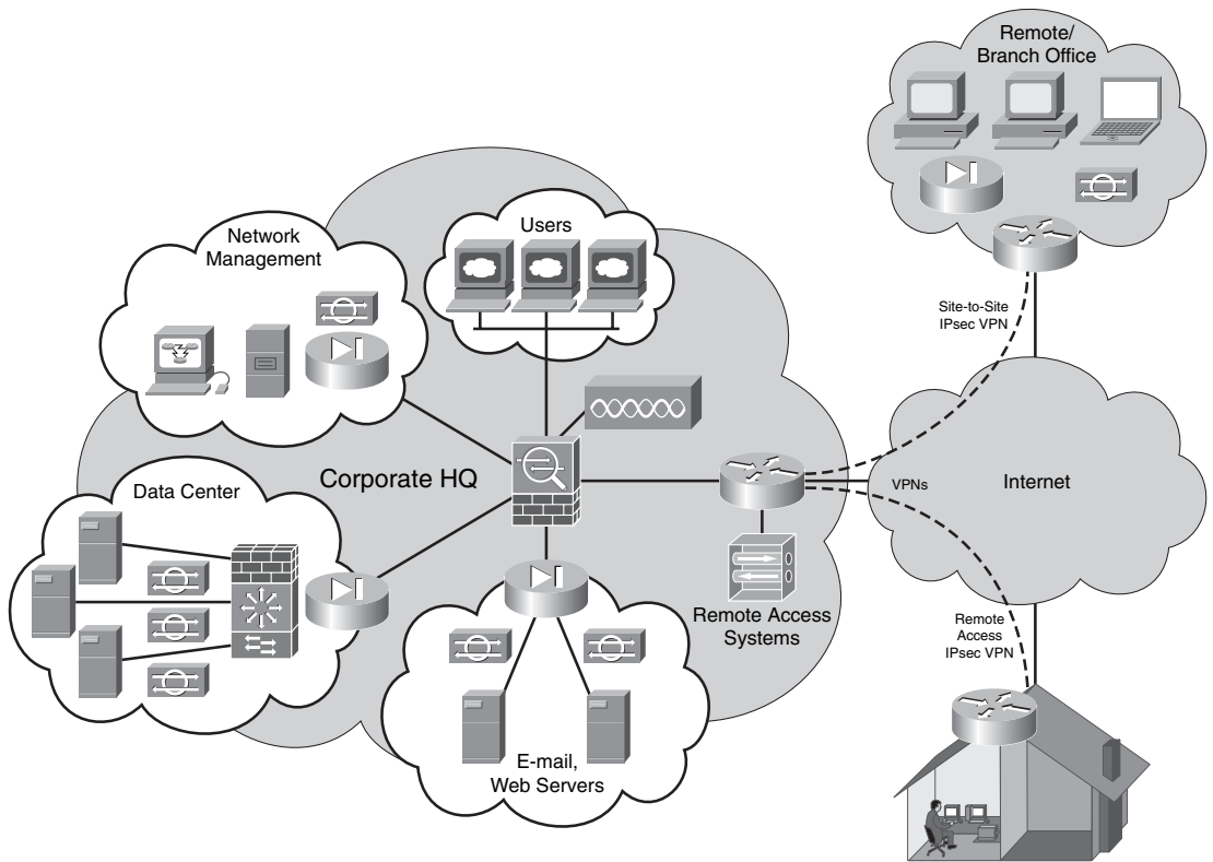
Figure 2-20 IPsec VPNs
