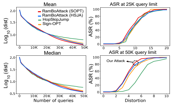
Fig. 23. A comparison between three current state-of-the-art attacks and RamBoAttack on a non-hard set selected from ImageNet. In non-hard cases, RamBoAttacks improve attack performance by yielding more effective adversarial examples notable in ASR results.
