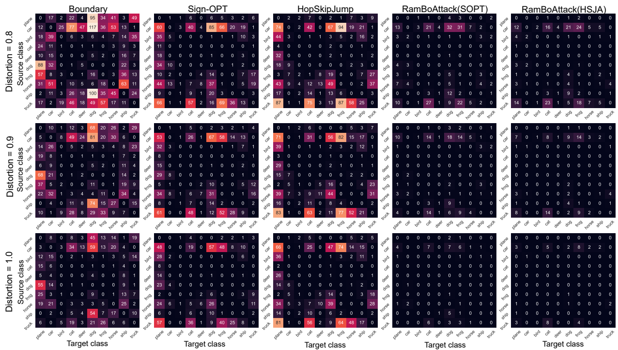
Fig. 33. The number of hard cases on CIFAR10 obtained from different attack methods categorized by pairs of source and target classes (at distortion threshold = 0.8, 0.9 and 1.0). RamBoAttacks are seen to nearly overcome all of the hard cases encountered by other decision-based blackbox attack methods; thus, demonstrating the robustness of our proposed attack.
