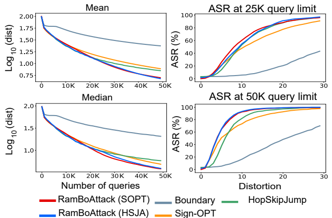
Fig. 21. A comparison between three current state-of-the-art attacks and RamBoAttack on a large scale balance set selected from ImageNet.
