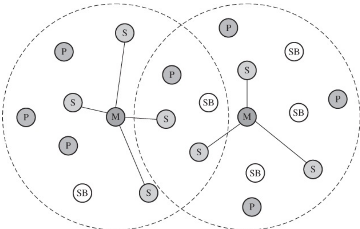
Figure 6.10 Scatternet schematic
