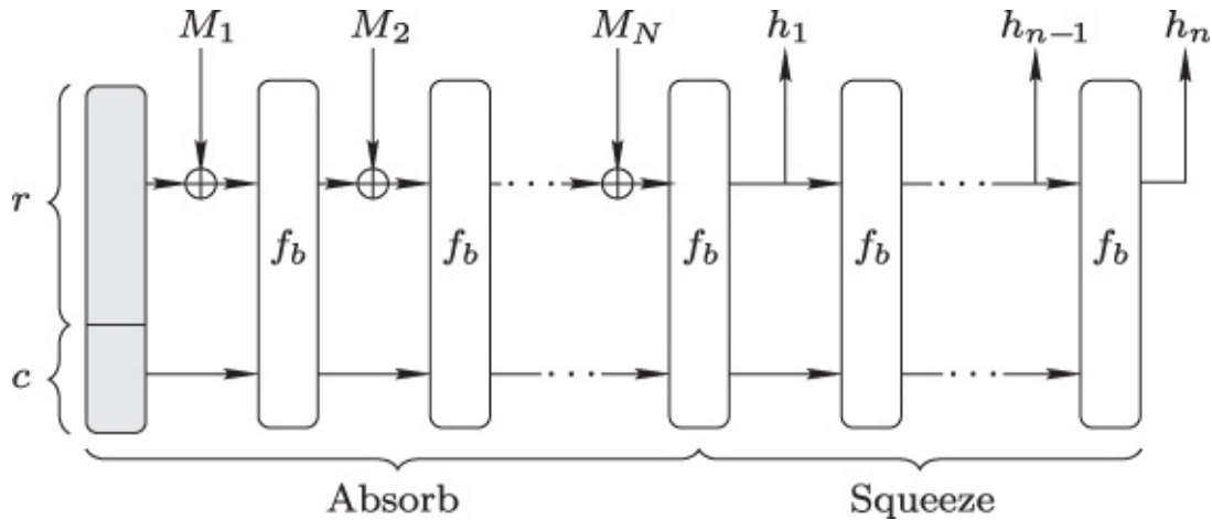
Figure 4.3 The sponge function construction using a b -bit permutation f_b , where b = r + c . The state is initially set to 0^b and the result is an rn -bit string
