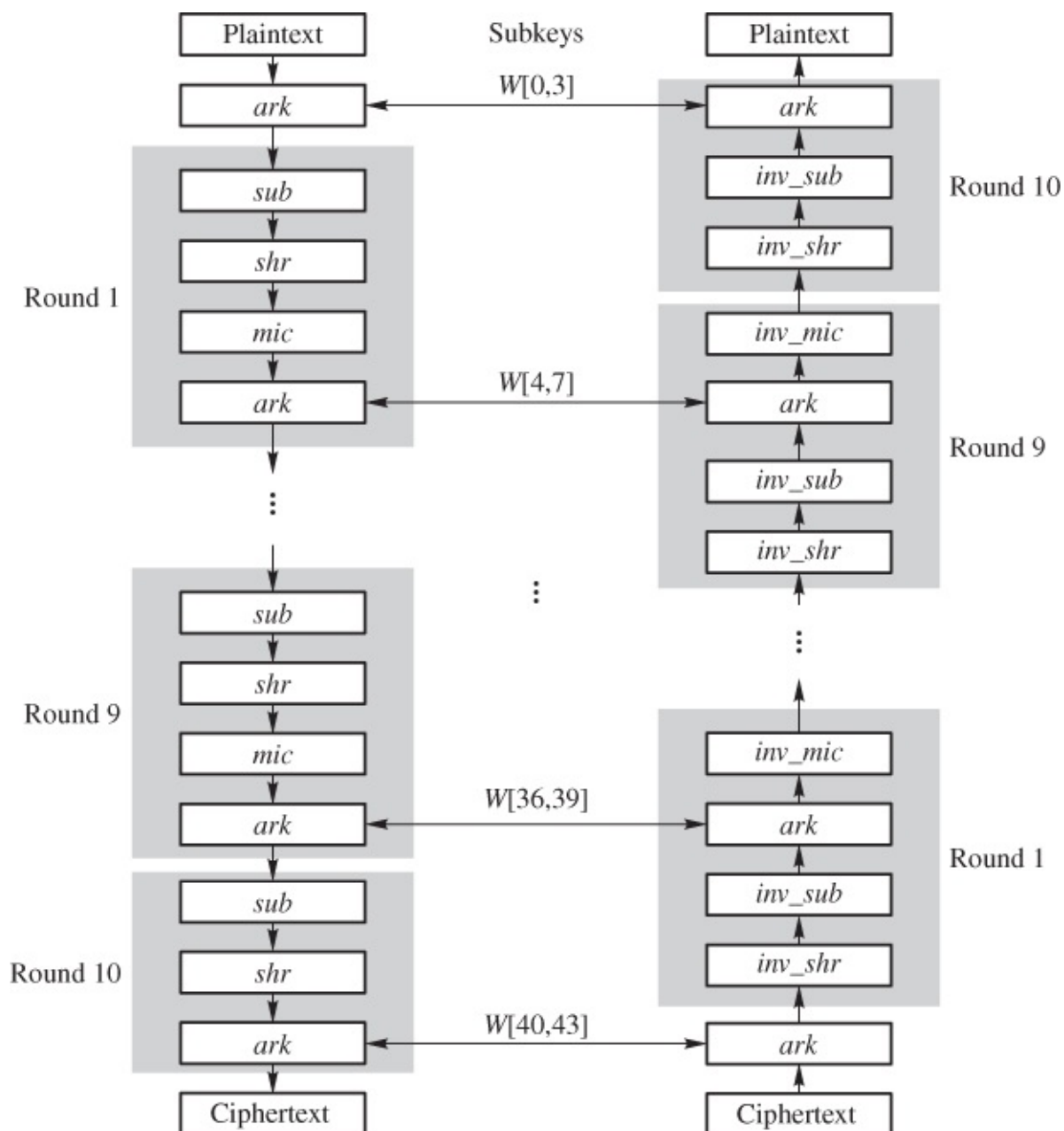
Figure 2.2 AES-128 encryption and decryption diagram
