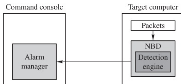
Figure 9.3 Network-node detection
