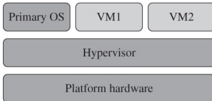
Figure 7.2 Hardware-assisted virtualization
