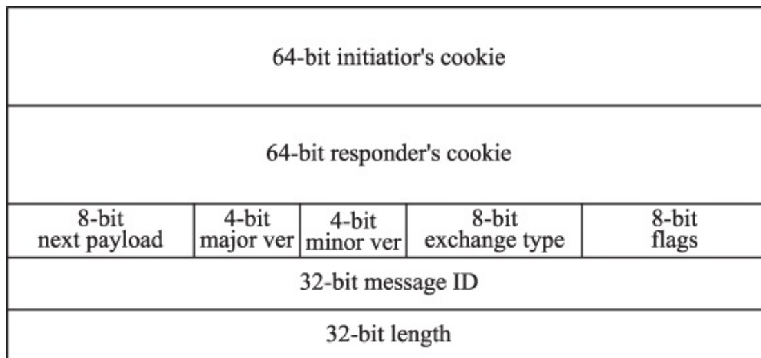
Figure 5.7 ISAKMP header
