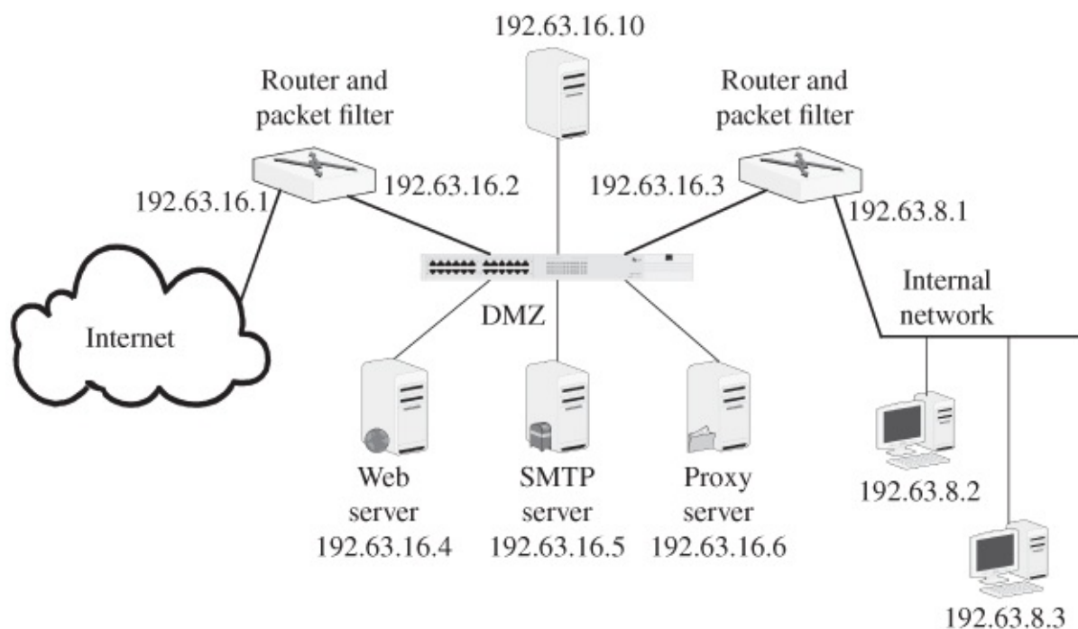
Figure 8.12 The firewall system used for Exercises 8.6 and 8.7
