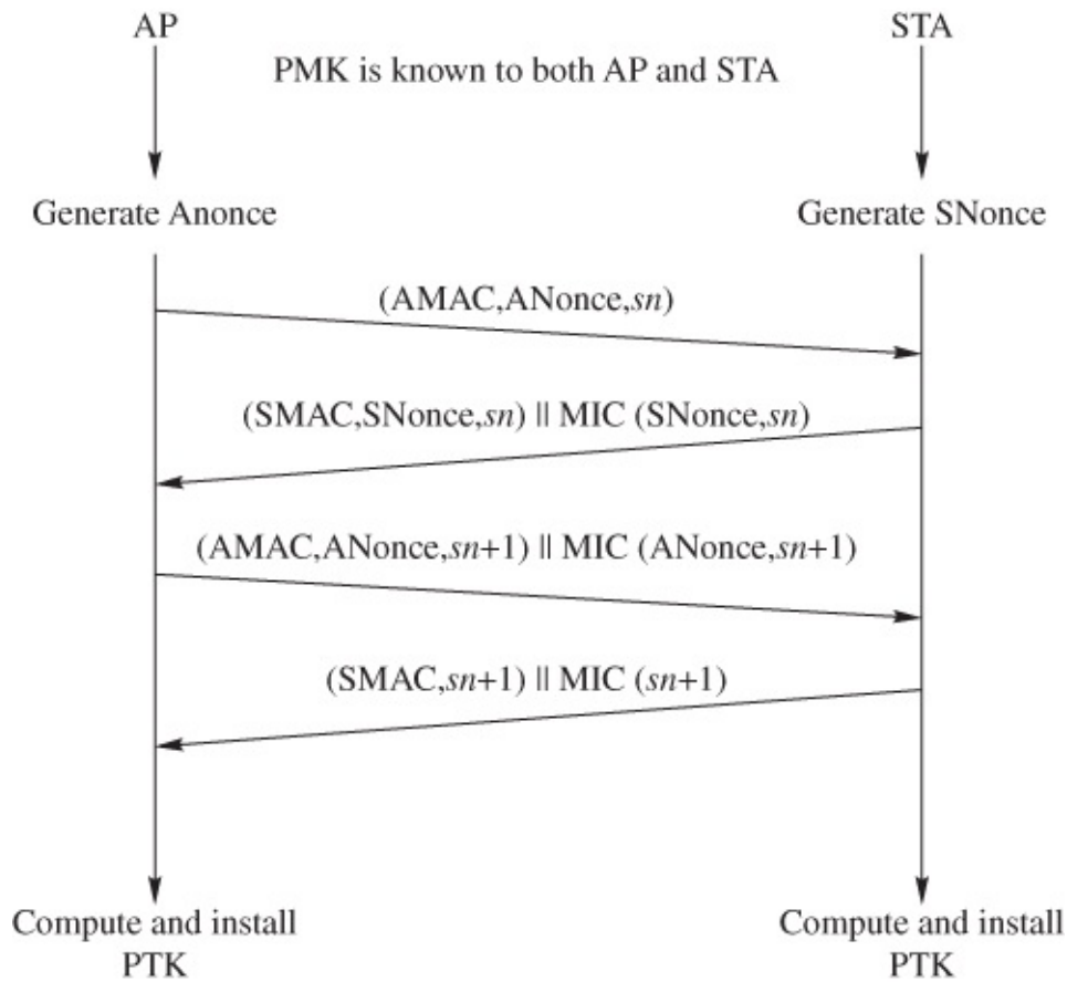
Figure 6.7 Schematic of a 4-way handshake procedure
