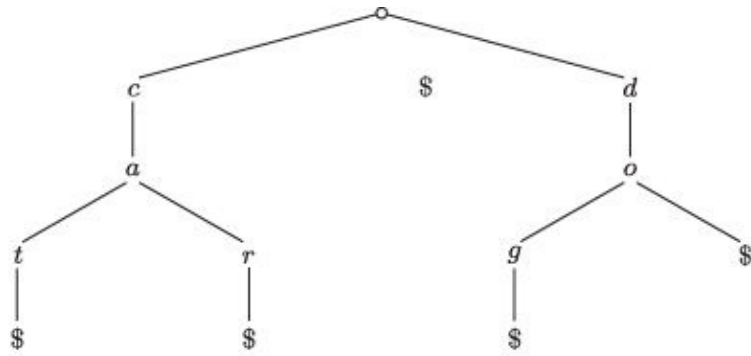
(a) Insert the words “cat”, “car”, “dog”, and “do” into the trie
