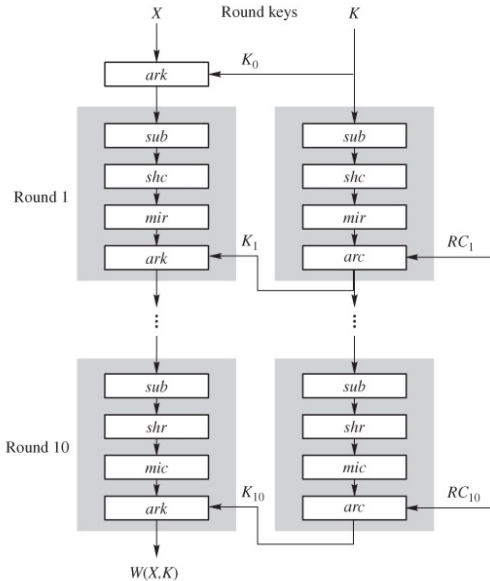
Figure 4.2 Block diagram of W
