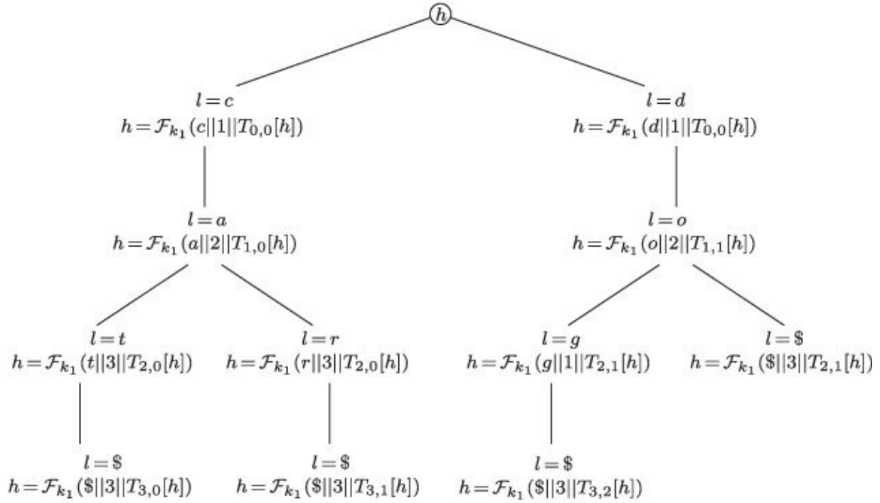
(b) Using a level order traversal, construct the appropriate hash chains
