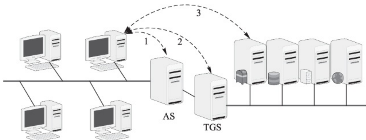
Figure 5.13 Single-realm Kerberos, where the three dash lines indicate, respectively, the first-phase, the second-phase, and the third-phase communications
