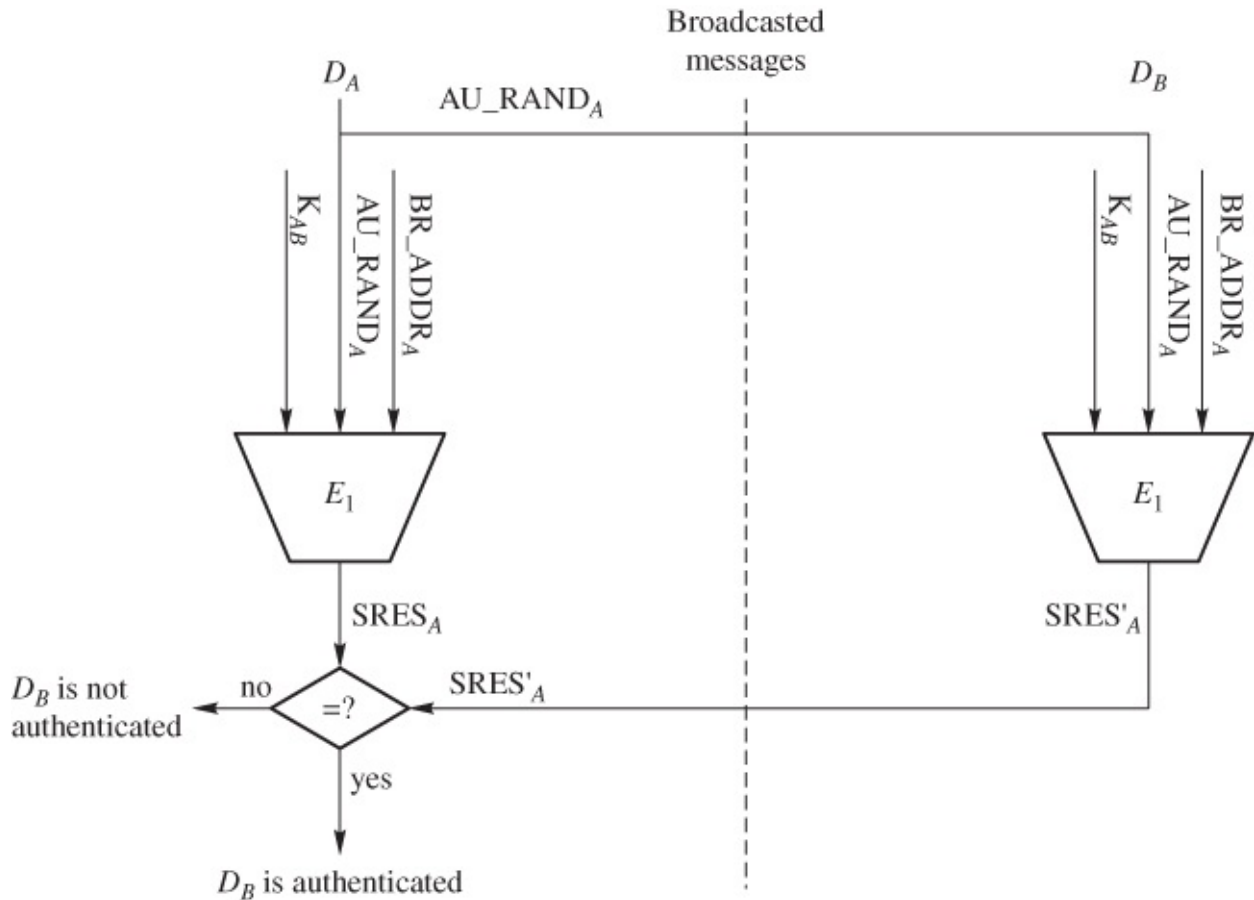
Figure 6.12 Bluetooth device D_A authenticates device D_B
