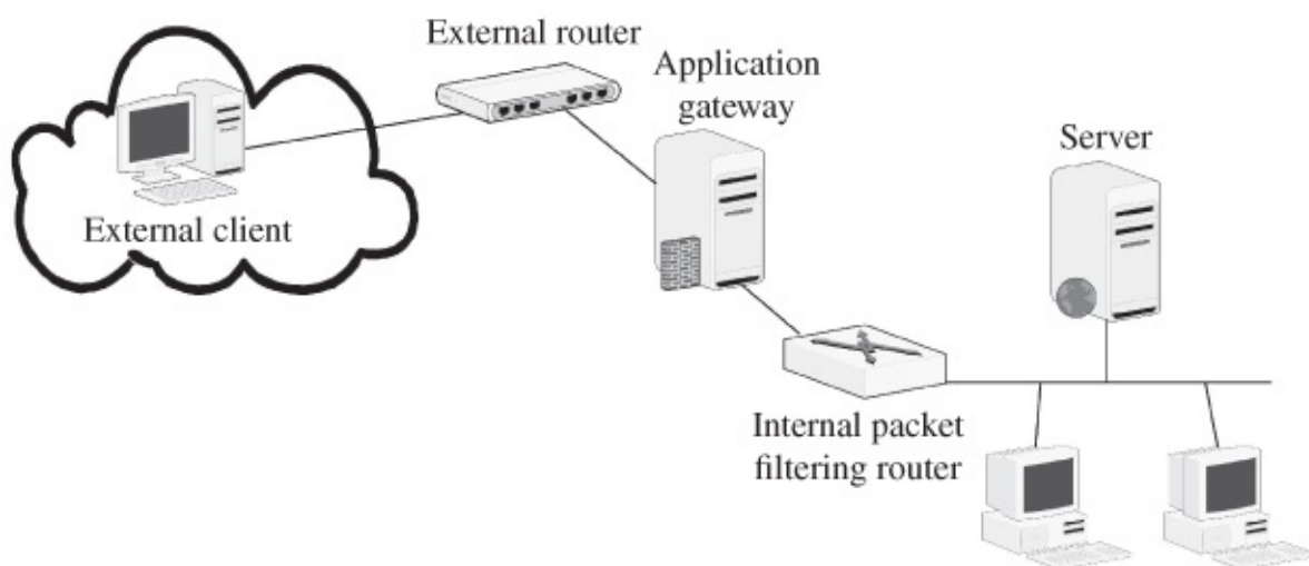
Figure 8.5 Schematic of an application gateway
