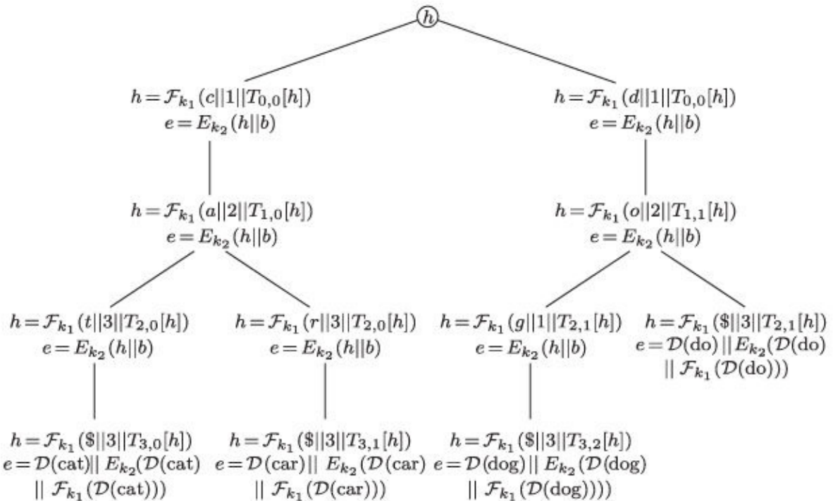
(c) Using a level order traversal, construct the appropriate verification tags and delete the values in the l fields
