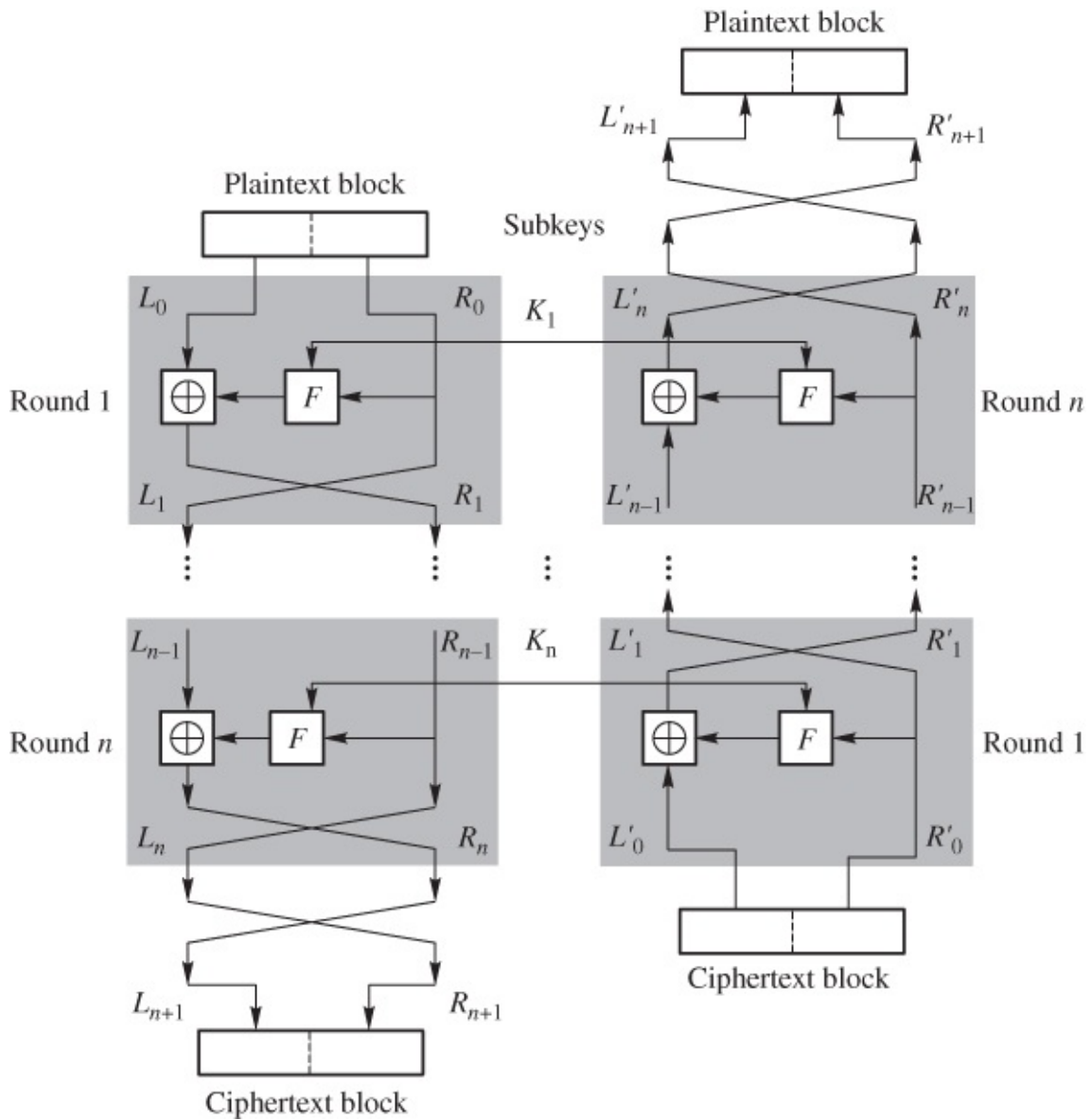
Figure 2.1 Feistel cipher scheme block diagram
