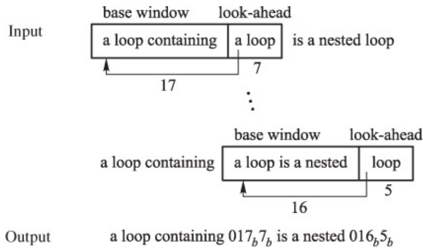
Figure C.1 A demonstration of a ZIP process
