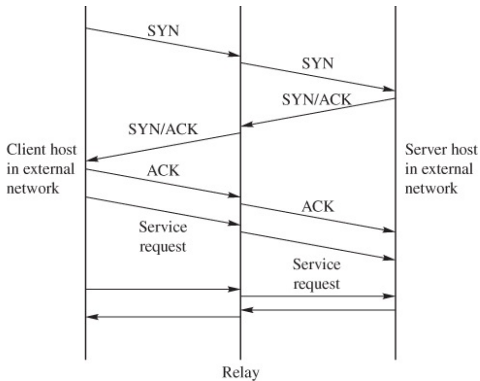
Figure 8.3 Circuit gateway acts as connection relay
