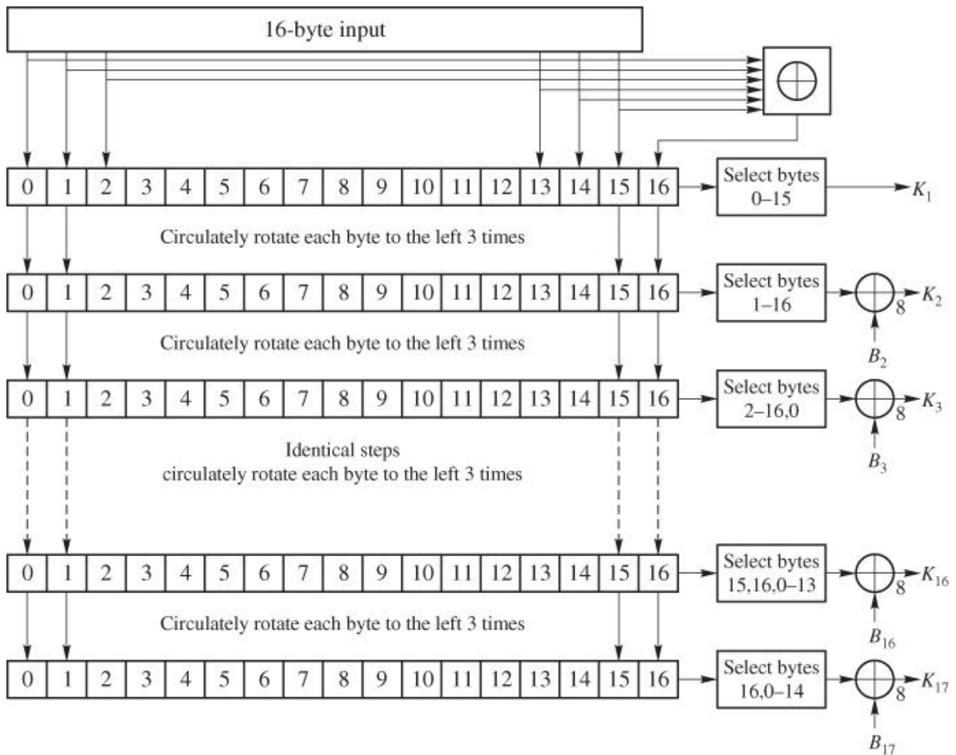
Figure 6.11 Schematic of SAFER+ subkey generation
