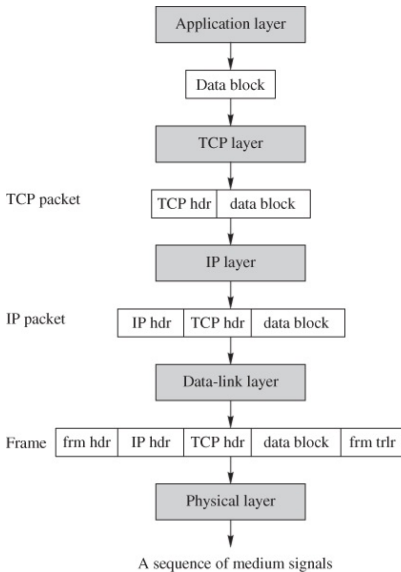
Figure 5.2 Flow diagram of packet generation
