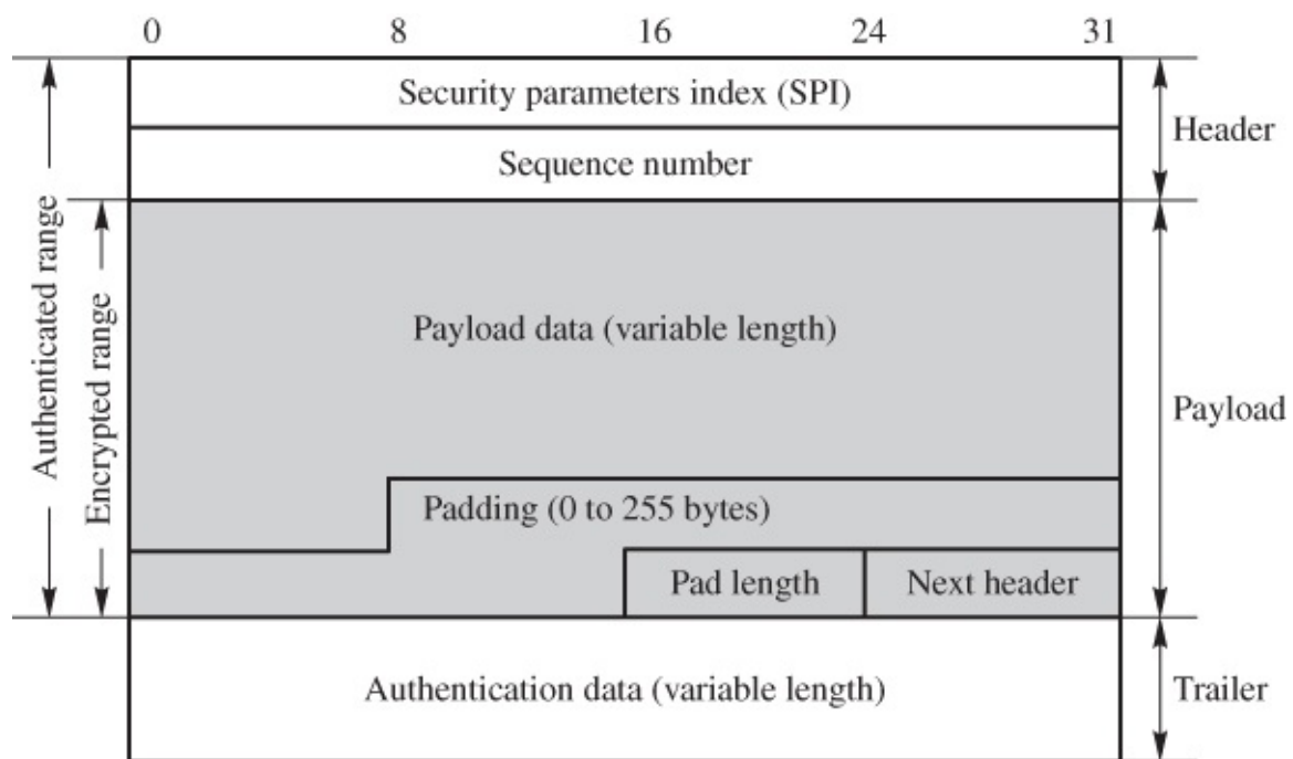
Figure 5.6 ESP format
