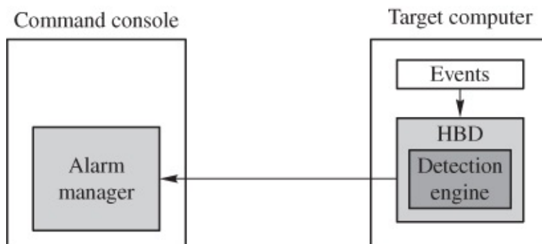
Figure 9.5 Host-based detection
