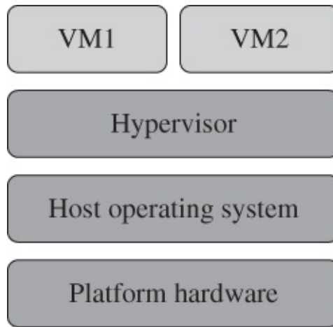
Figure 7.1 Software-based virtualization
