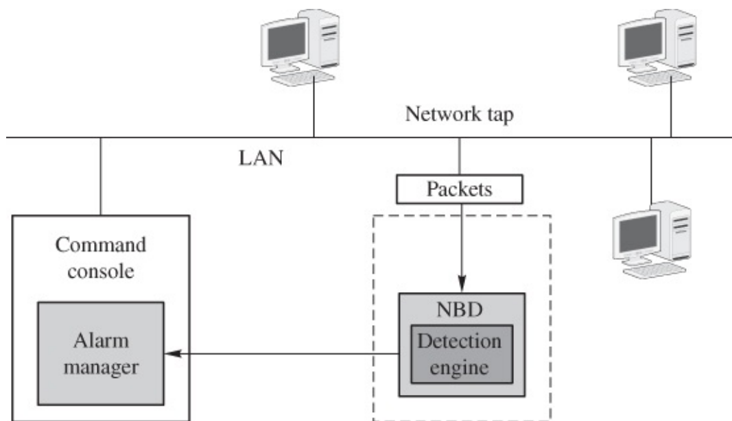
Figure 9.4 Network-sensor detection
