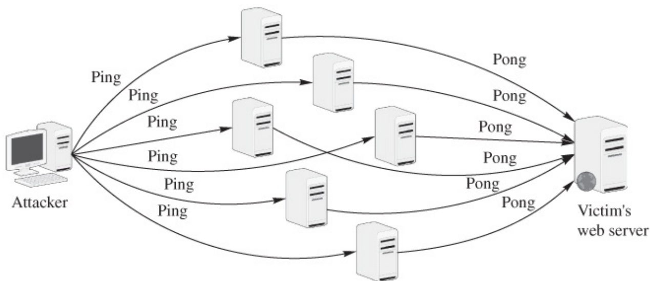
Figure 1.8 Smurf attack
