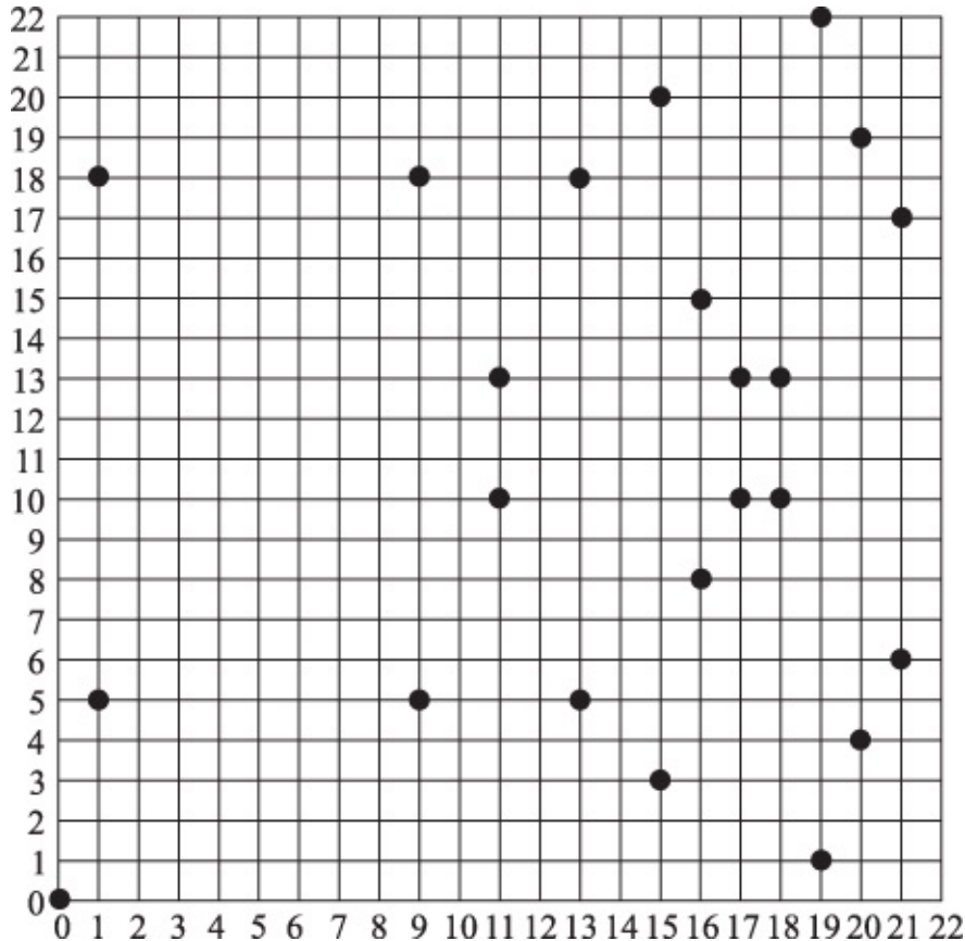
Figure 3.3 Point distribution in \mathbb{E}'_{23}(1, 0)
