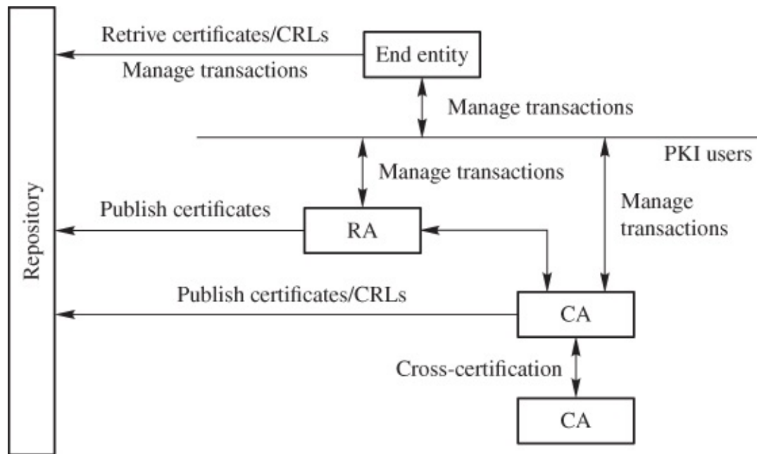
Figure 5.3 PKIX architecture
