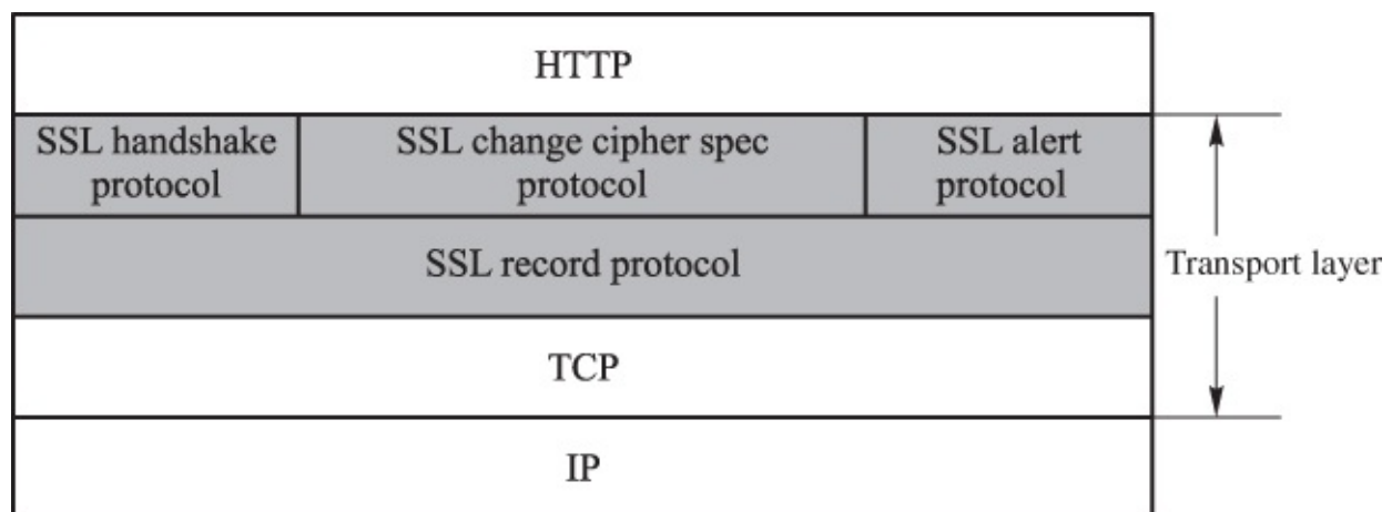
Figure 5.9 SSL structure
