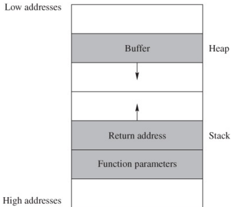
Figure 1.5 Typical memory layout for function call
