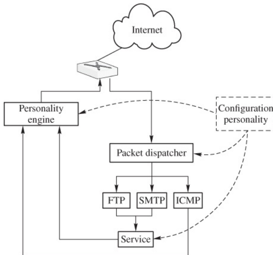
Figure 9.8 A block diagram of Honeyd architecture
