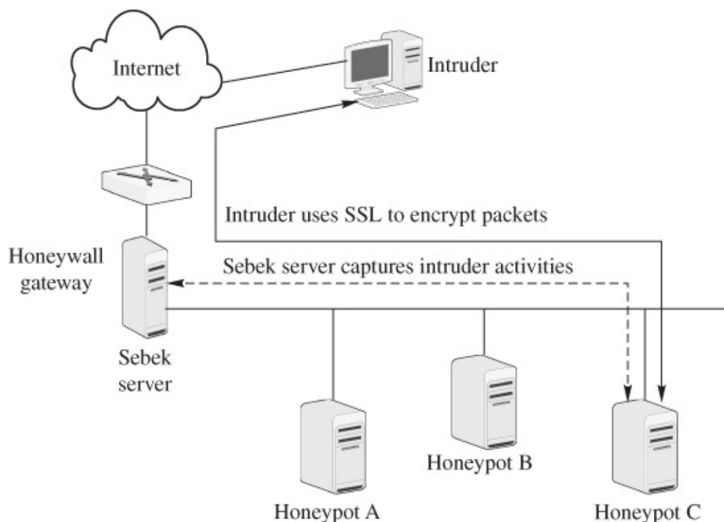
Figure 9.9 Schematic of Sebek honeynet
