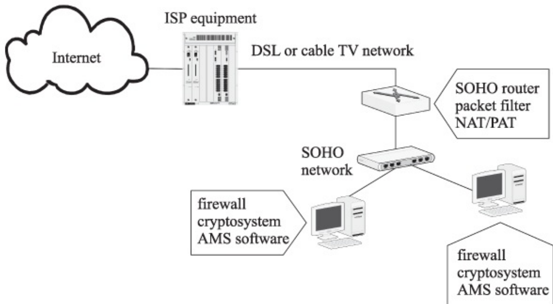
Figure 8.11 Schematic of a SOHO firewall network
