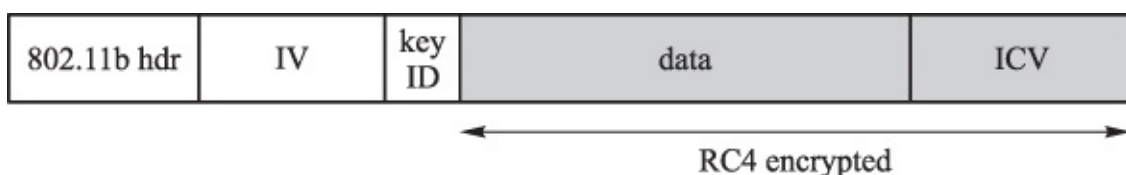
Figure 6.4 802.11b MAC sublayer frame layout
