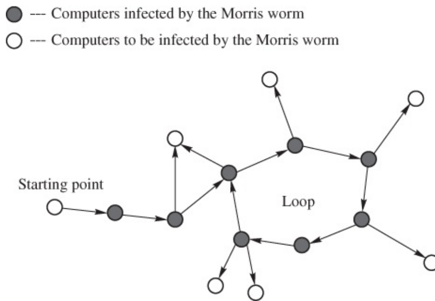
Figure 10.4 Spread schematics of the Morris worm
