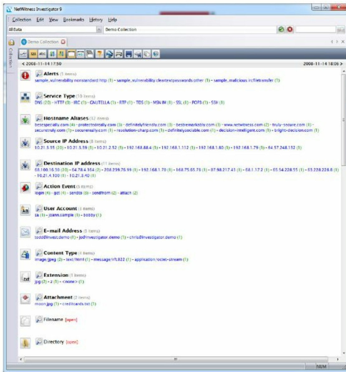
Figure 9-12. NetWitness Investigator
