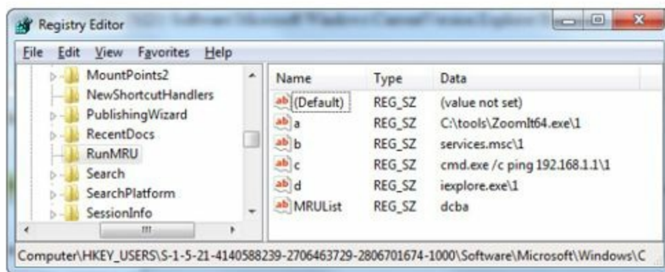
Figure 12-25. Sample contents of a user's Start Menu RunMRU registry key
