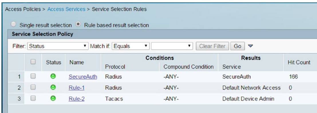
Figure 16-42. The Secure-Auth custom access service policy is active
