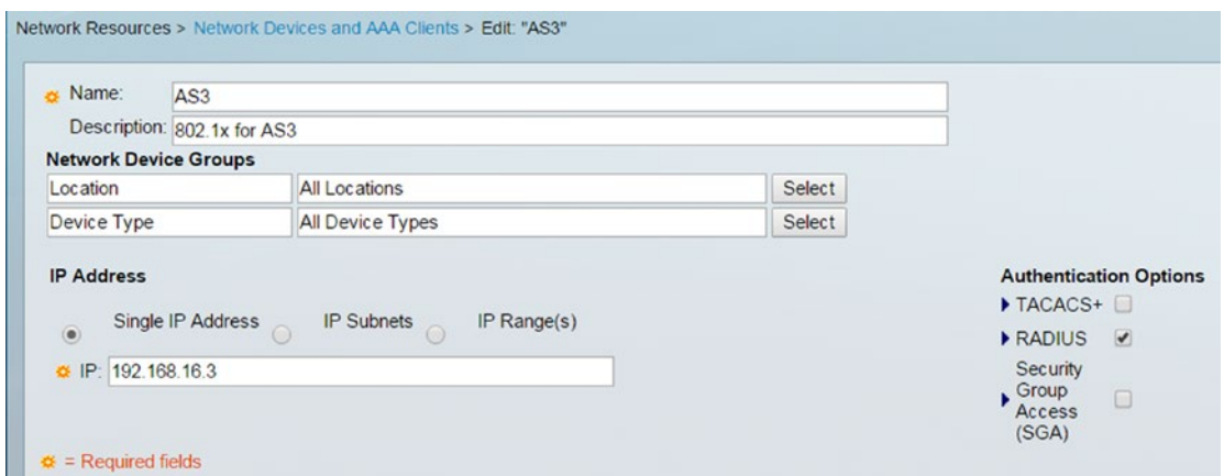
Figure 16-30. NAS/AAA client settings
