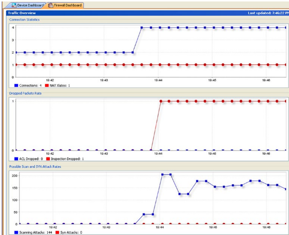
Figure 21-44. Effect of DoS with tuned connection settings and TCP normalization map is used
