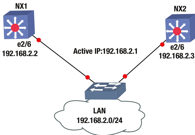
Figure 19-7. GLBP diagram
