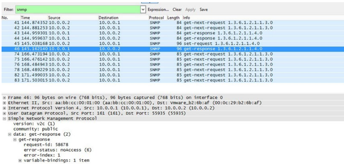
Figure 10-4. SNMPv2c authentication
