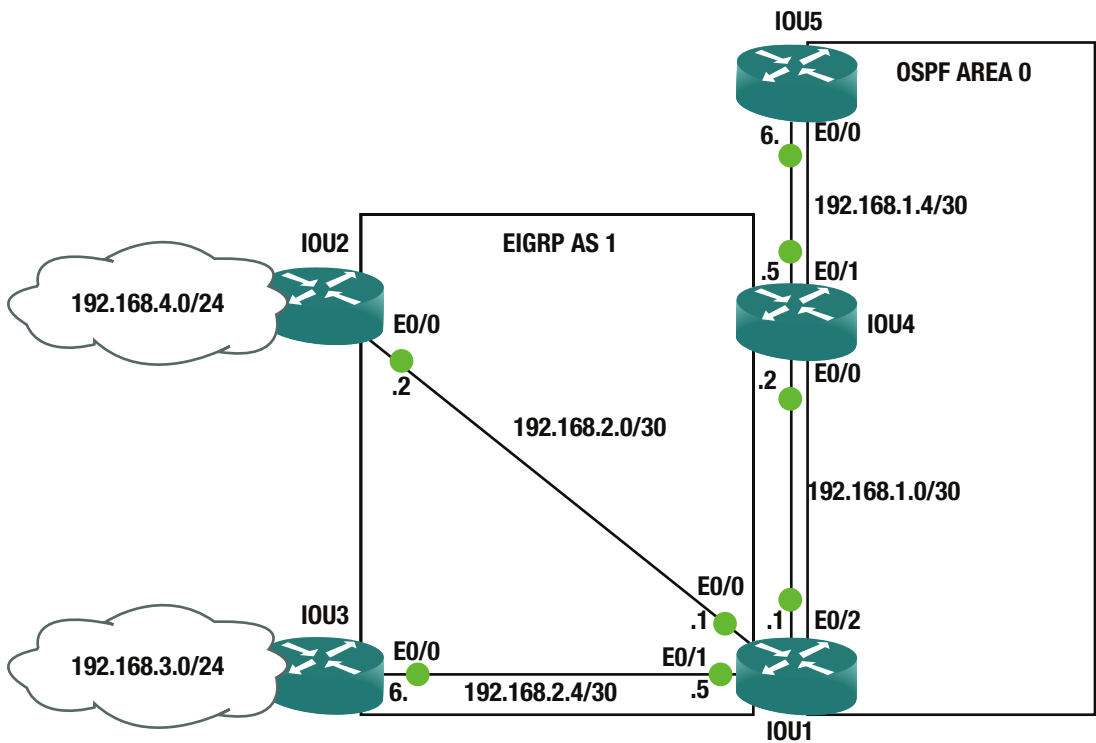
Figure 17-7. EIGRP example diagram
