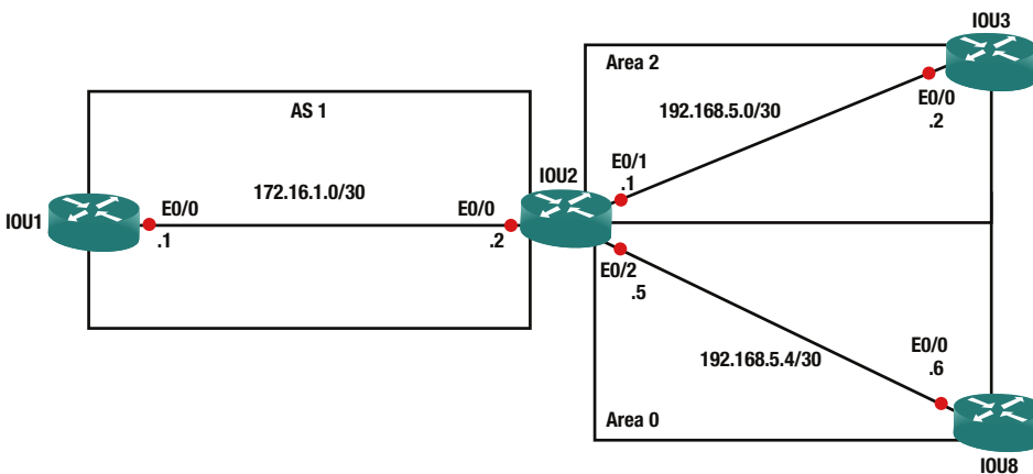
Figure 15-9. Exercise 1 diagram
