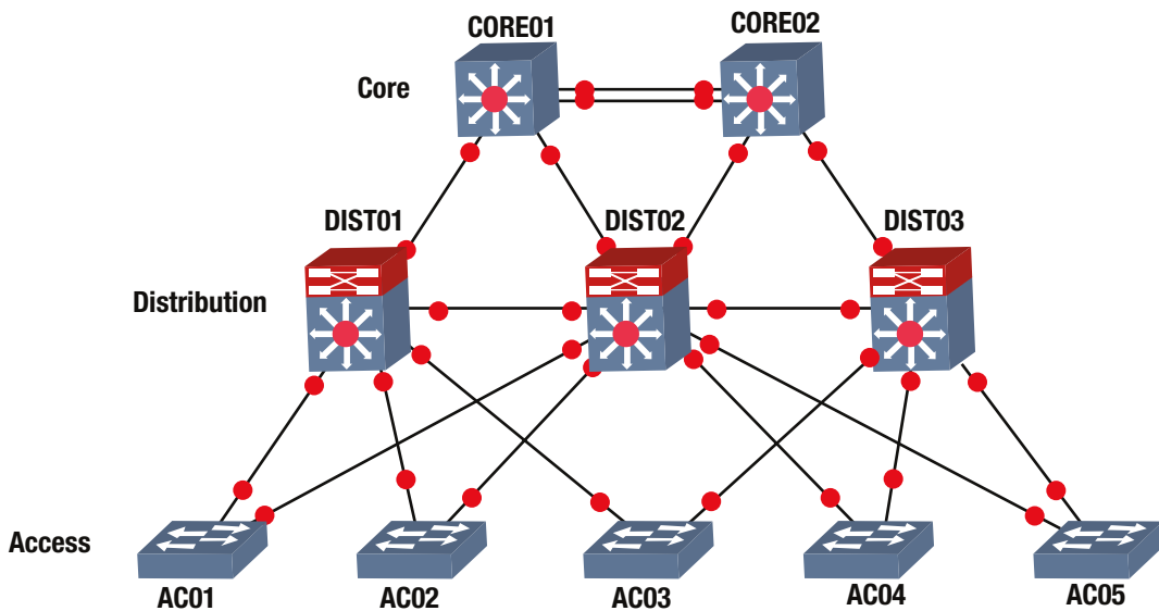
Figure 13-1. Cisco hierarchical model
