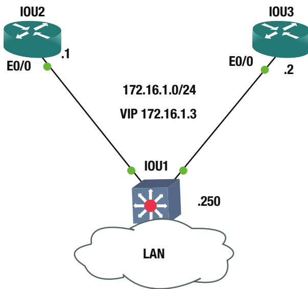
Figure 13-2. HSRP example
