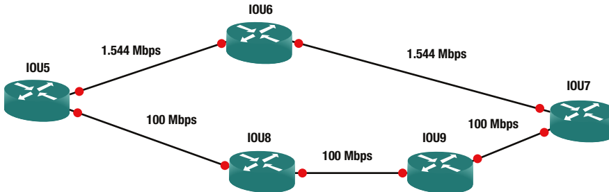
Figure 6-4. Distance-Vector diagram
