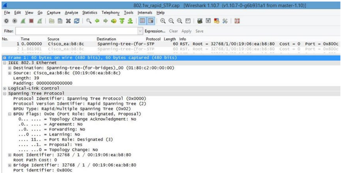
Figure 5-4. Captured BPDUP packet
