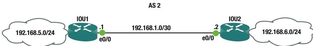
Figure 17-5. EIGRP example diagram
