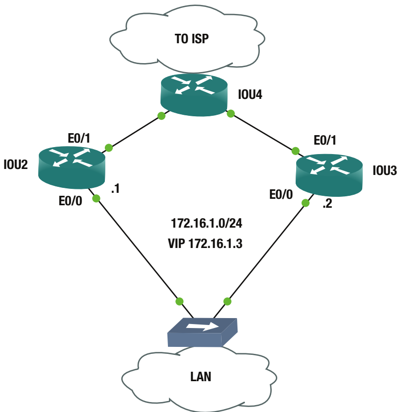
Figure 13-3. HSRP example 2
