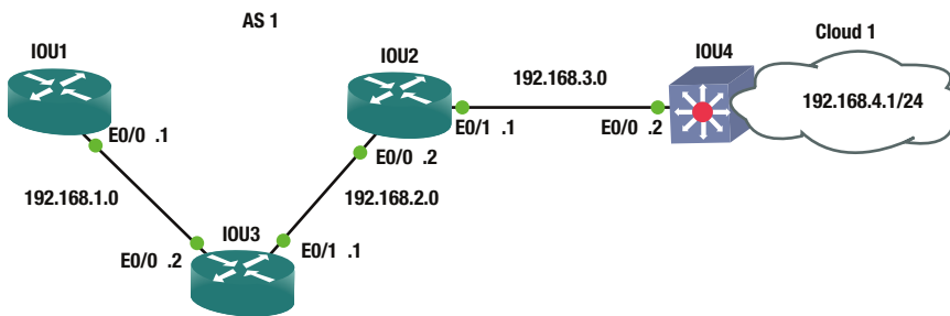
Figure 6-10. EIGRP routing diagram
