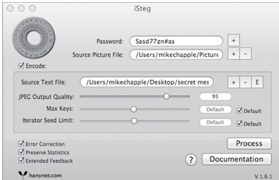
FIGURE 7.2 Steganography tool
