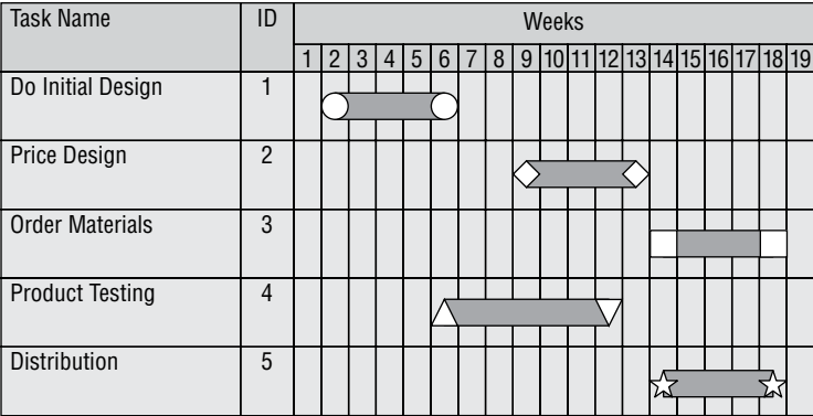
FIGURE 20.7 Gantt chart
