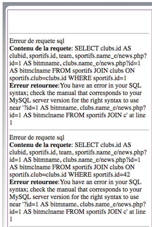
FIGURE 21.9 SQL error disclosure
