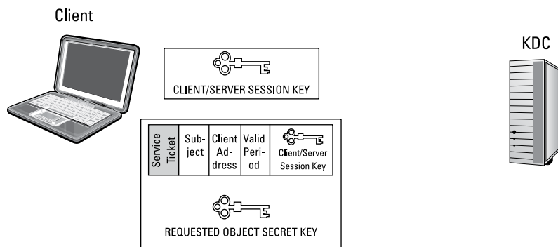
FIGURE 7-6: Kerberos: Decrypt Client/Server Session Key (Step 6).
