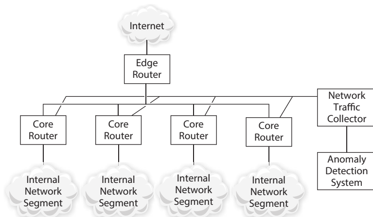
Figure 6-6 NTA systems collect data from several sources for analysis
