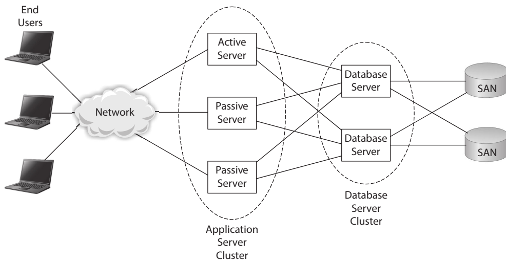
Figure 7-15 Application and database server clusters
