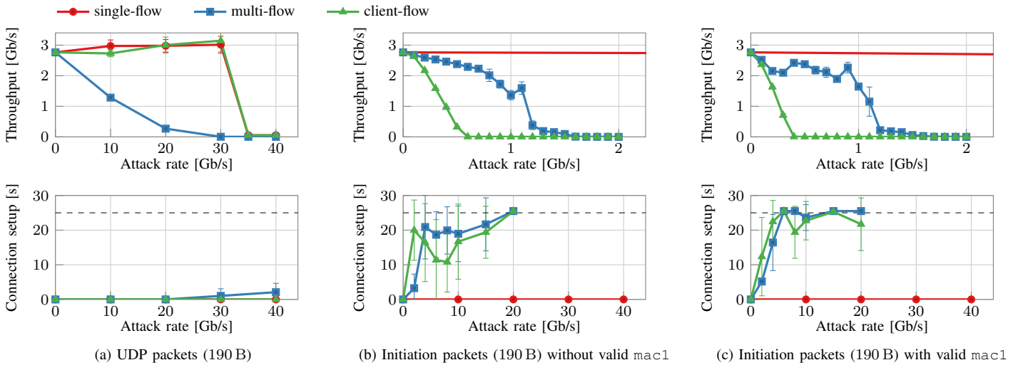
Fig. 4. Performance achieved by WireGuard under flooding attacks using different types of packets.
