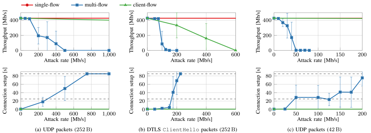
Fig. 11. Performance achieved by Cisco AnyConnect (SSL) under flooding attacks using different packets.
