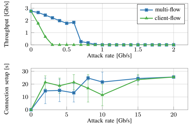
Fig. 13. Performance of WireGuard while flooding it with cookie response packets.
