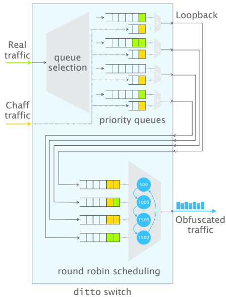
Fig. 4: ditto implements hierarchical queuing by sending each packet through the switch twice.
