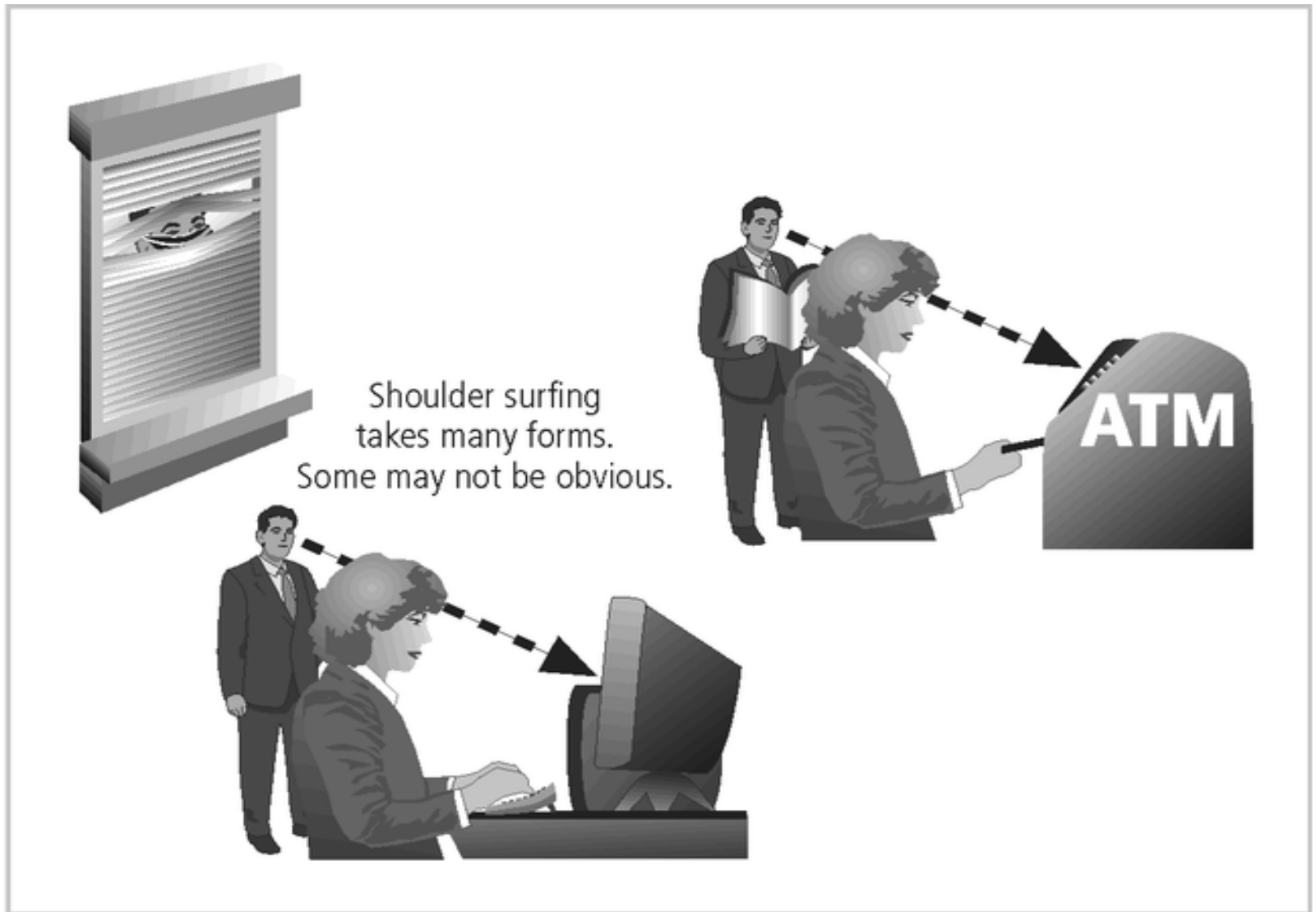
FIGURE 2-2 Shoulder Surfing
