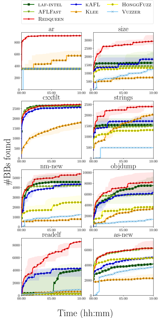
Fig. 2: The coverage (in basic blocks) produced by various tools over 5 runs at 10 h each on the binutils . Displayed are the median and the 60 % intervals.
