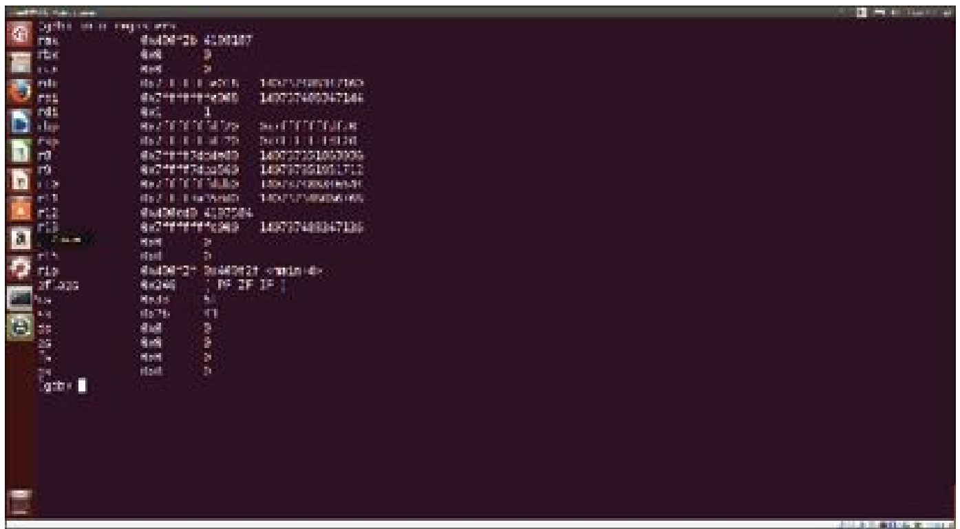
FIGURE 10.32 Examining registers in gdb.
