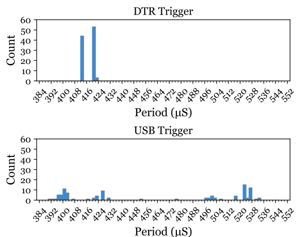
Figure 13: Histogram over 100 trigger period measured on i3-9100-MZ370 (2 GHz) with program running at priority 99 and SCHED_RR policy on core 1.
