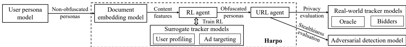
Fig. 5: Overview of HARPO’s evaluation process.
