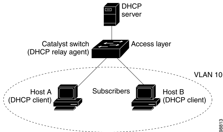
Figure 54-1 DHCP Relay Agent in a Metropolitan Ethernet Network
