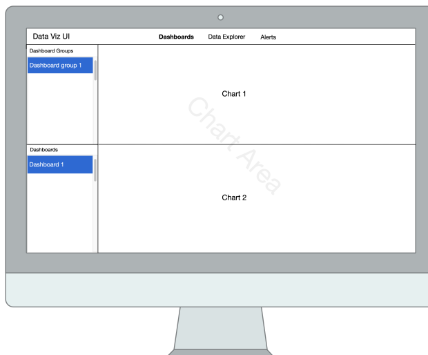
Figure 5.1. Dashboards Page
