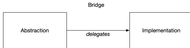
Fig 3.5 Bridge Pattern
