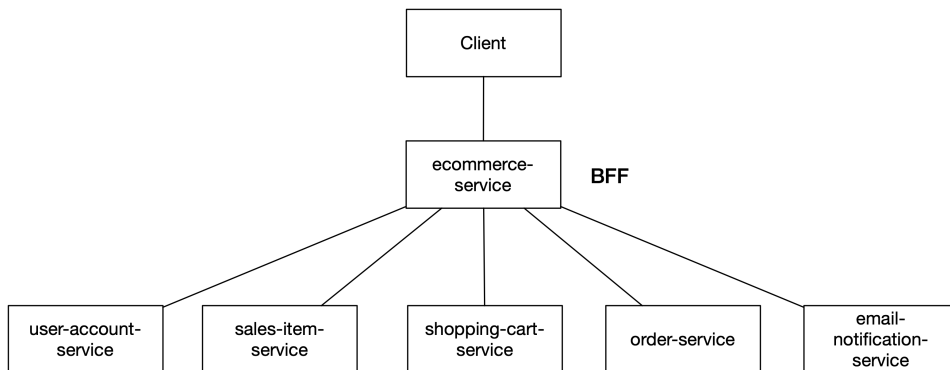
Fig 2.4 Service Aggregation in E-Commerce Software System
