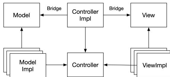
Fig 3.7 Dependencies in MVC pattern
