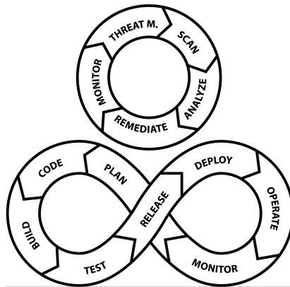
Fig 11.1 DevSecOps Diagram
