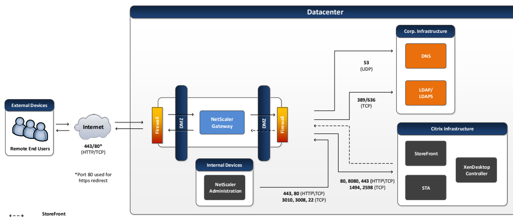
Figure 6: 2-Arm Topology
