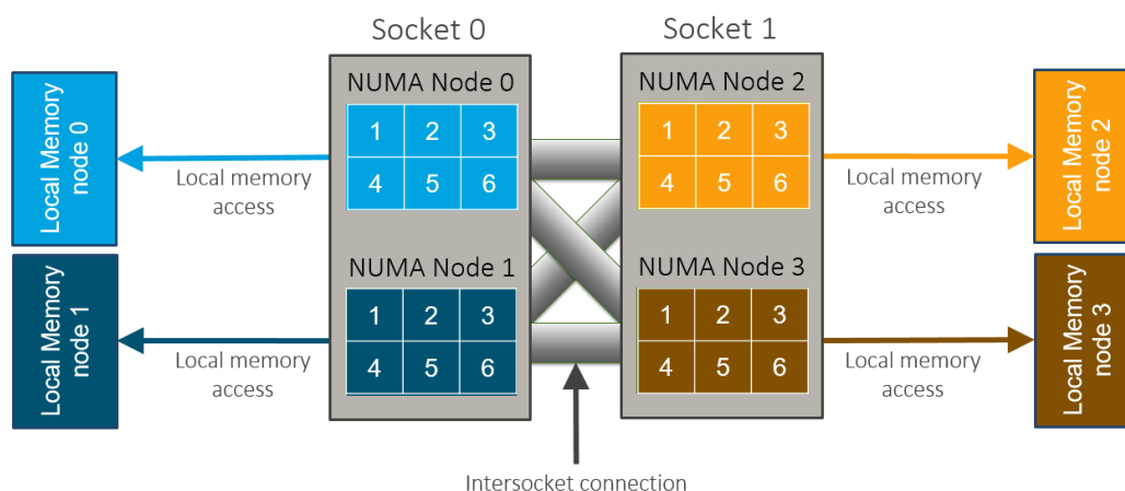
Figure 14: NUMA Architecture
