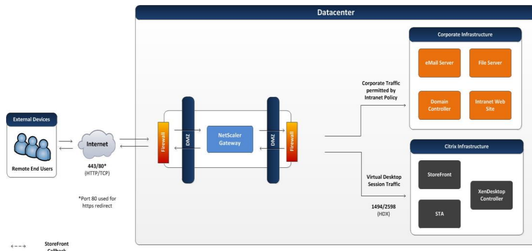
Figure 8: SSL VPN
