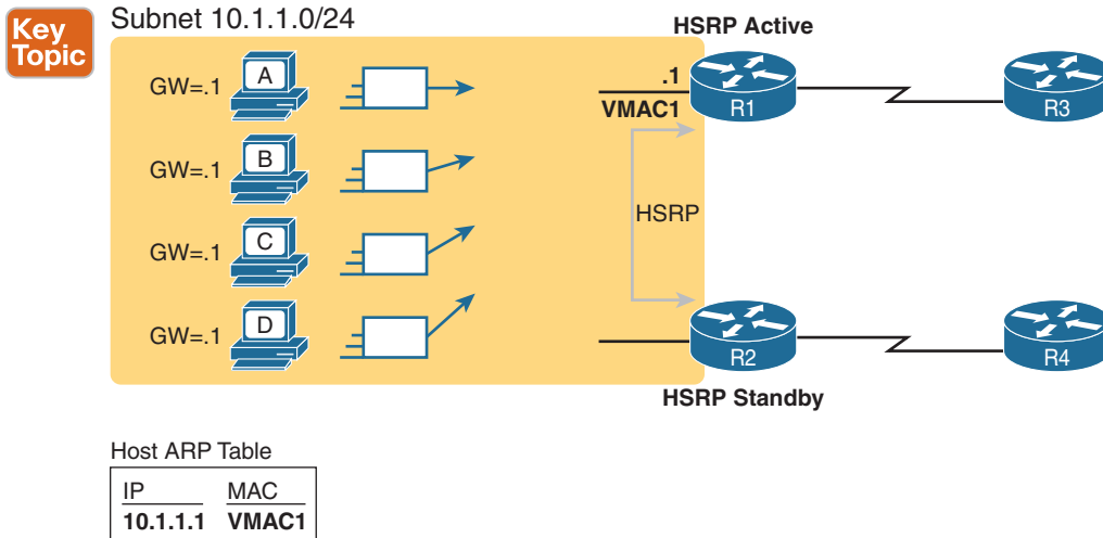
Figure 12-5 All Traffic Goes to .1 (R1, Which Is Active); R2 Is Standby
