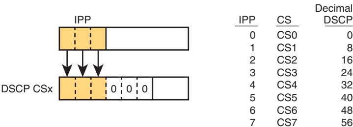
Figure 11-12 Class Selector
