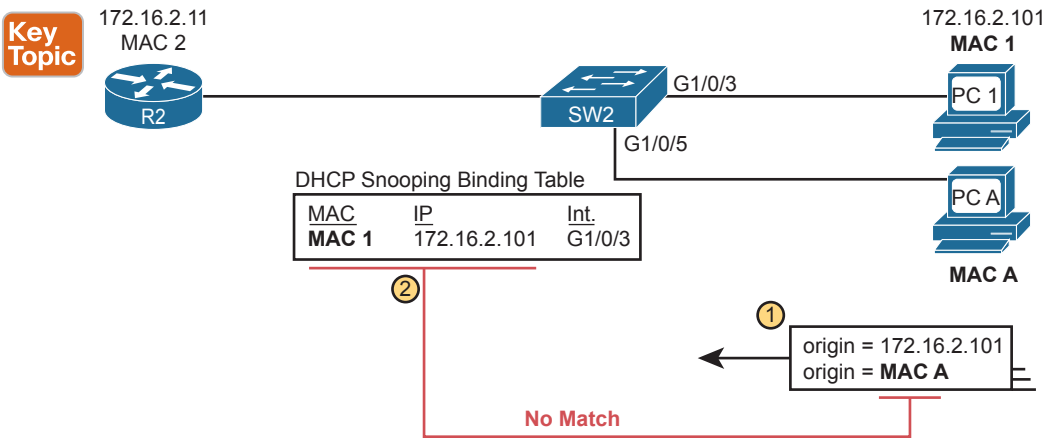
Figure 8-13 DAI Filtering ARP Based on DHCP Snooping Binding Table
