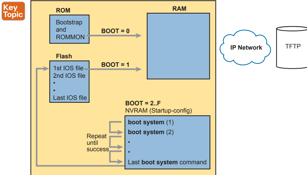
Figure F-4 Choices for Choosing the OS at Boot Time: Modern Cisco Router
