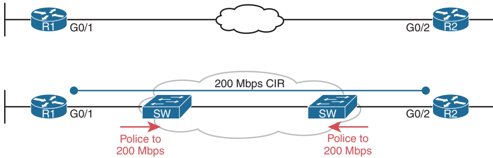
Figure 11-19 Ethernet WAN: Link Speed Versus CIR
