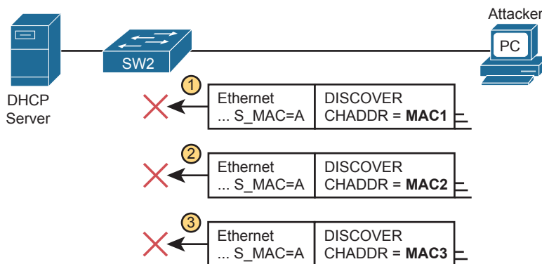
Figure 8-5 DHCP Snooping Checks chaddr and Ethernet Source MAC
