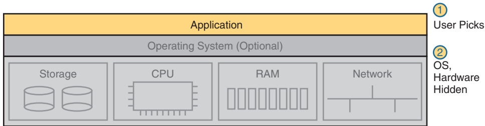
Figure 15-11 SaaS Concept
