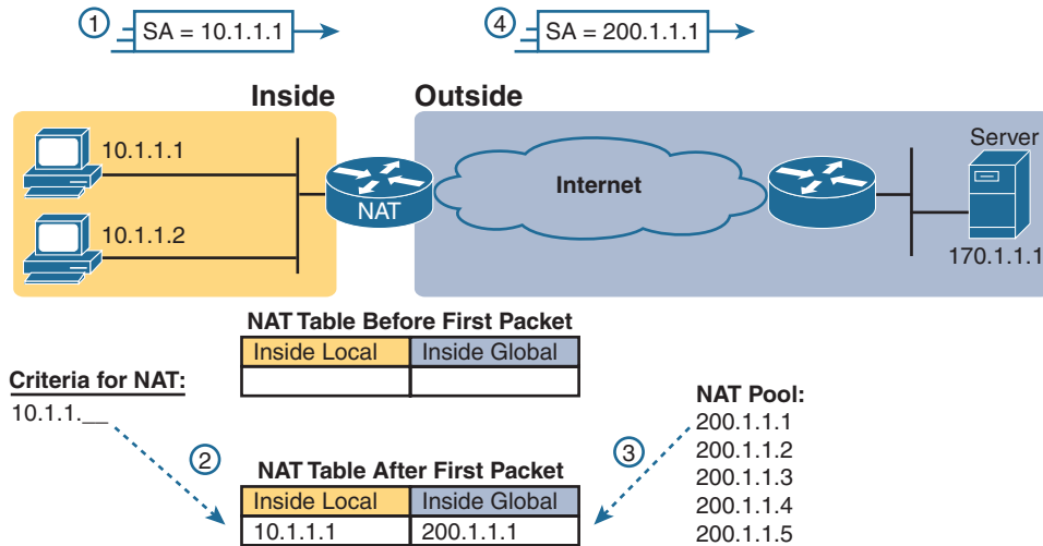
Figure 10-5 Dynamic NAT
