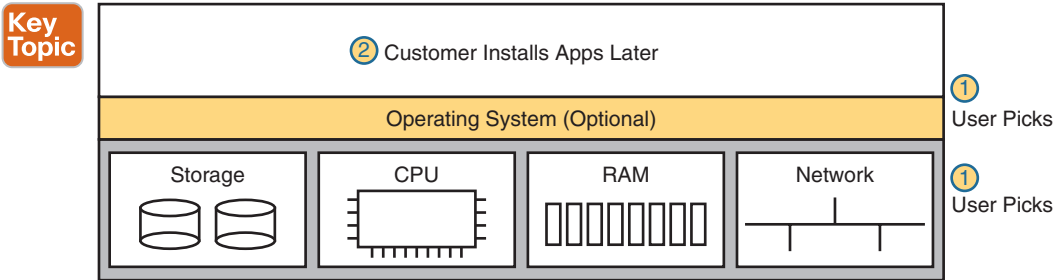
Figure 15-9 IaaS Concept
