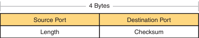
Figure 1-10 UDP Header
