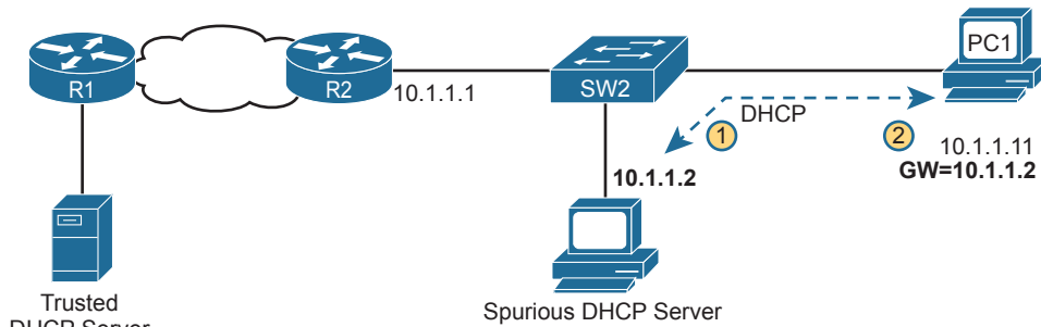
Figure 8-2 DHCP Attack Supplies Good IP Address but Wrong Default Gateway
