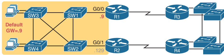
Figure 12-3 Removing All Single Points of Failure from the Network Design
