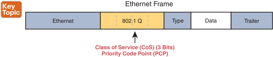
Figure 11-7 Class of Service Field in 802.1Q/p Header
