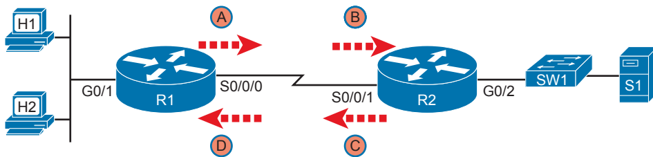
Figure D-6 Sample Network with IP ACLs in Four Locations
