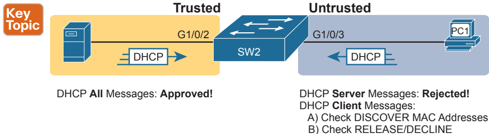
Figure 8-4 Summary of Rules for DHCP Snooping
