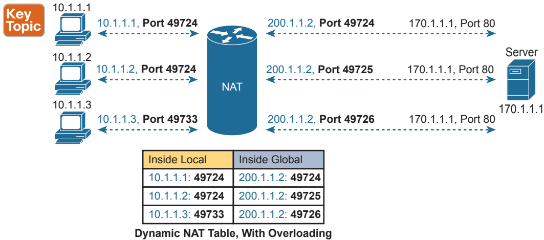
Figure 10-8 NAT Overload (PAT)
