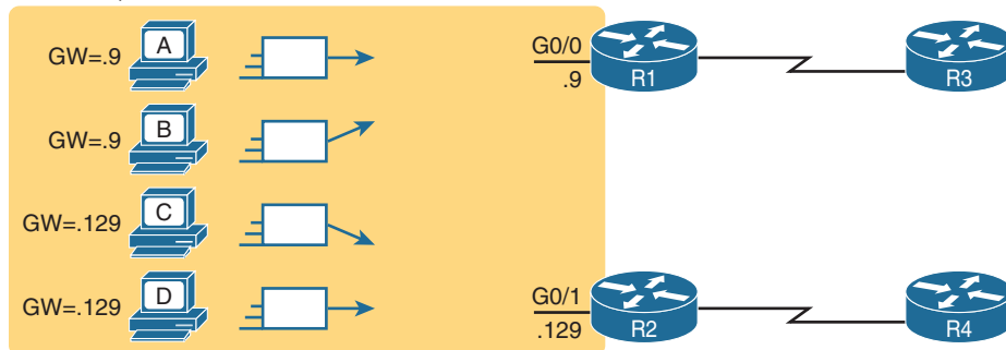
Figure 12-4 Balancing Traffic by Assigning Different Default Routers to Different Clients
