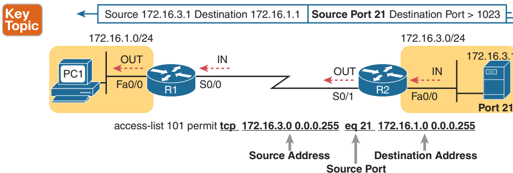
Figure 3-7 Filtering Packets Based on Source Port
