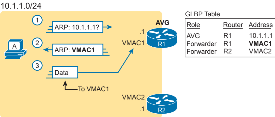
Figure D-10 GLBP Directs Host A by Sending Back ARP Reply with R1's VMAC1
