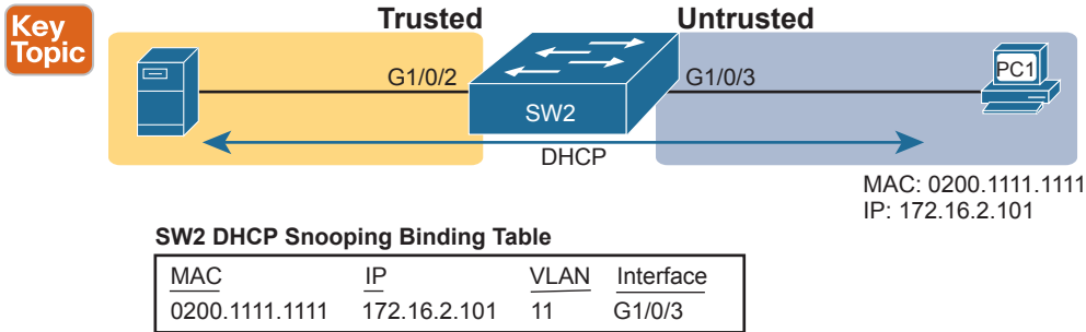
Figure 8-6 Legitimate DHCP Client with DHCP Binding Entry Built by DHCP Snooping
