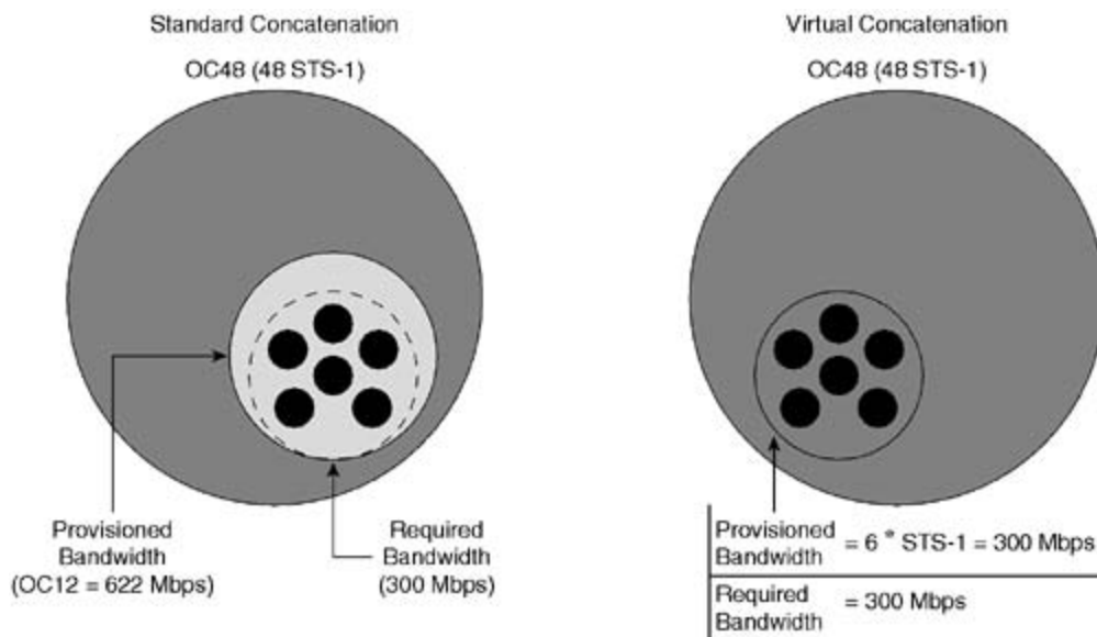
Figure 2-5. Virtual Concatenation
