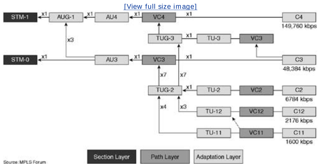
Figure A-6. SDH Low-Order Multiplexing Structure
