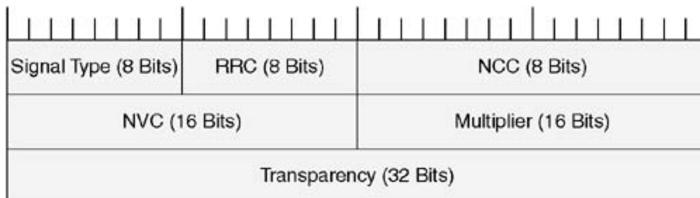
Figure 8-11. SONET/SDH Traffic Parameters
