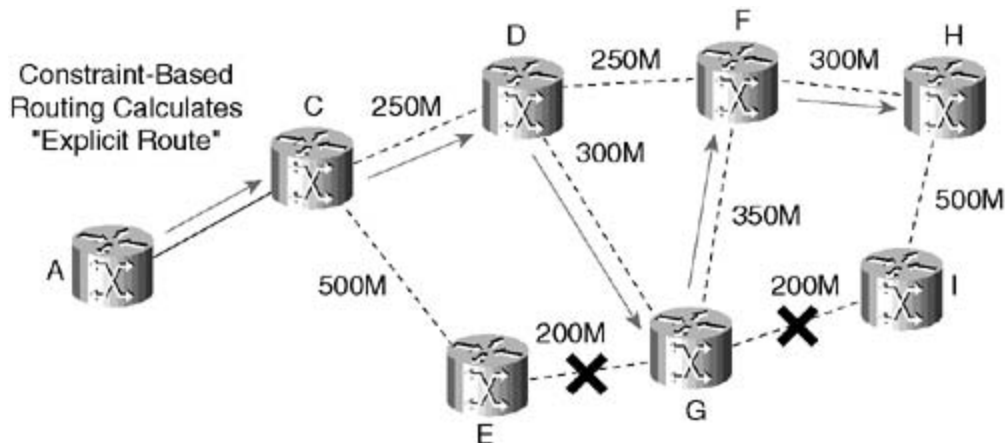
Figure 5-4b. Constraint-Based Routing
