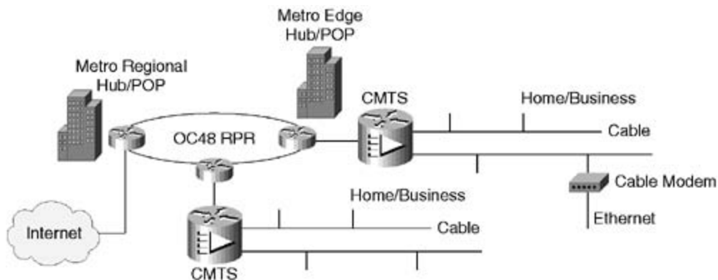
Figure 2-14. RPR Deployments
