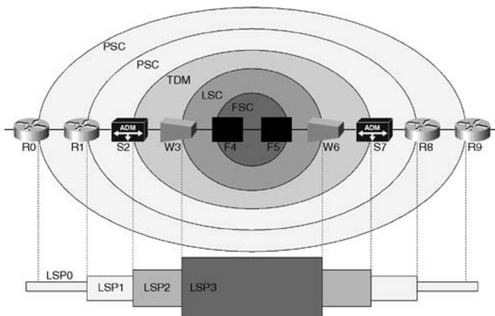
Figure 8-8. Nested LSPs
