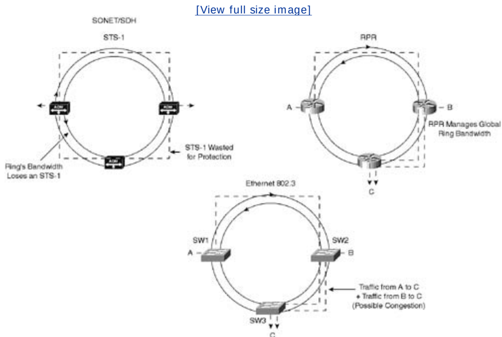
Figure 2-17. Ring Bandwidth
