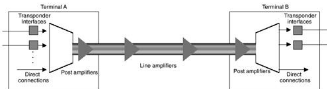
Figure 10-4. DWDM System
