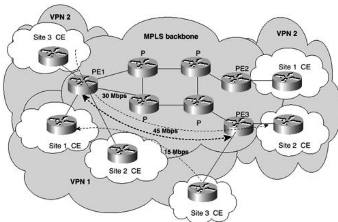
Figure 8-13. Guaranteed Bandwidth LSP: Pipe Model
