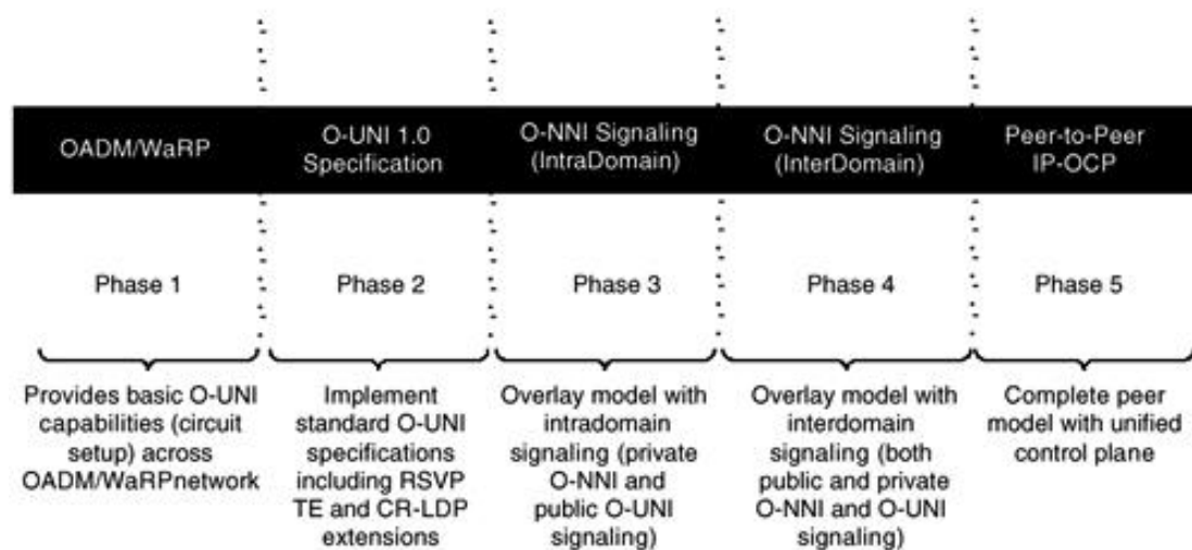
Figure 10-10. UCP Phased Deployment
