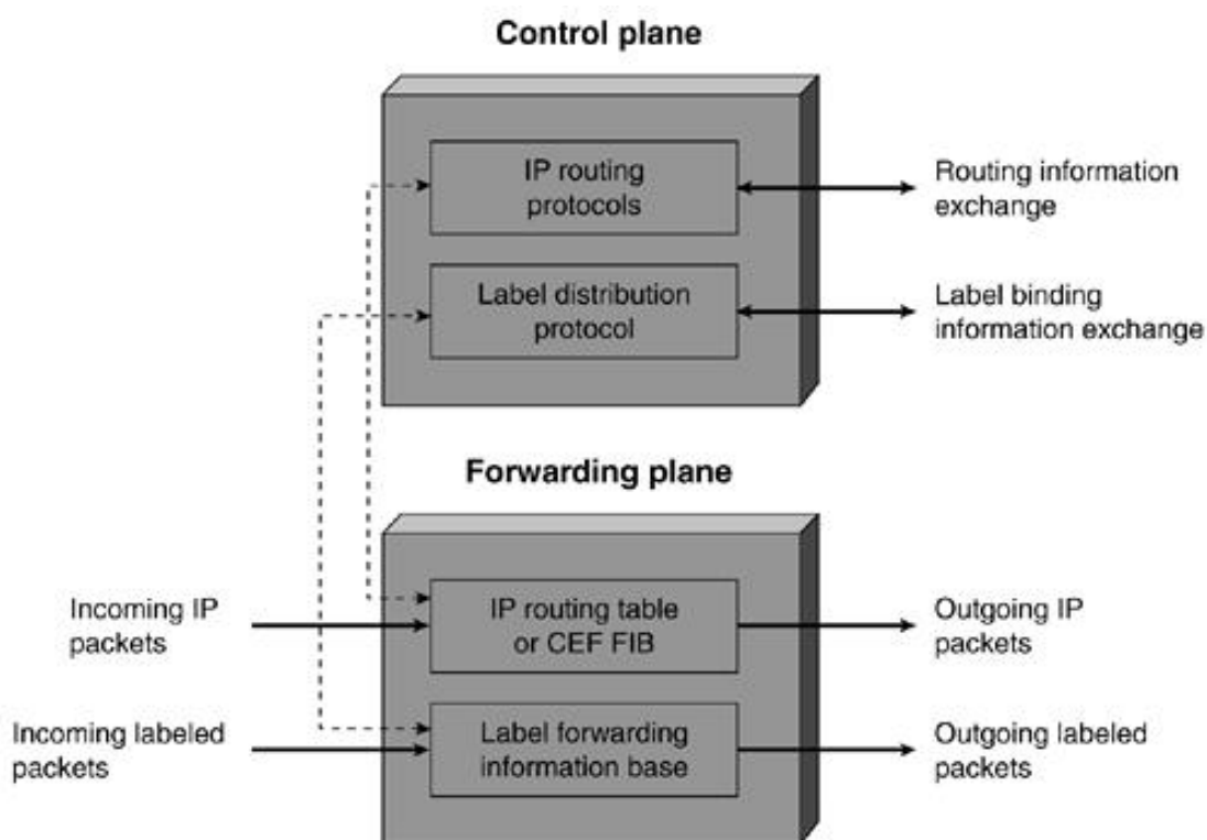
Figure 3-1. MPLS Node Architecture
