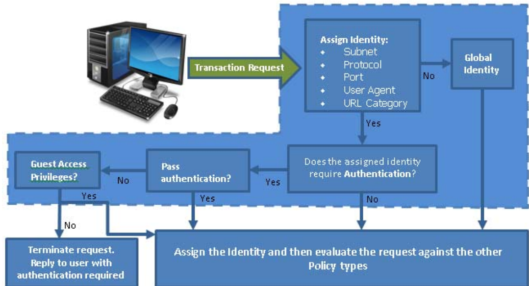
Figure 6-1 Transaction Request flow: Identification Profiles and Authentication - No Surrogates and IP-Based Surrogates
