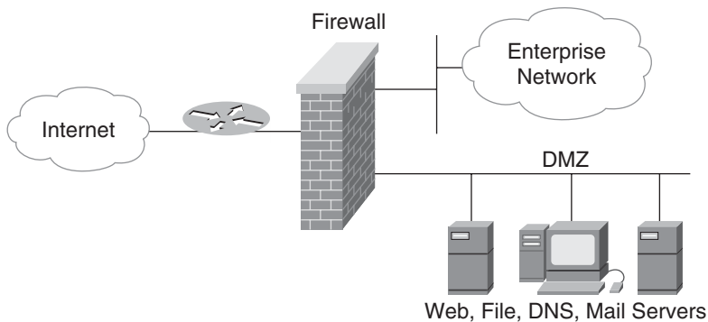
Figure 5-16 DMZ Topology
