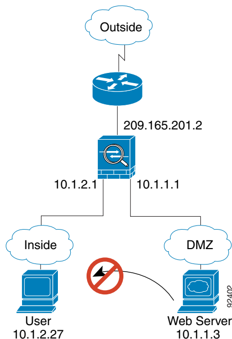
Figure 15-6 DMZ to Inside
