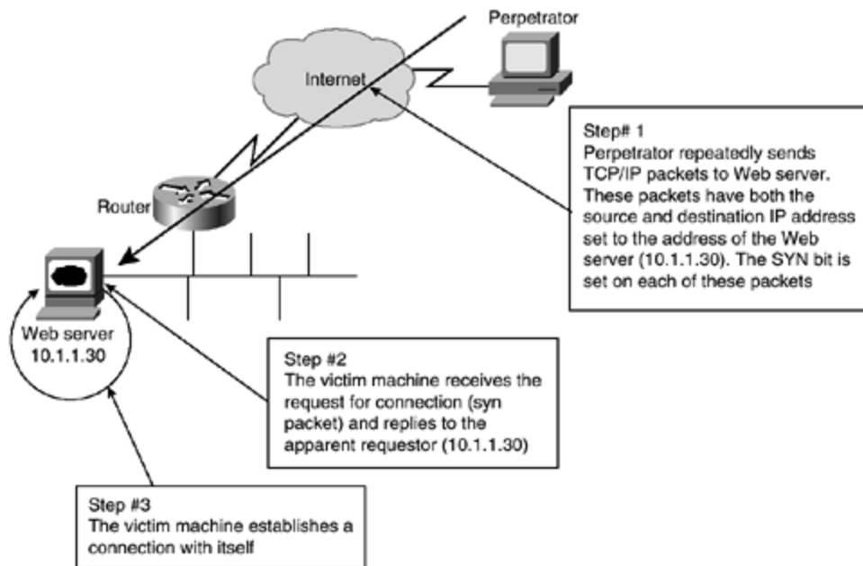
Figure 1-13. LAND.c Attack
