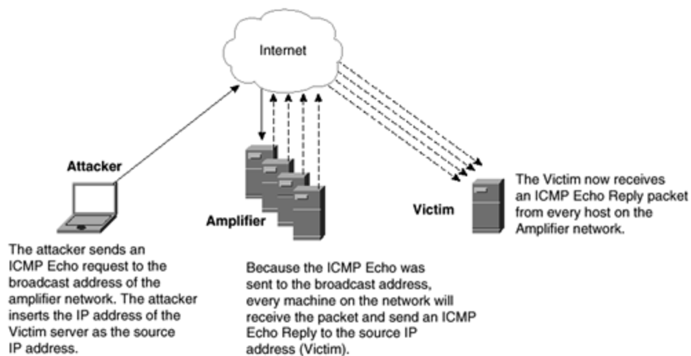
Figure 11-1. Smurf Attack
