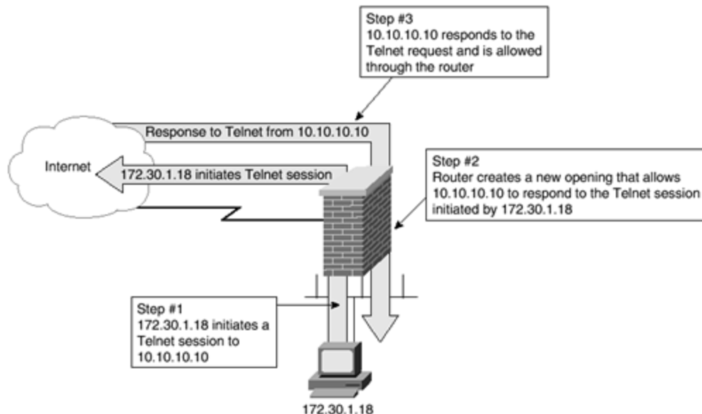
Figure 5-3. Reflective Access Lists Open the Router in Response to Connections Initiated from Inside the Network
