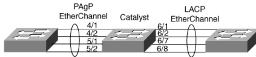
Figure 4-1. Network Diagram for the EtherChannel Example
