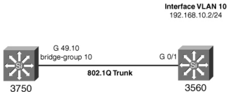
Figure 5-4. Network Topology for Virtual Interface Configuration Example
