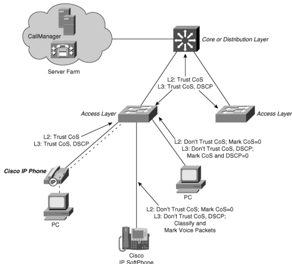
Figure 14-1. QoS Trust Considerations in a Switched Network
